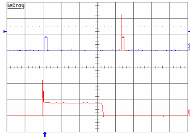
Figure 14. Load current (top trace, 5A/div., 50ms/div.) into a 10\text{m} short circuit during restart, at V_{in} = 48\text{V} . Bottom trace (5A/div., 2ms/div.) is an expansion of the on-time portion of the top trace
