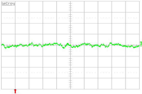
Figure 12. Input reflected-ripple current, i_s (10mA/div.), measured through 10\mu\text{H} at the source at full rated load current and V_{in} = 48\text{V} . Refer to Figure 11 for test setup. Time scale: 1\mu\text{s}/\text{div} .
