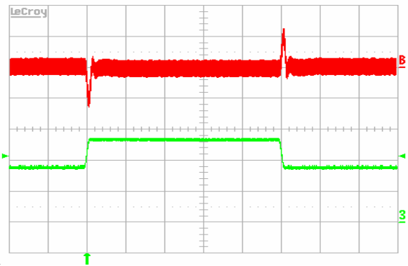
Figure 8. Output voltage response to load current step- (3.5A–5.25A–3.5A) at V_{in}=48V . Top trace: output voltage (100mV/div.) Bottom trace: load current (2A/div.). Current slew rate: 0.1A/ \mu s. C_o=1\mu F ceramic + 10 \mu F tantalum. Time scale: 0.2ms/div.
