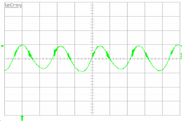
Figure 13. Input reflected ripple-current, i_C (50mA/div.), measured at input terminals at full rated load current and V_{in} = 48\text{V} . Refer to Figure 11 for test setup. Time scale: 1\mu\text{s}/\text{div} .
