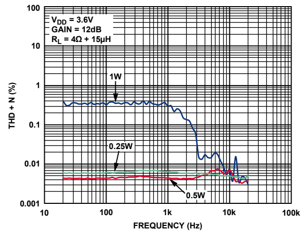
Figure 14. THD + N vs. Frequency, V_{DD} = 3.6\text{ V} , R_L = 4\ \Omega , Gain = 12 dB
