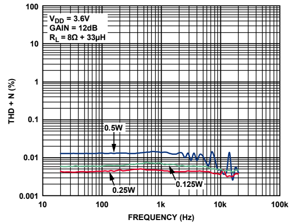
Figure 13. THD + N vs. Frequency, V_{DD} = 3.6\text{ V} , R_L = 8\ \Omega , Gain = 12 dB
