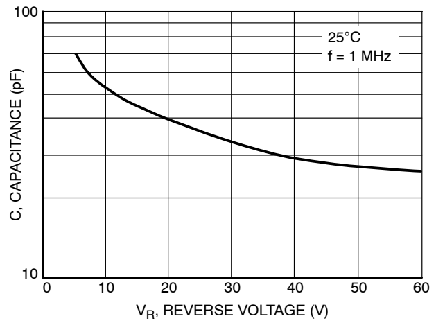
Figure 4. Typical Capacitance
