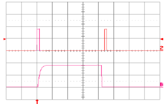
Fig. 2.5V.16: Load current (top trace, 20 A/div., 50 ms/div.) into a 10 m \Omega short circuit during restart, at V_{in} = 48 \text{ V} . Bottom trace (20 A/div., 2 ms/div.) is an expansion of the on-time portion of the top trace.
