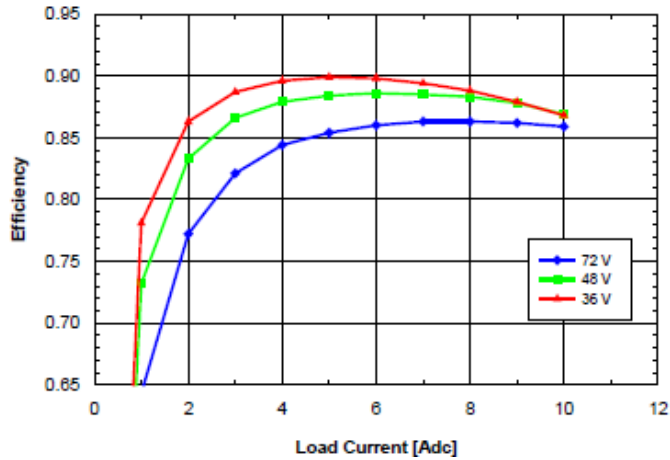
Fig. 5.0V.5: Efficiency vs. load current and input voltage for SQ48T/S10050 converter mounted vertically with air flowing from pin 3 to pin 1 at a rate of 300 LFM (1.5 m/s) and T_a = 25^\circ\text{C} .
