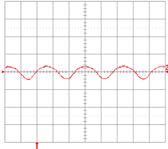
Fig. 1.5V.15: Input reflected ripple current, i_c (100 mA/div.), measured at input terminals at full rated load current and V_{in} = 48 V. Refer to Fig. 1.5V.14 for test setup. Time scale: 1 \mu s/div.
