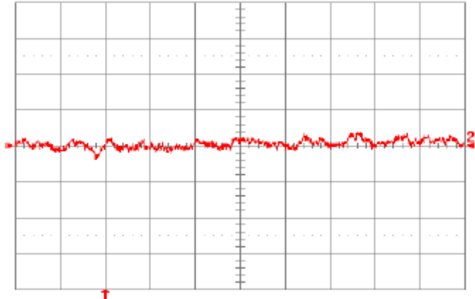
Fig. 12V.16: Input reflected ripple current, i_s (100 mA/div.), measured at input terminals at full rated full rated load current and V_{in} = 48V . Refer to Fig. 12V.14 for test setup. Time scale: 1 \mu s /div.
