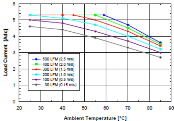
Fig. 8.OV.2: Available load current vs. ambient air temperature and airflow rates for SQ48T05080 converter with D height pins mounted horizontally with V_{in} = 48\text{ V} , air flowing from pin 3 to pin 1, and maximum FET temperature \leq 120^\circ\text{C} .
