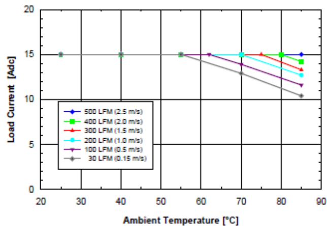
Fig. 2.5V.1: Available load current vs. ambient air temperature and airflow rates for SQ48T15025 converter with D height pins mounted vertically with V in = 48 V, air flowing from pin 3 to pin 1, and maximum FET temperature ≤ 120 °C.
