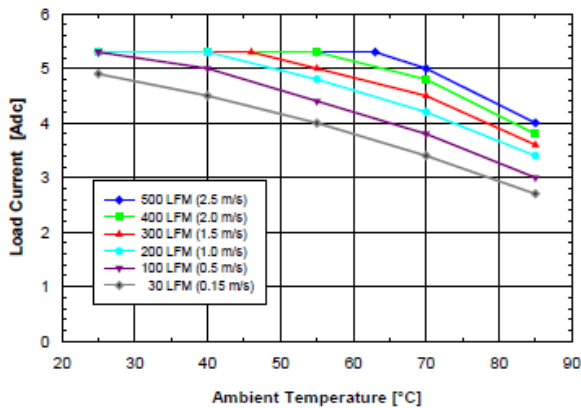
Fig. 8.OV.1: Available load current vs. ambient air temperature and airflow rates for SQ48T05080 converter with D height pins mounted vertically with V_{in} = 48\text{ V} , air flowing from pin 3 to pin 1, and maximum FET temperature \leq 120^\circ\text{C} .
