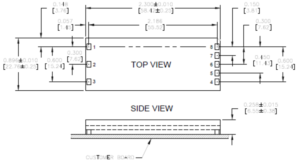
SQ48S Pinout (Surface Mount)
