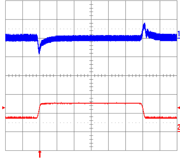
Fig. 1.5V.11: Output voltage response to load current step-change (3.75 A – 7.5 A – 3.75 A) at V_{in} = 48 V. Top trace: output voltage (100 mV/div.). Bottom trace: load current (5 A/div.). Current slew rate: 0.1 A/ \mu s. C_o = 1 \mu F ceramic. Time scale: 0.2 ms/div.
