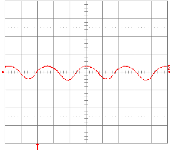
Fig. 1.8V.15: Input reflected ripple current, i_c (100 mA/div.), measured at input terminals at full rated load current and V_{in} = 48 V. Refer to Fig. 1.8V.14 for test setup. Time scale: 1 \mu s/div.
