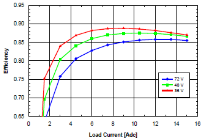
Fig. 2.0V.5: Efficiency vs. load current and input voltage for SQ48T/S15020 converter mounted vertically with air flowing from pin 3 to pin 1 at a rate of 300 LFM (1.5 m/s) and T_a = 25 °C.
