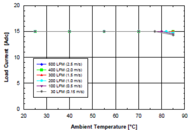
Fig. 1.2V.4: Available load current vs. ambient air temperature and airflow rates for SQ48S15012 converter mounted horizontally with V_{in} = 48 V, air flowing from pin 3 to pin 1, and maximum FET temperature \leq 120 °C.
