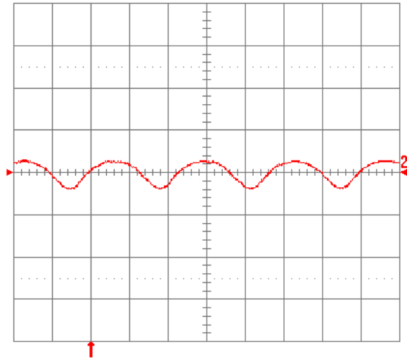
Fig. 1.2V.15: Input reflected ripple current, i_c (100 mA/div.), measured at input terminals at full rated load current and V_{in} = 48 V. Refer to Fig. 1.2V.14 for test setup. Time scale: 1 \mu s/div.
