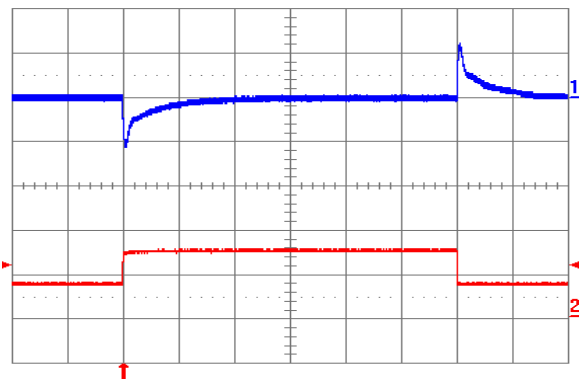
Fig. 1.5V.12: Output voltage response to load current step-change (3.75 A – 7.5 A – 3.75 A) at V in = 24V. Top trace: output voltage (100 mV/div.). Bottom trace: load current (5 A/div.). Current slew rate: 5 A/µs. C o = 450 µF tantalum + 1 µF ceramic. Time scale: 0.2 ms/div.
