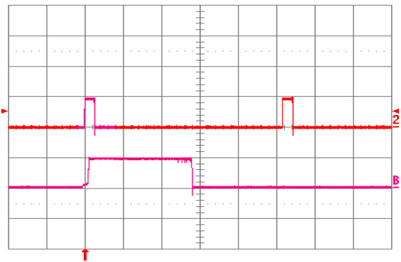
Fig. 1.5V.18: Load current (top trace, 20 A/div., 20 ms/div.) into a 10 \text{ m}\Omega short circuit during restart, at V_{in} = 24 \text{ V} . Bottom trace (20 A/div., 2 ms/div.) is an expansion of the on-time portion of the top trace.
