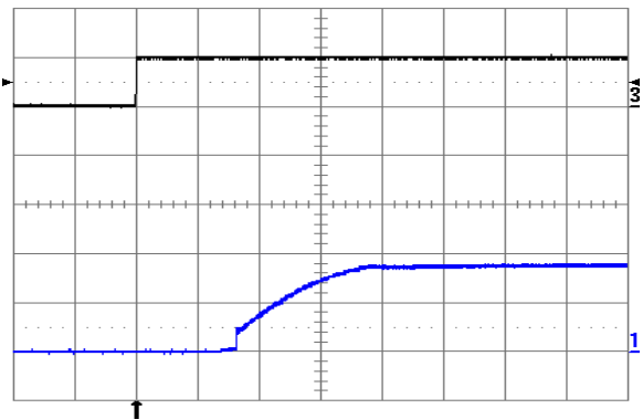
Fig. 1.8V.10: Turn-on transient at full rated load current (resistive) plus 10,000µF at V in = 24V, triggered via ON/OFF pin. Top trace: ON/OFF signal (5 V/div.). Bottom trace: output voltage (1 V/div.). Time scale: 1 ms/div.
