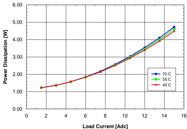
Fig. 1.5V.8: Power dissipation vs. load current and ambient temperature for SQ24T/S15015 converter mounted vertically with V in = 24V and air flowing from pin 3 to pin 1 at a rate of 200 LFM (1.0 m/s).
