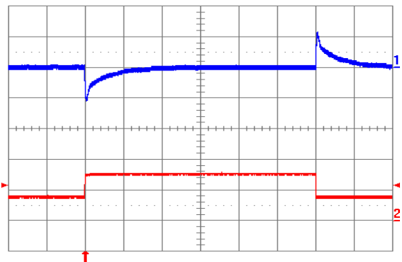
Fig. 2.5V.12: Output voltage response to load current step-change (3.75 A – 7.5 A – 3.75 A) at V in = 24V. Top trace: output voltage (100 mV/div.). Bottom trace: load current (5 A/div.). Current slew rate: 5 A/µs. C o = 450 µF tantalum + 1 µF ceramic. Time scale: 0.2 ms/div.
