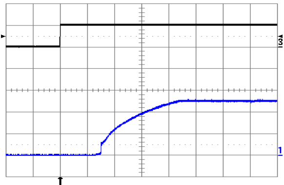
Fig. 2.5V.10: Turn-on transient at full rated load current (resistive) plus 10,000 µF at V in = 24V, triggered via ON/OFF pin. Top trace: ON/OFF signal (5 V/div.). Bottom trace: output voltage (1 V/div.). Time scale: 1 ms/div.
