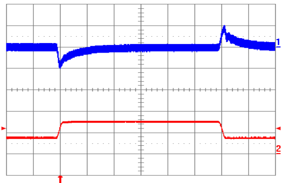
Fig. 1.5V.11: Output voltage response to load current step-change (3.75 A – 7.5 A – 3.75 A) at V in = 24V. Top trace: output voltage (100 mV/div.). Bottom trace: load current (5 A/div.). Current slew rate: 0.1 A/µs. C o = 1 µF ceramic. Time scale: 0.2 ms/div.
