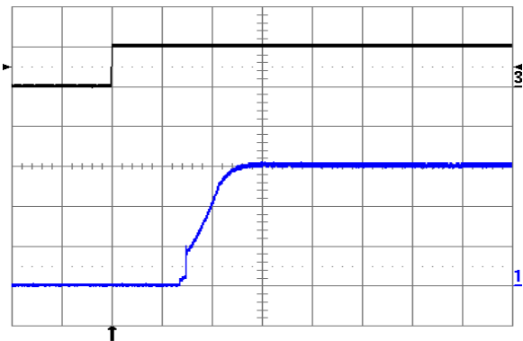
Fig. 1.5V.9: Turn-on transient at full rated load current (resistive) with no output capacitor at V in = 24V, triggered via ON/OFF pin. Top trace: ON/OFF signal (5 V/div.). Bottom trace: output voltage (0.5 V/div.). Time scale: 1 ms/div.
