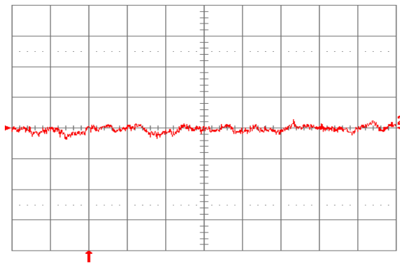
Fig. 3.3V.16: Input reflected ripple current, i_s (10 mA/div.), measured through 10 \mu\text{H} at the source at full rated load current and V_{in} = 24\text{V} . Refer to Fig. 3.3V.14 for test setup. Time scale: 1 \mu\text{s}/\text{div} .
