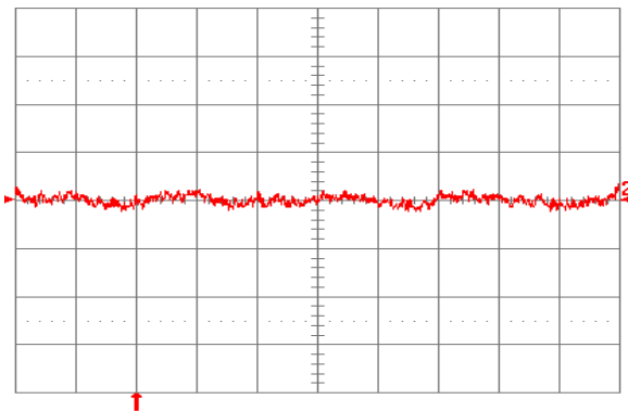
Fig. 6.0V.16: Input reflected ripple current, i_s (10 mA/div.), measured through 10 \mu\text{H} at the source at full rated load current and V_{in} = 24\text{V} . Refer to Fig. 6.0V.14 for test setup. Time scale: 1 \mu\text{s}/\text{div} .
