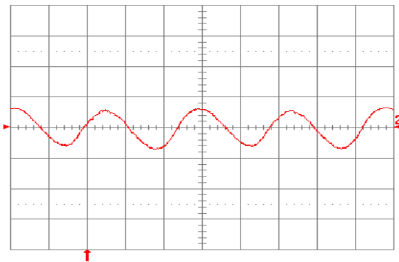
Fig. 6.0V.15: Input reflected ripple current, i_c (100 mA/div.), measured at input terminals at full rated load current and V_{in} = 24\text{V} . Refer to Fig. 6.0V.14 for test setup. Time scale: 1 \mu\text{s}/\text{div} .
