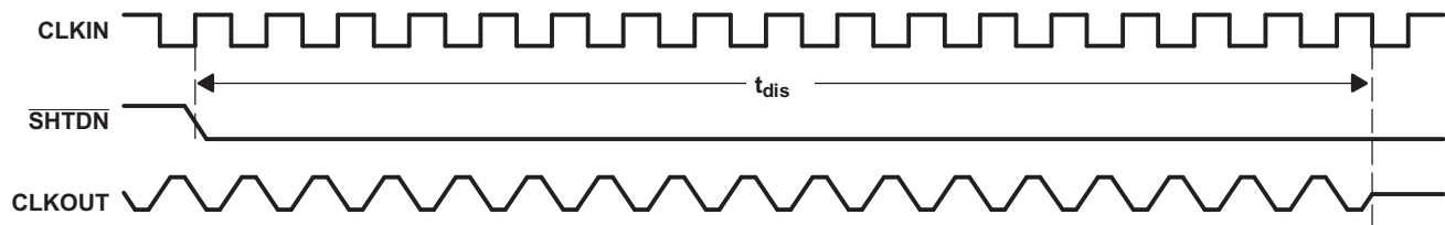
Figure 4. Disable Time Waveforms
