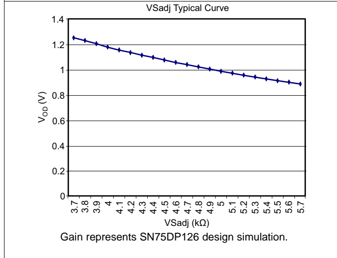
Figure 17. V_{OD} vs. V_{Sadj}
