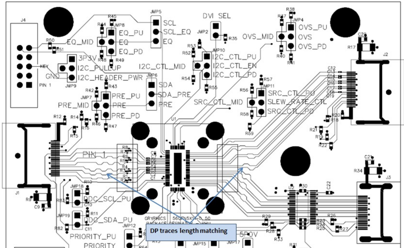
Figure 40. SN75DP126 Layout
