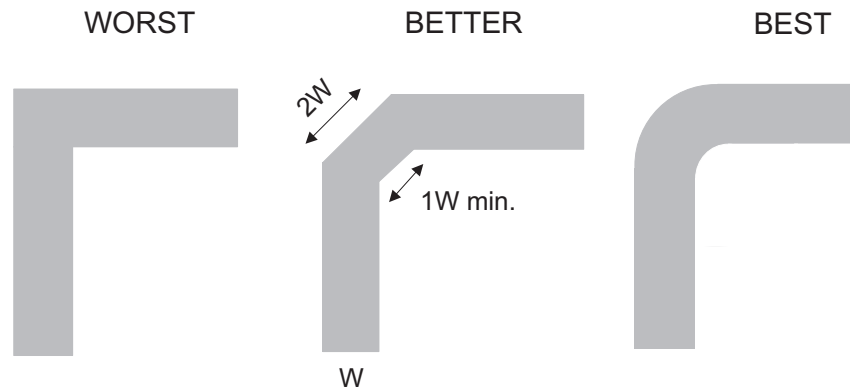
Figure 15. Trace Example
