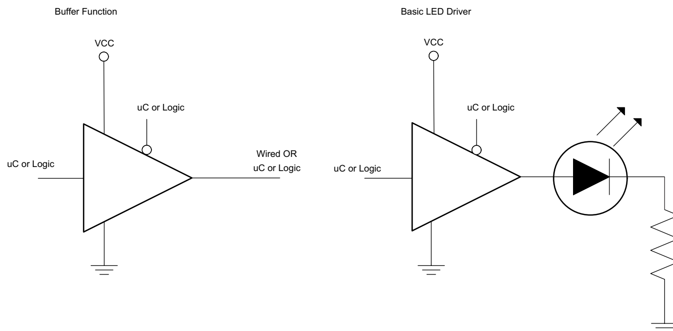
Figure 9-1. Application Schematic
