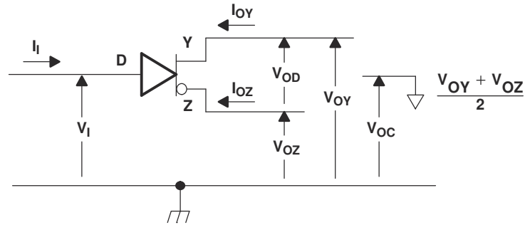
Figure 7-1. Driver Voltage and Current Definitions
