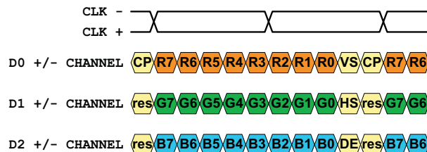
Figure 37. Data and Clock Input in 3-ChM (LS0 = low; LS1 = high)
