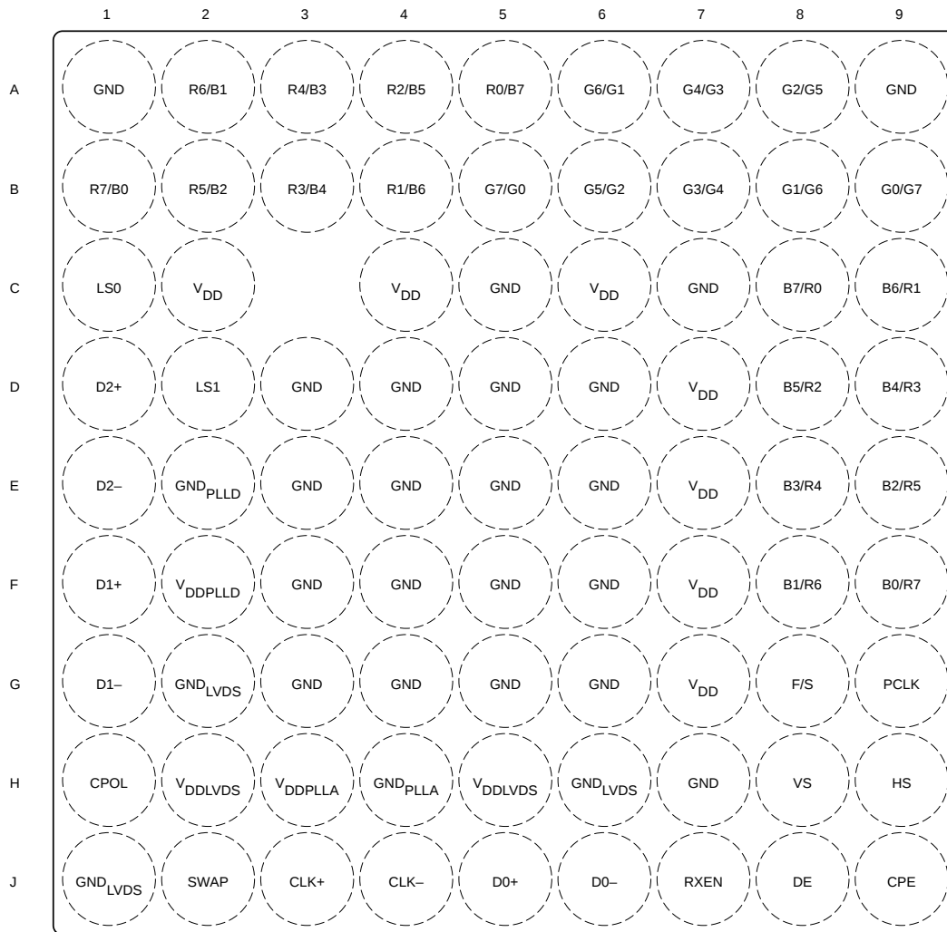
ZQE Package 80-Pin BGA MICROSTAR JUNIOR Top View
