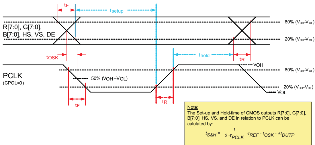
Figure 23. Output Rise and Fall, Setup and Hold Time
