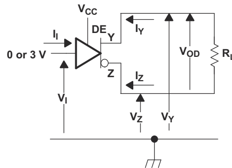
Figure 8-1. Driver Enable Time From DE to V_{OD}
