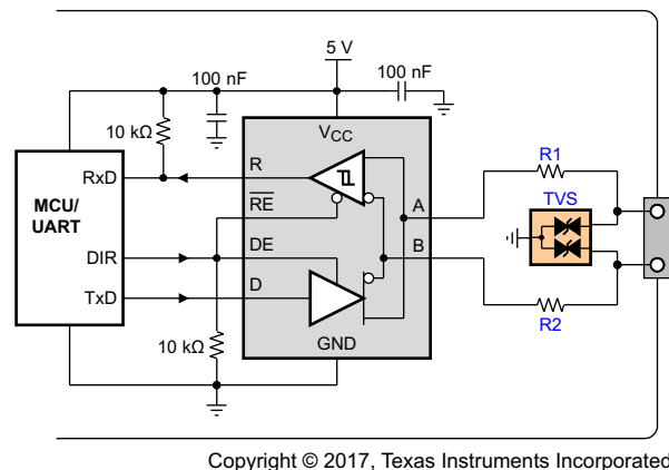
Figure 25. Transient Protection Against ESD, EFT, and Surge Transients
