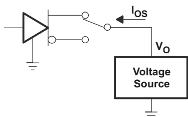
Figure 14. Driver Short-Circuit
