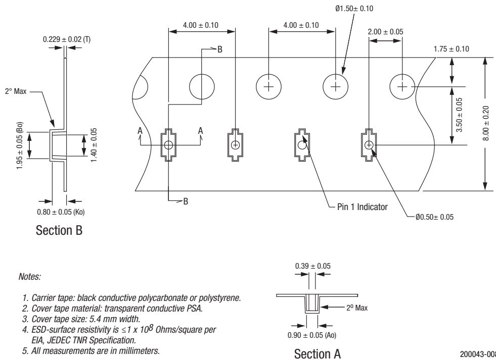
Figure 8. SC-79 Tape and Reel Dimensions
