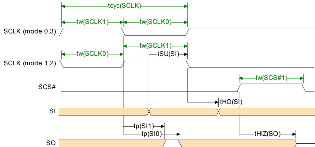
Figure 32: Slave SPI Data Timing
