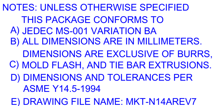
Figure 4. 14-Lead Plastic Dual-In-Line Package (PDIP), JEDEC MS-001, 0.300" Wide
