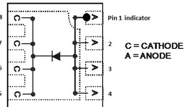
Top View Schematic and Pin Configuration
