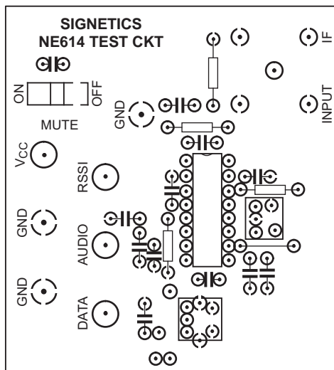
Fig 15. Components (viewed from the top)
