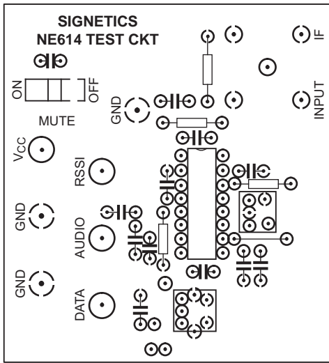
Fig 15. Components (viewed from the top)
