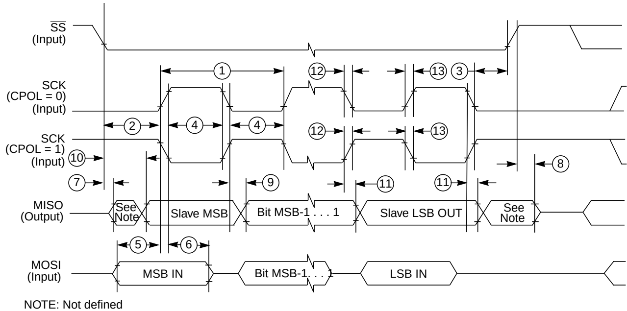
Figure A-9. SPI Slave Timing ( CPHA = 0 )
