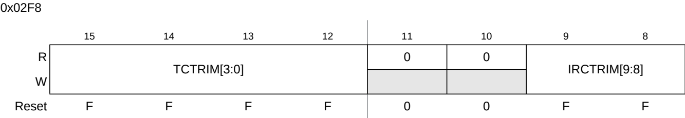
Figure 7-24. S12CPMU IRC1M Trim High Register (CPMUIRCTRIMH)
