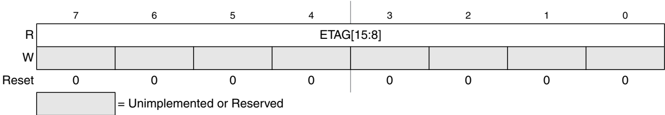
Figure 27-18. EEE Tag Counter High Register (ETAGHI)
