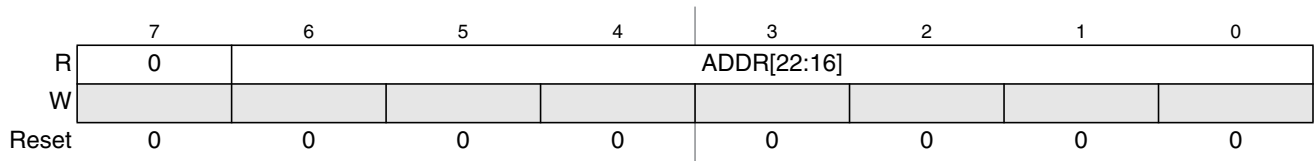
Figure 4-4. MPU Address Status Register 0 (MPUASTAT0)
