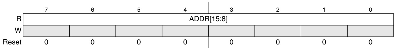
Figure 4-5. MPU Address Status Register 1 (MPUASTAT1)
