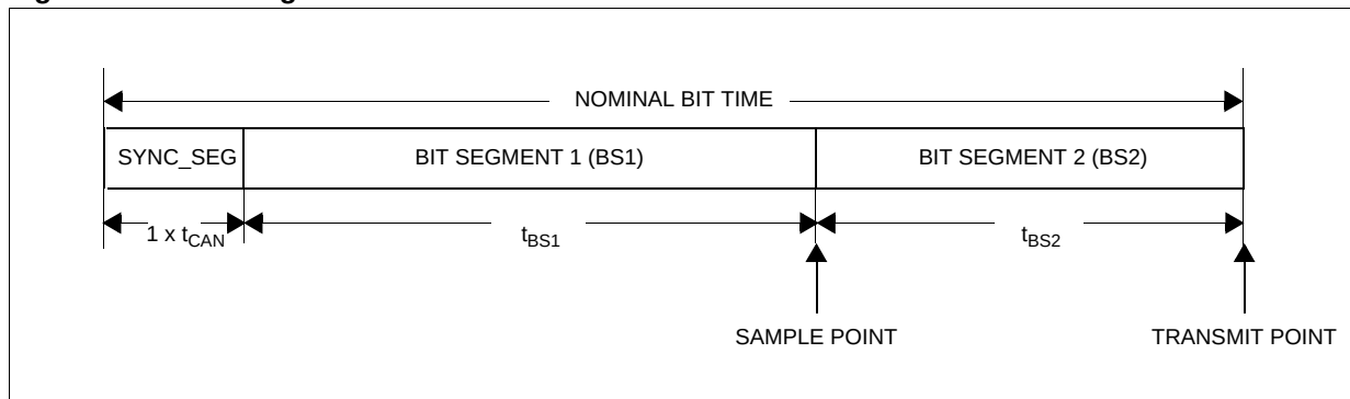
Figure 72. Bit Timing
