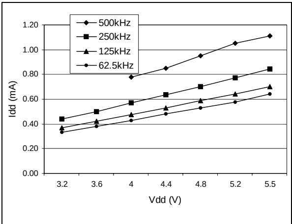
Figure 88. Typical I_{DD} in SLOW mode
