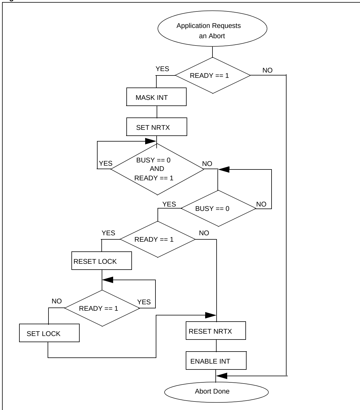
Figure 75. Work-around Flowchart
