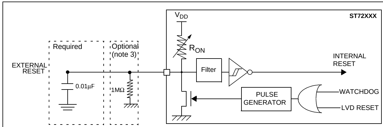
Figure 104. RESET pin protection when LVD is disabled. 1)
