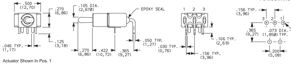
7101MD9A4BE Horizontal Actuation SPDT
