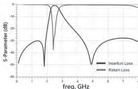
RFBPF2009A12T
