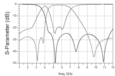
RFDIP1608060LST
