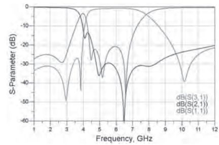
RFDIP160806ALM6T30
