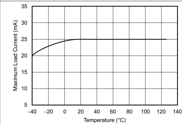
Figure 7-4. Maximum Load Current vs Temperature
