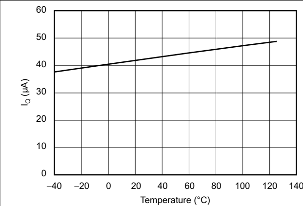
Figure 7-6. Quiescent Current vs Temperature
