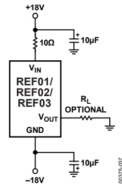
Figure 37. Burn-In Circuit
