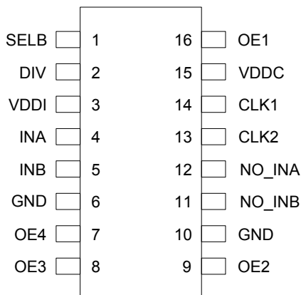
16-pin TSSOP
