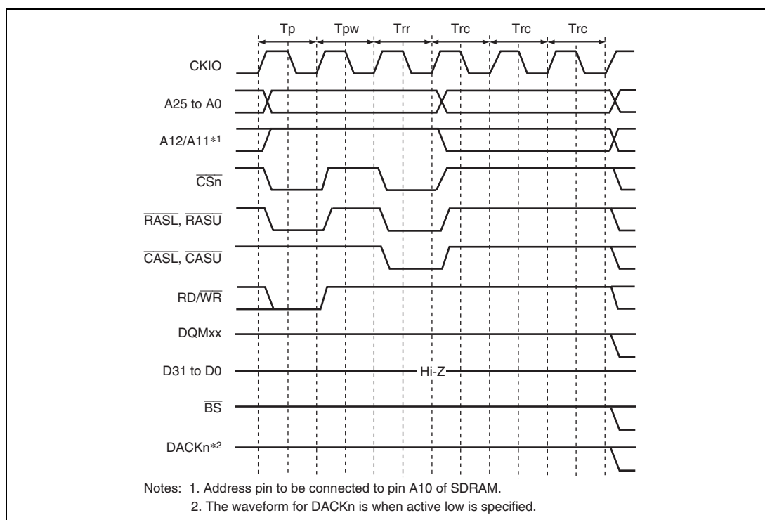
Figure 9.28 Auto-Refresh Timing
