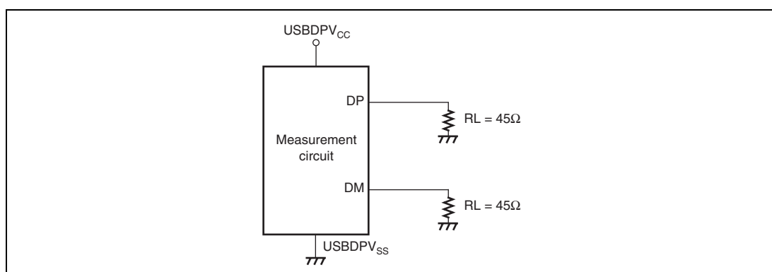
Figure 31.77 Measurement Circuit (High-Speed)
