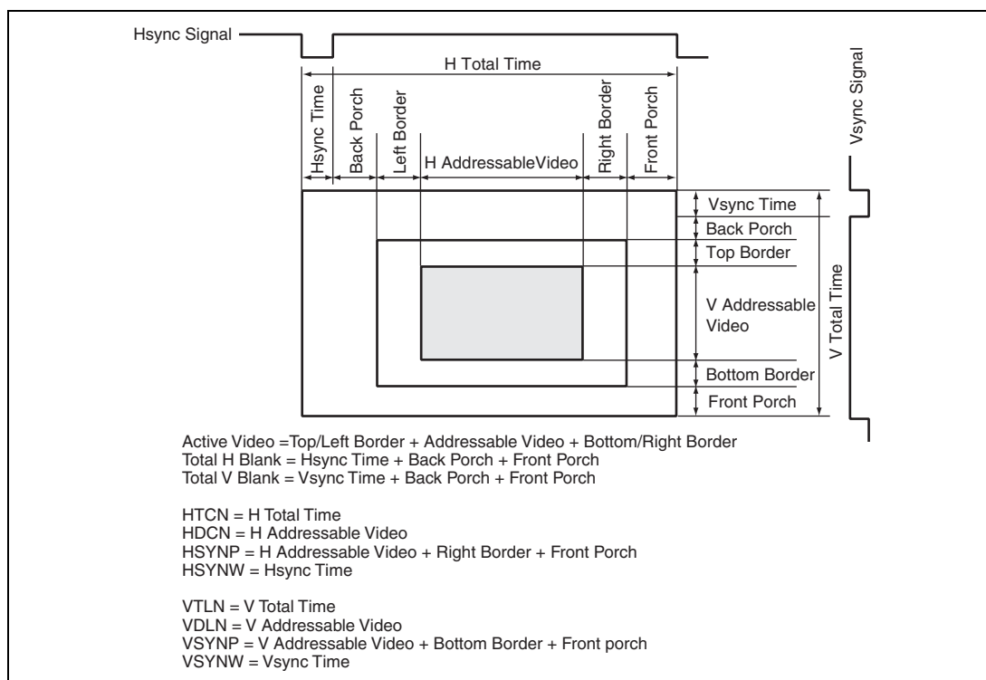
Figure 24.2 Valid Display and the Retrace Period
