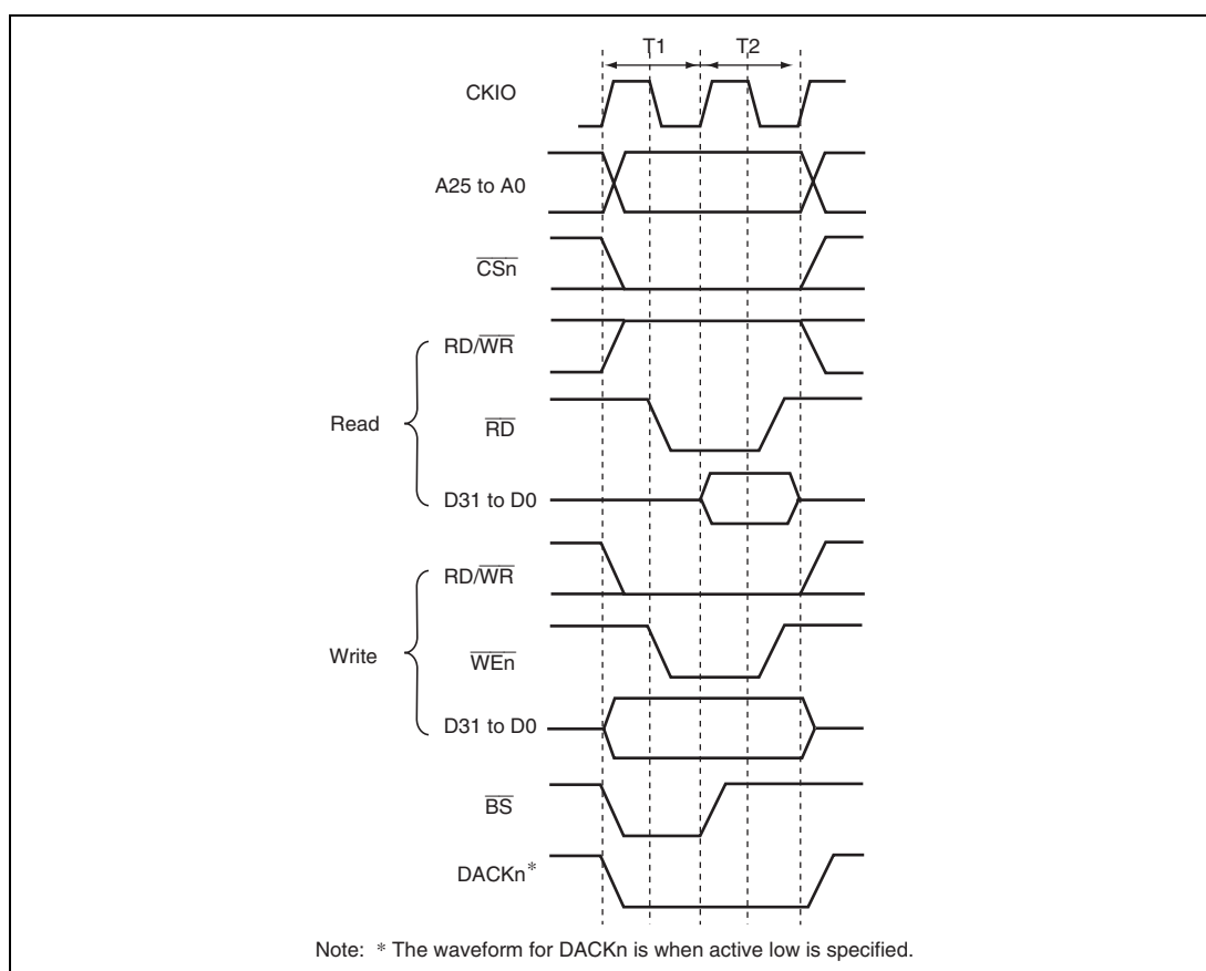
Figure 9.2 Normal Space Basic Access Timing (Access Wait 0)
