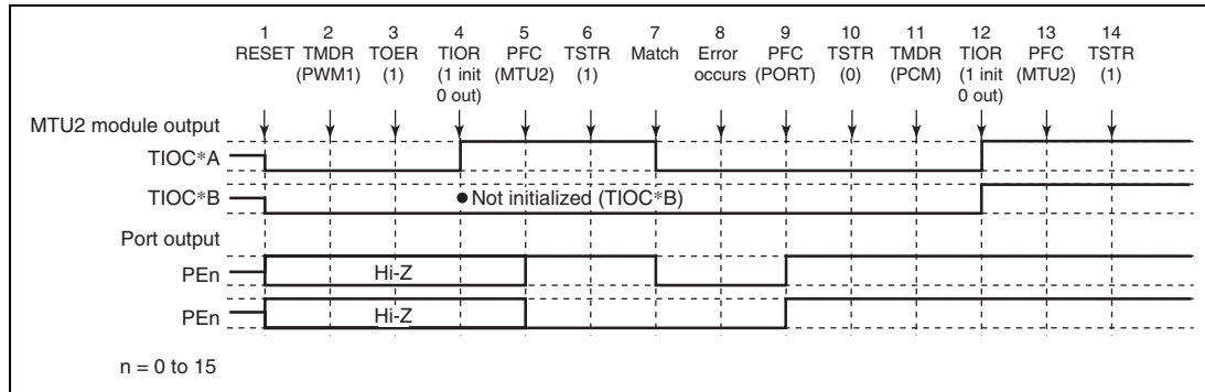
Figure 11.122 Error Occurrence in PWM Mode 1, Recovery in Phase Counting Mode
