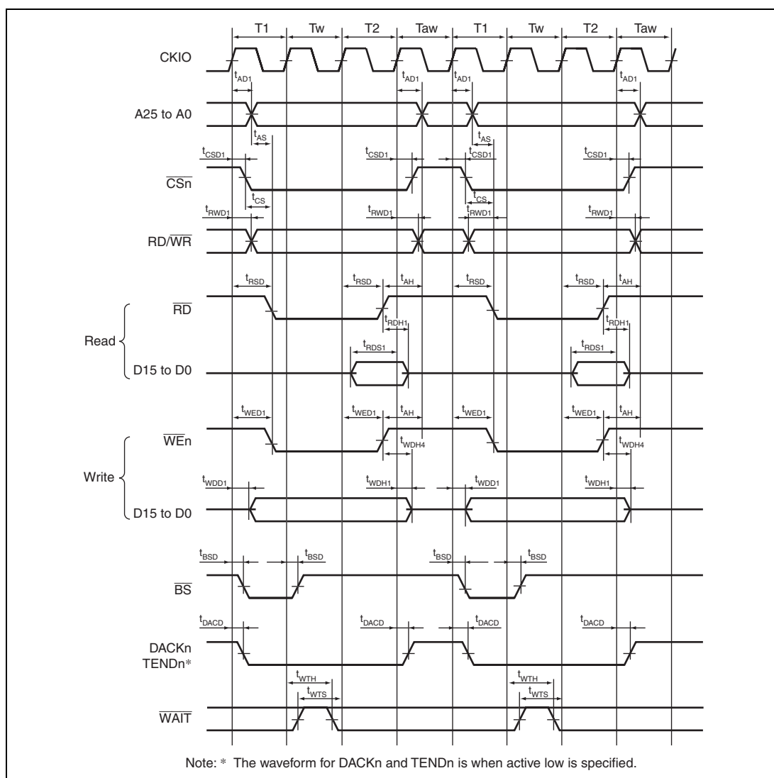
Figure 31.16 Basic Bus Timing for Normal Space (One Software Wait Cycle, External Wait Cycle Valid (WM Bit = 0), No Idle Cycle)
