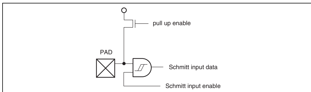
Figure 1.3 (2) Simplified Circuit Diagram (Schmitt AND Input Buffer with Pull-Up)
