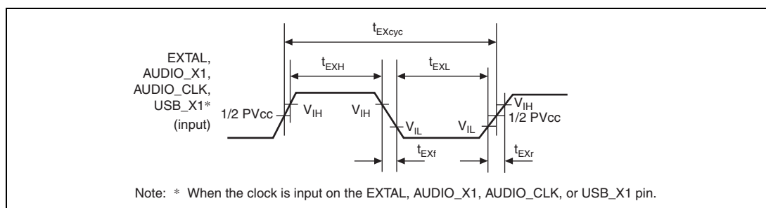
Figure 31.2 EXTAL, AUDIO_X1, AUDIO_CLK, and USB_X1 Clock Input Timing
