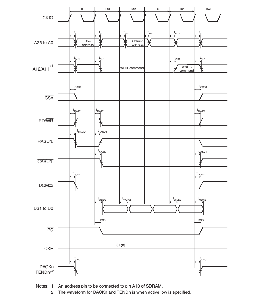
Figure 31.28 Synchronous DRAM Burst Write Bus Cycle (Four Write Cycles) (Auto Precharge, WTRCD = 0 Cycle, TRWL = 1 Cycle)
