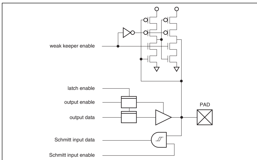
Figure 1.3 (10) Simplified Circuit Diagram (Bidirectional Buffer, Schmitt AND Input, with Latch and Weak Keeper)
