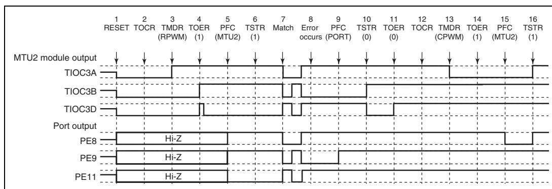
Figure 11.140 Error Occurrence in Reset-Synchronized PWM Mode, Recovery in Complementary PWM Mode
