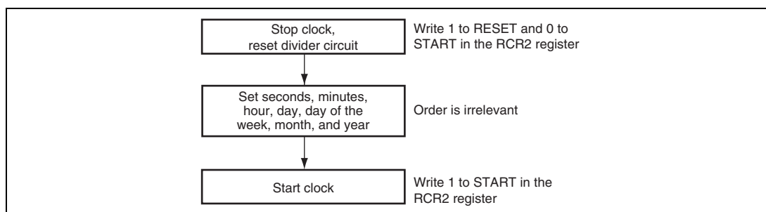
Figure 14.2 Setting Time
