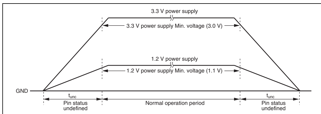
Figure 31.1 Power-on/Power-off Sequence
