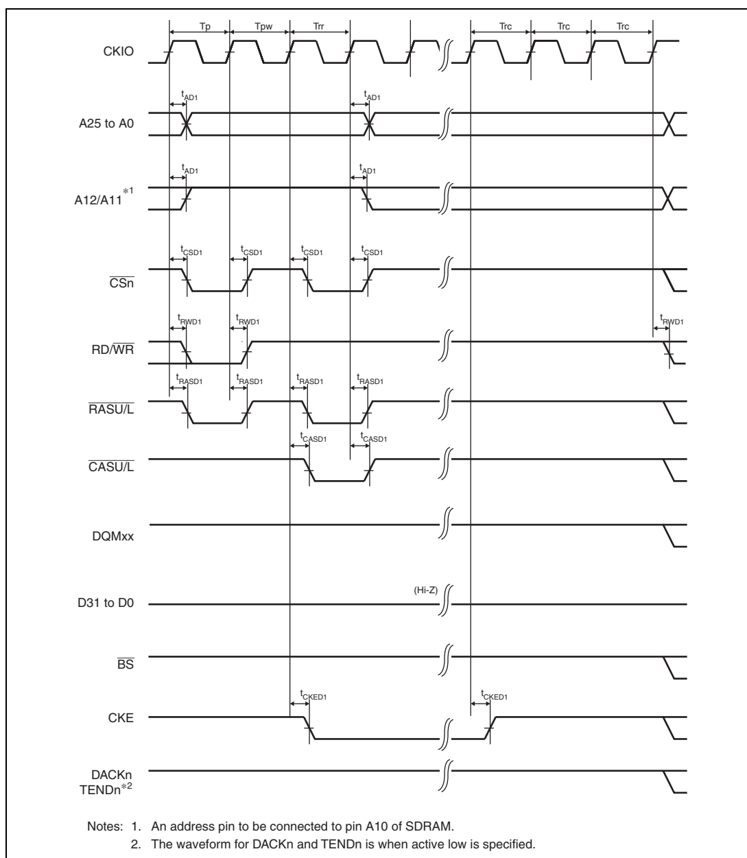
Figure 31.37 Synchronous DRAM Self-Refreshing Timing (WTRP = 1 Cycle)
