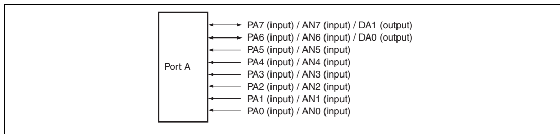
Figure 26.1 Port A
