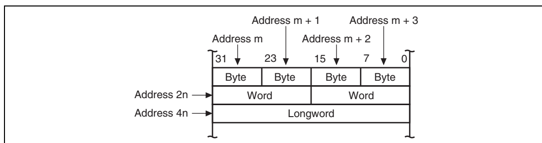
Figure 2.5 Data Formats in Memory
