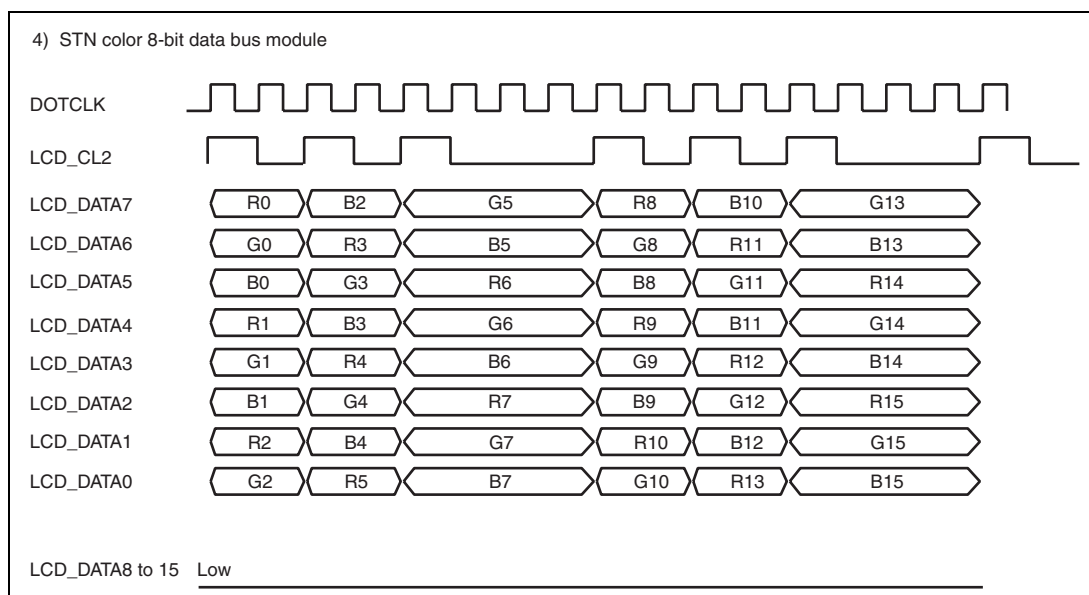
Figure 24.13 Clock and LCD Data Signal Example (STN Color 8-Bit Data Bus Module)
