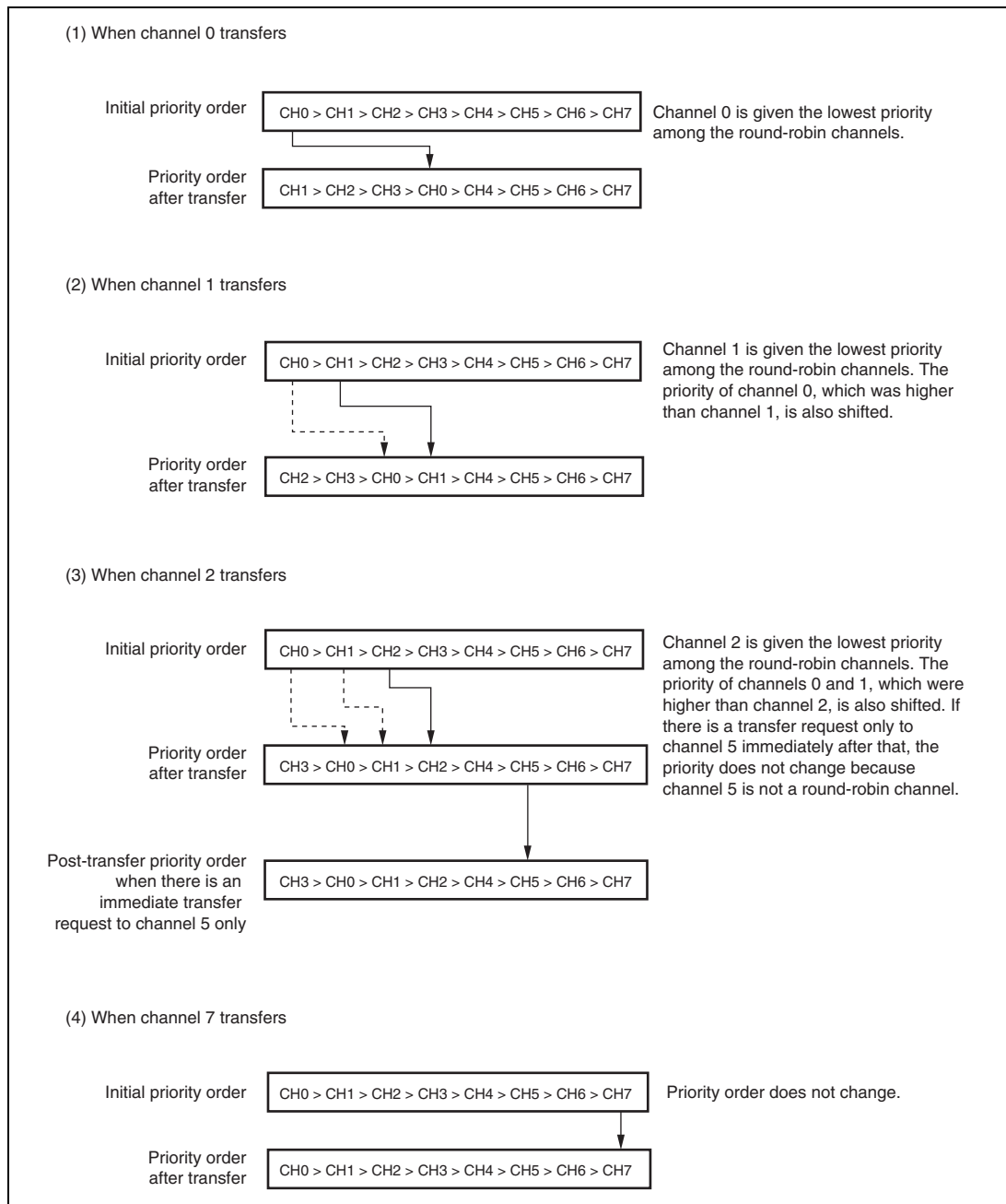
Figure 10.3 Round-Robin Mode
