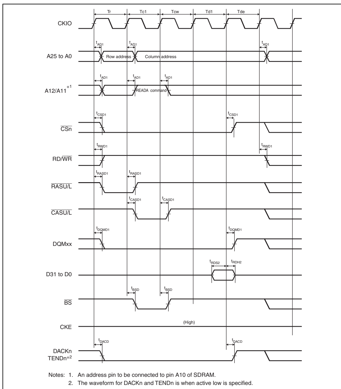
Figure 31.22 Synchronous DRAM Single Read Bus Cycle (Auto Precharge, CAS Latency 2, WTRCD = 0 Cycle, WTRP = 0 Cycle)
