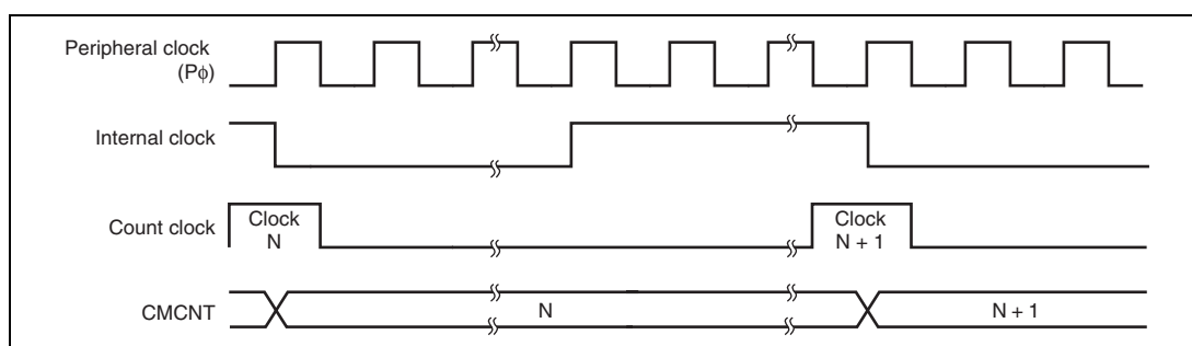
Figure 12.3 Count Timing
