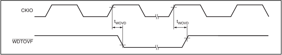
Figure 31.50 WDT Timing
