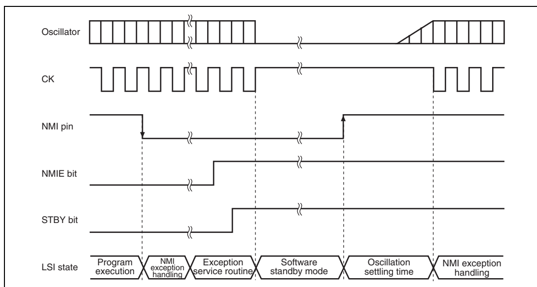
Figure 28.1 NMI Timing in Software Standby Mode (Application Example)
