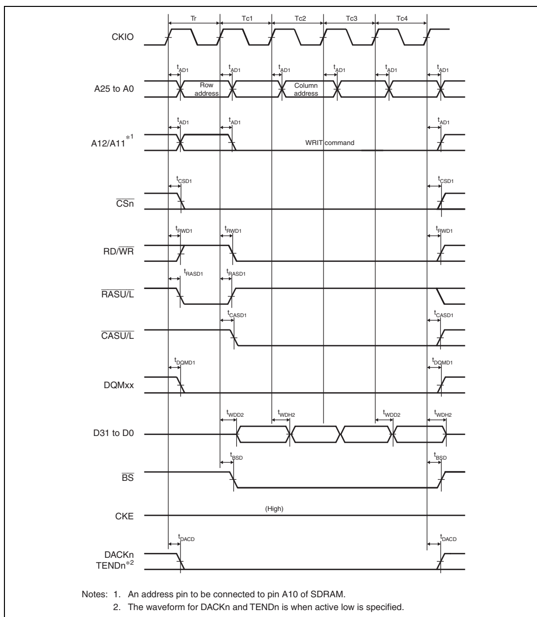
Figure 31.33 Synchronous DRAM Burst Write Bus Cycle (Four Write Cycles) (Bank Active Mode: ACT + WRITE Commands, WTRCD = 0 Cycle, TRWL = 0 Cycle)
