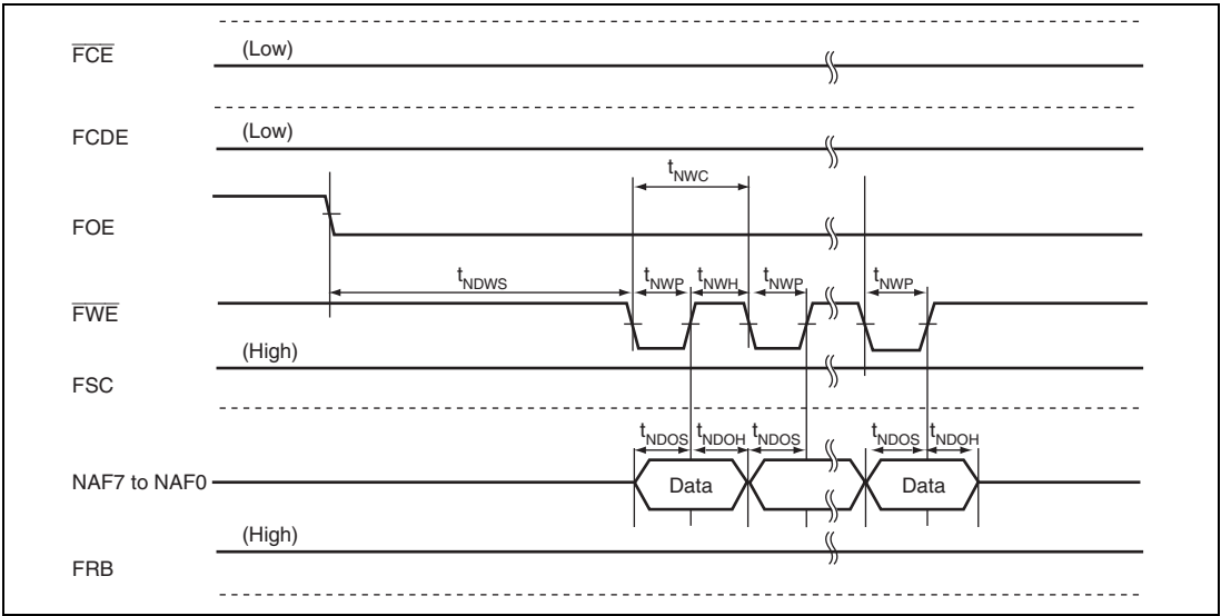
Figure 31.72 NAND Type Flash Memory Data Write Timing
