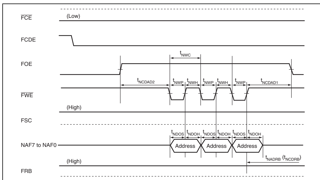
Figure 31.70 NAND Type Flash Memory Address Issuance Timing
