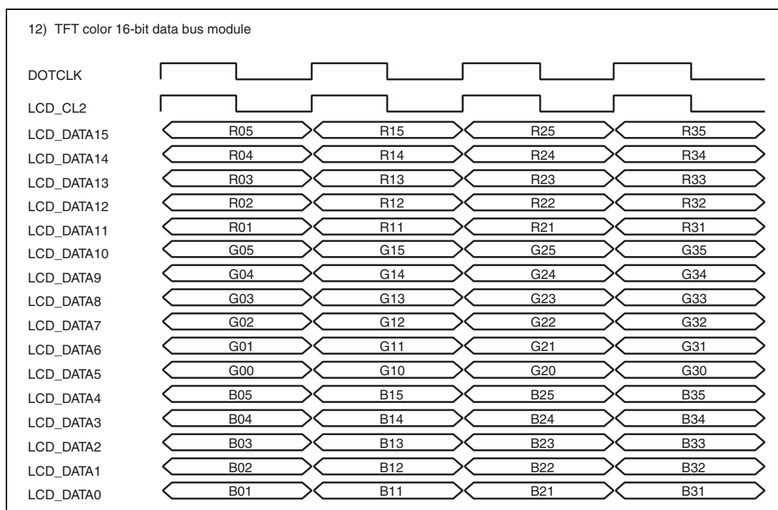
Figure 24.21 Clock and LCD Data Signal Example (TFT Color 16-Bit Data Bus Module)
