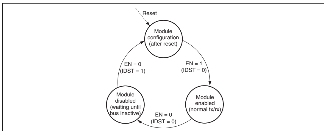
Figure 18.19 Operation Modes
