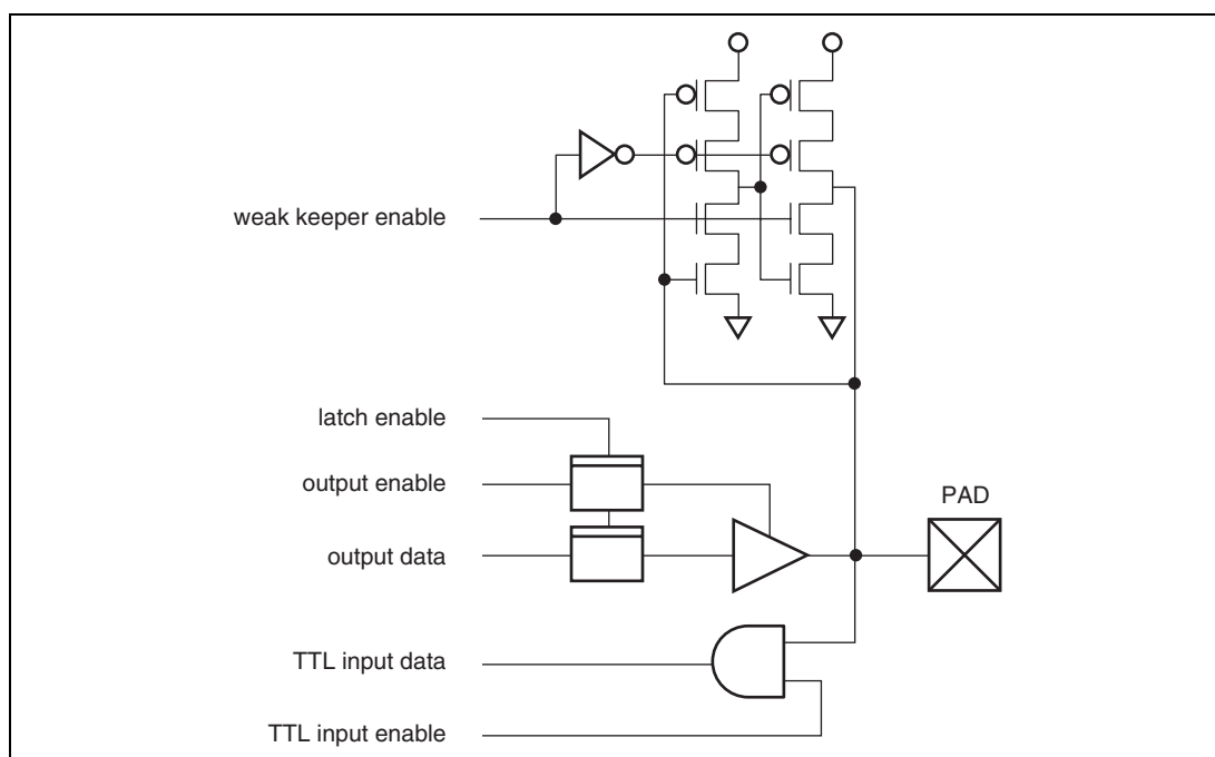
Figure 1.3 (9) Simplified Circuit Diagram (Bidirectional Buffer, TTL AND Input, with Latch and Weak Keeper)
