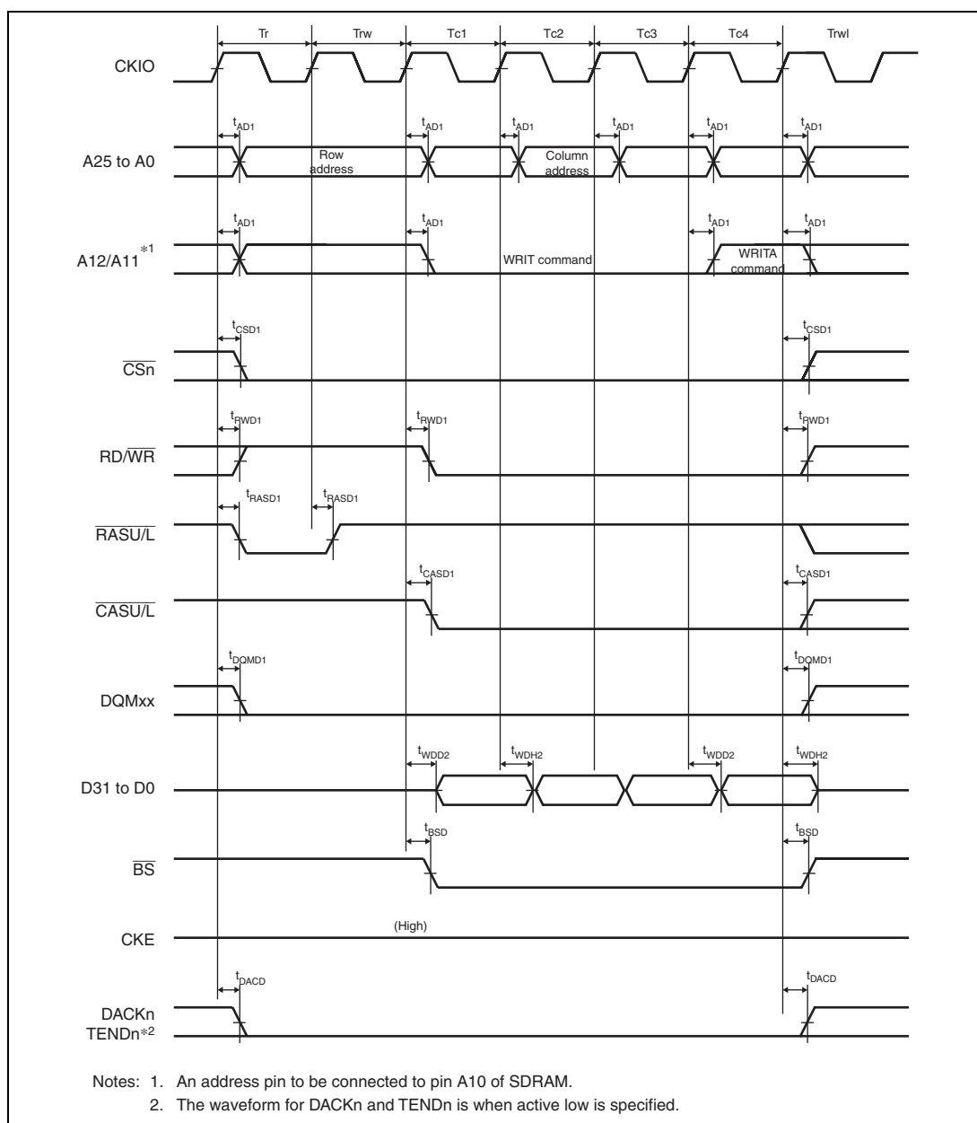
Figure 31.29 Synchronous DRAM Burst Write Bus Cycle (Four Write Cycles) (Auto Precharge, WTRCD = 1 Cycle, TRWL = 1 Cycle)
