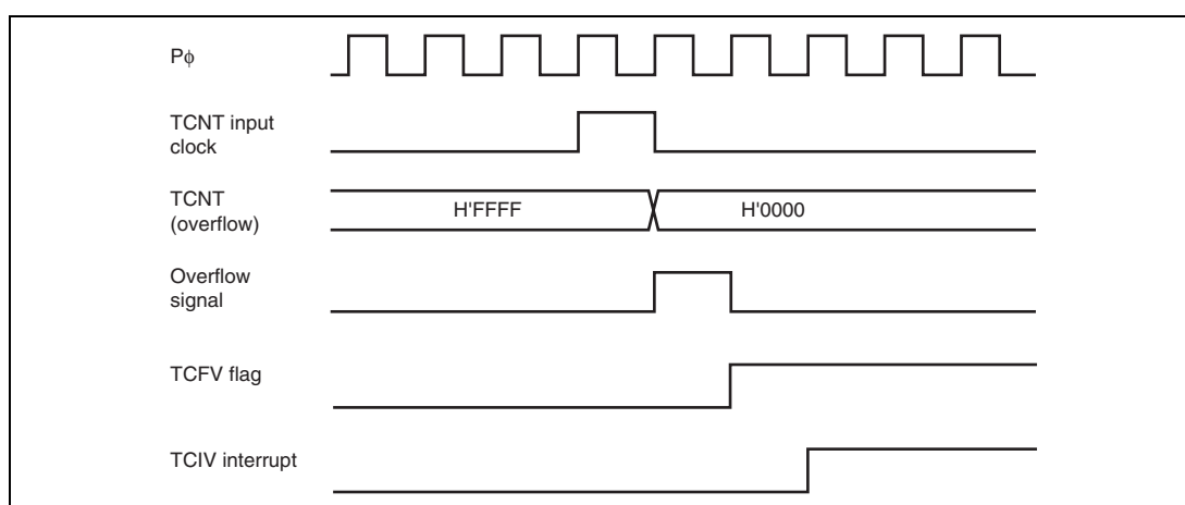
Figure 11.94 TCIV Interrupt Setting Timing
