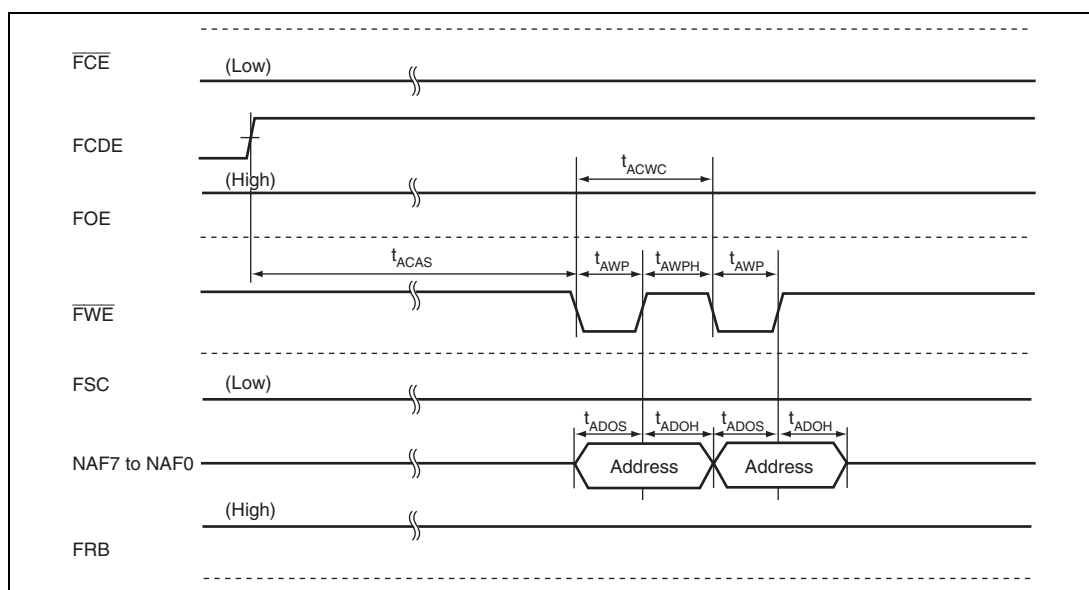
Figure 31.65 AND Type Flash Memory Address Issuance Timing
