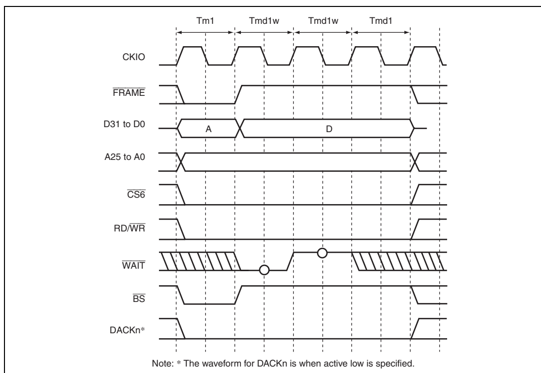
Figure 9.49 Burst MPX Space Access Timing (Single Write, Software Wait 1, Hardware Wait 1)
