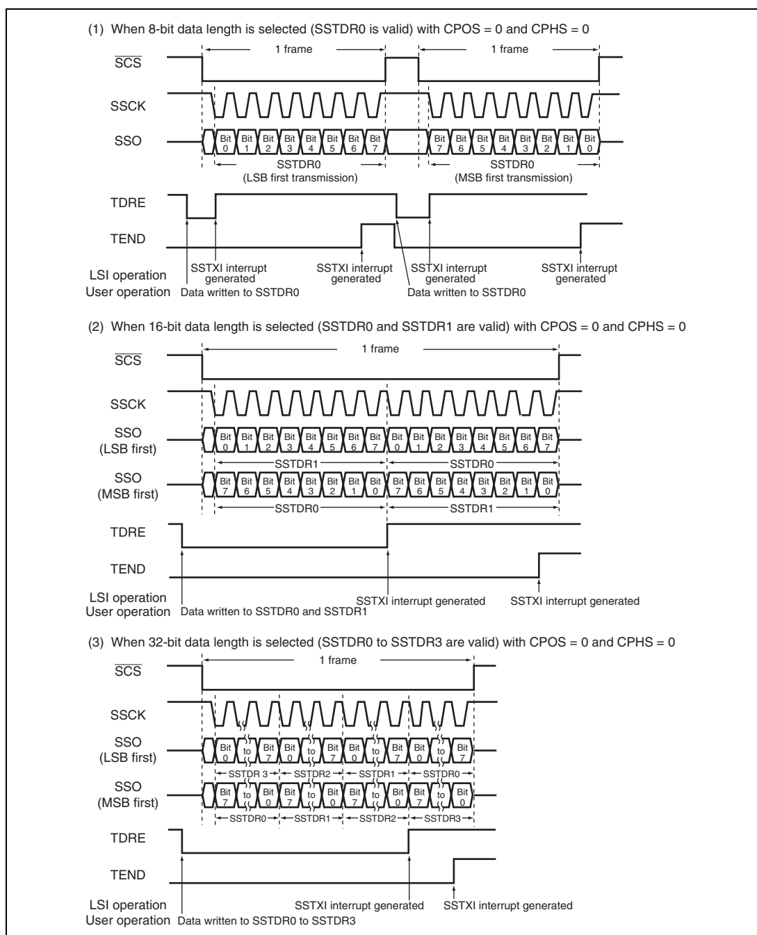
Figure 16.5 Example of Transmission Operation (SSU Mode)
