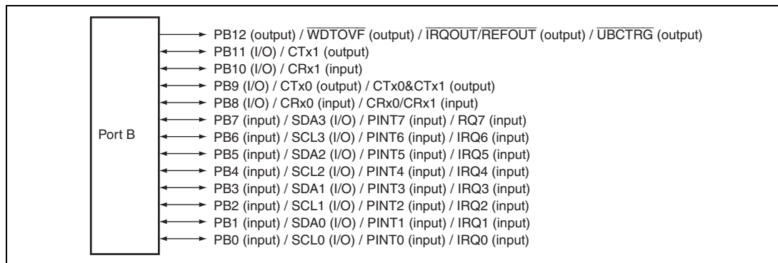
Figure 26.2 Port B
