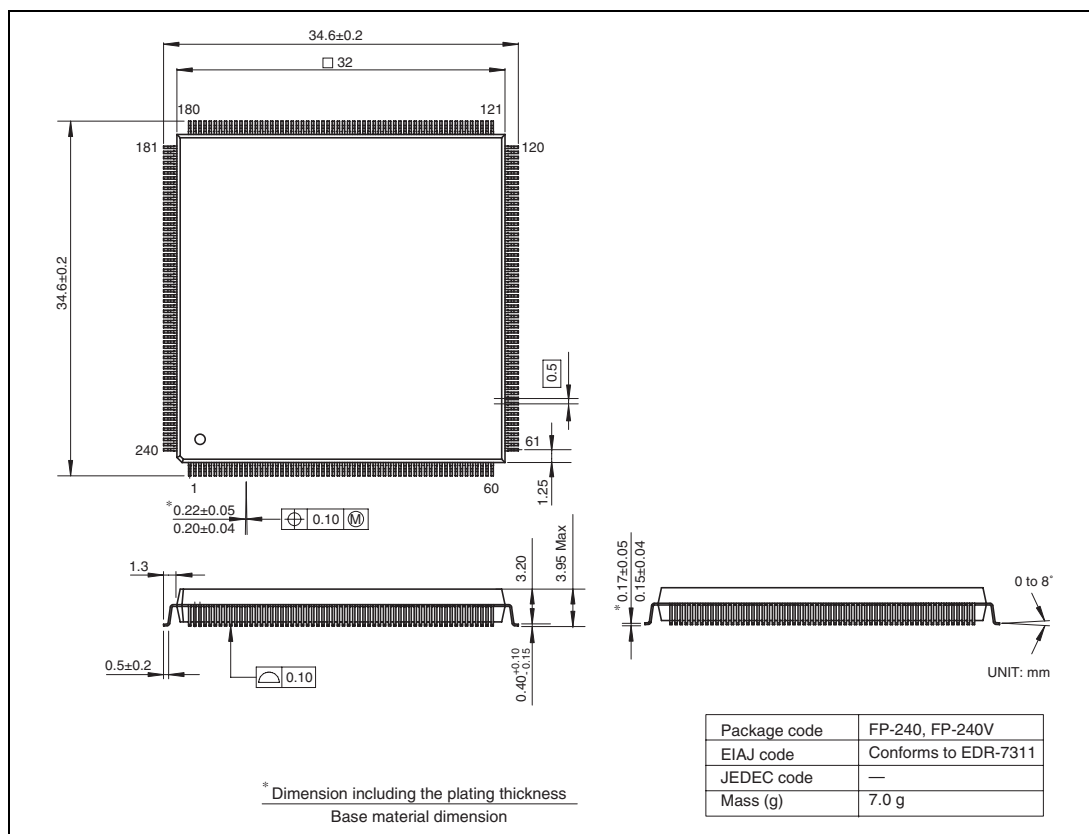
Figure C.1 Package Dimensions
