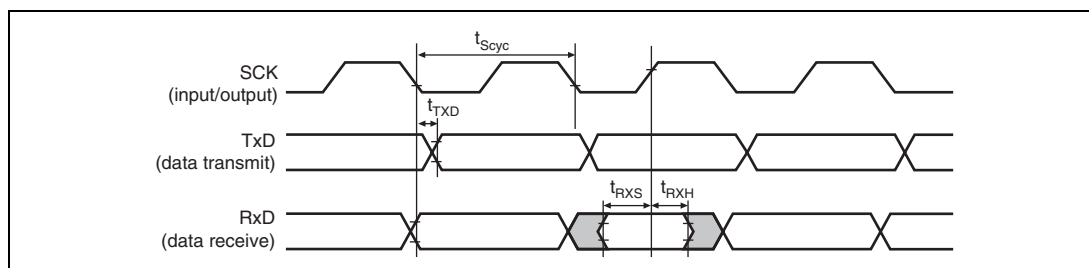
Figure 31.52 SCIF Input/Output Timing in Clocked Synchronous Mode
