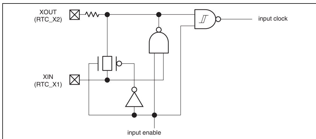
Figure 1.3 (14) Simplified Circuit Diagram (Oscillation Buffer 2)
