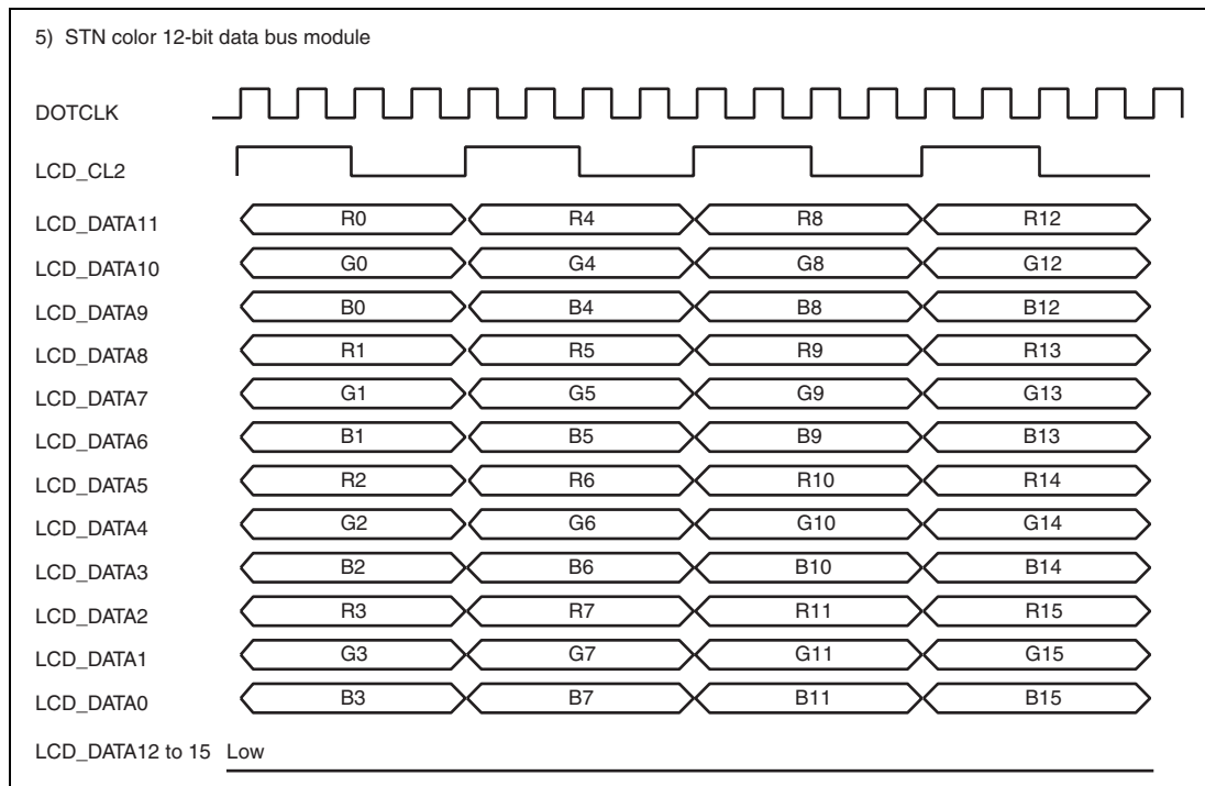
Figure 24.14 Clock and LCD Data Signal Example (STN Color 12-Bit Data Bus Module)
