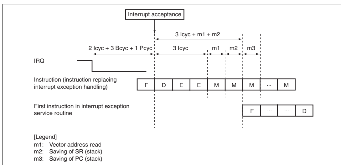
Figure 6.8 Example of Pipeline Operation when IRQ Interrupt Is Accepted (Register Banking with Register Bank Overflow)
