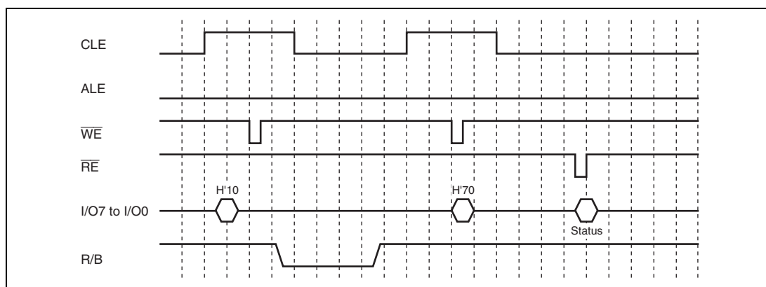
Figure 22.13 Programming Operation Timing for NAND-Type Flash Memory (2)
