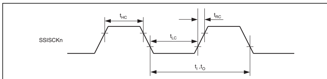
Figure 31.58 Clock Input/Output Timing
