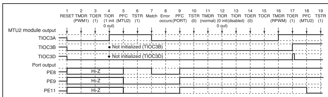
Figure 11.124 Error Occurrence in PWM Mode 1, Recovery in Reset-Synchronized PWM Mode
