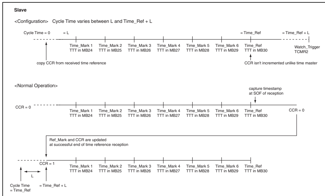
Figure 19.20 Time Slave
