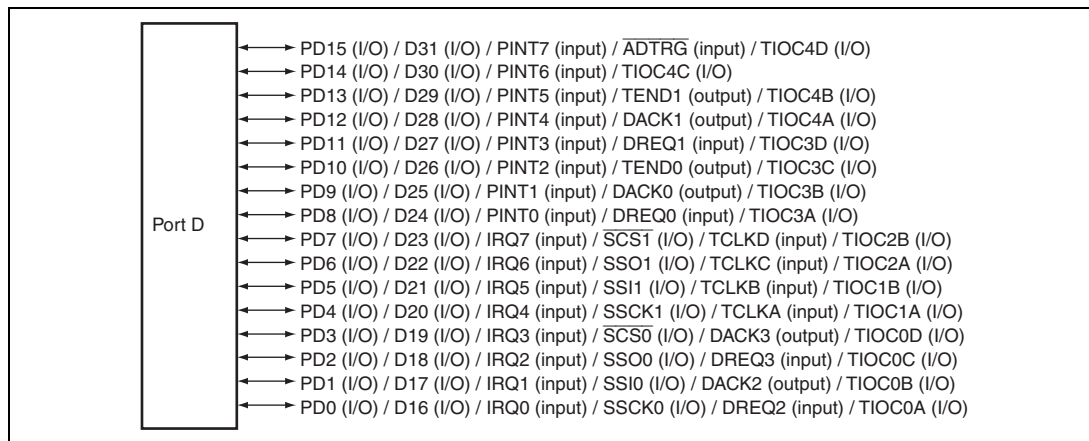
Figure 26.4 Port D
