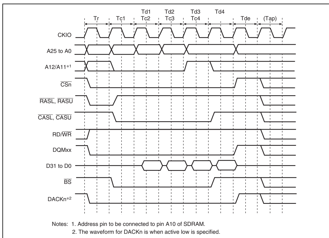
Figure 9.17 Burst Read Basic Timing (CAS Latency 1, Auto Pre-Charge)
