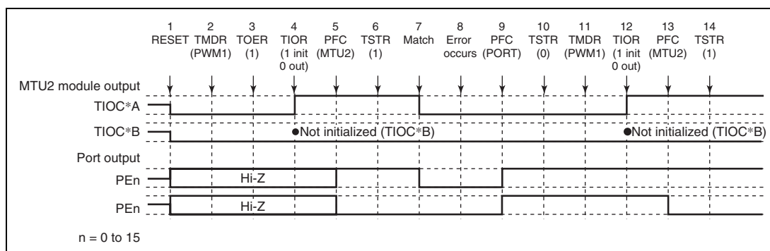
Figure 11.120 Error Occurrence in PWM Mode 1, Recovery in PWM Mode 1
