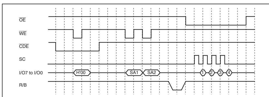
Figure 22.4 Read Operation Timing for AND-Type Flash Memory (1)
