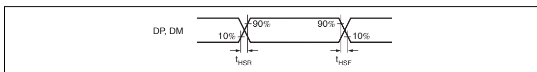
Figure 31.76 DP and DM Output Timing (High-Speed)
