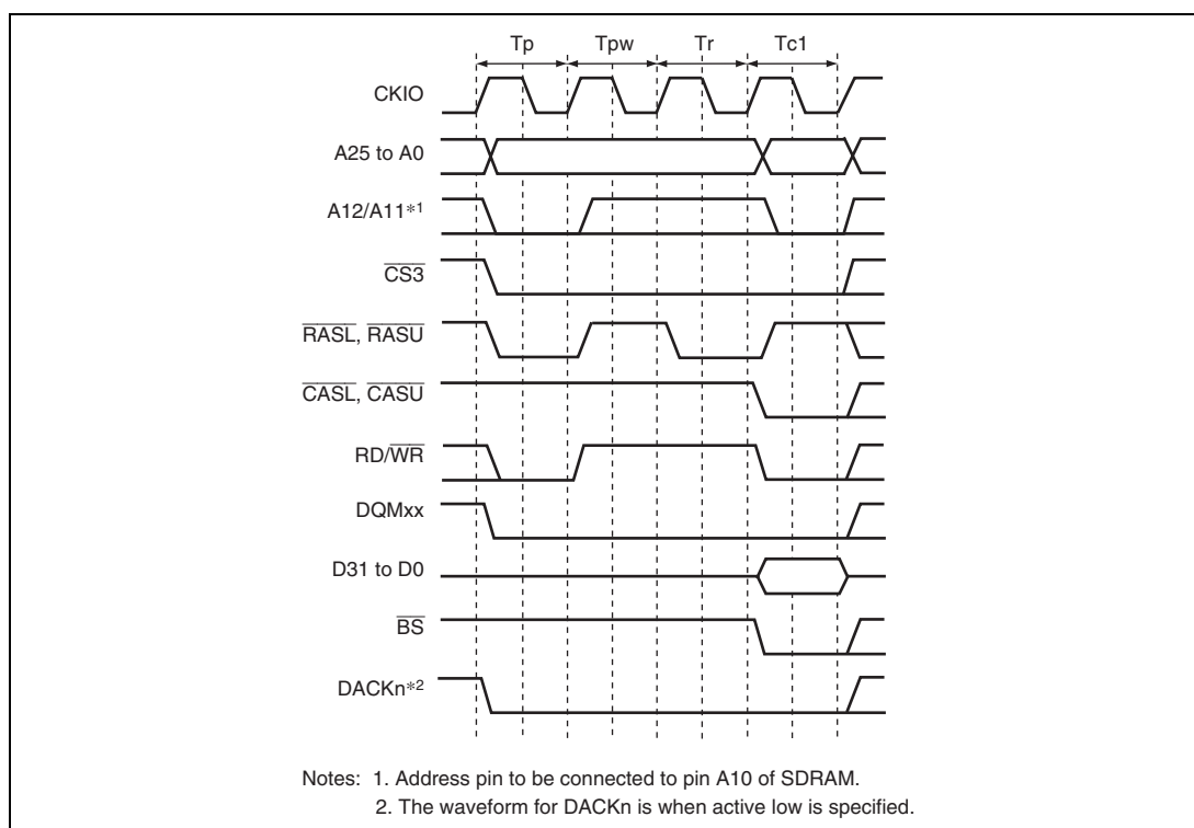
Figure 9.27 Single Write Timing (Bank Active, Different Row Addresses in the Same Bank)
