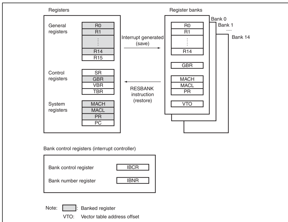
Figure 6.10 Overview of Register Bank Configuration
