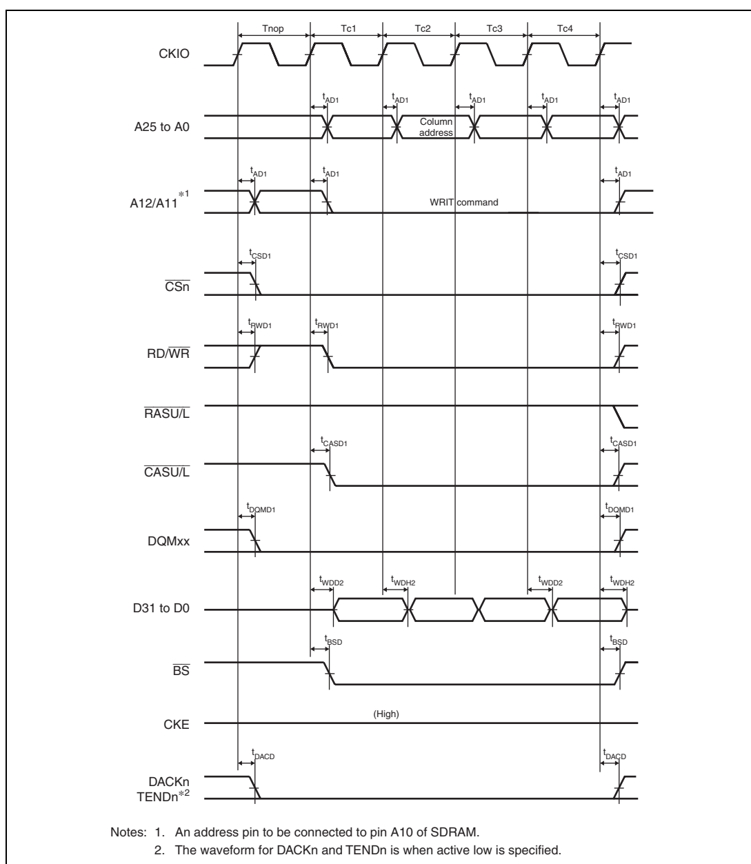
Figure 31.34 Synchronous DRAM Burst Write Bus Cycle (Four Write Cycles) (Bank Active Mode: WRITE Command, Same Row Address, WTRCD = 0 Cycle, TRWL = 0 Cycle)
