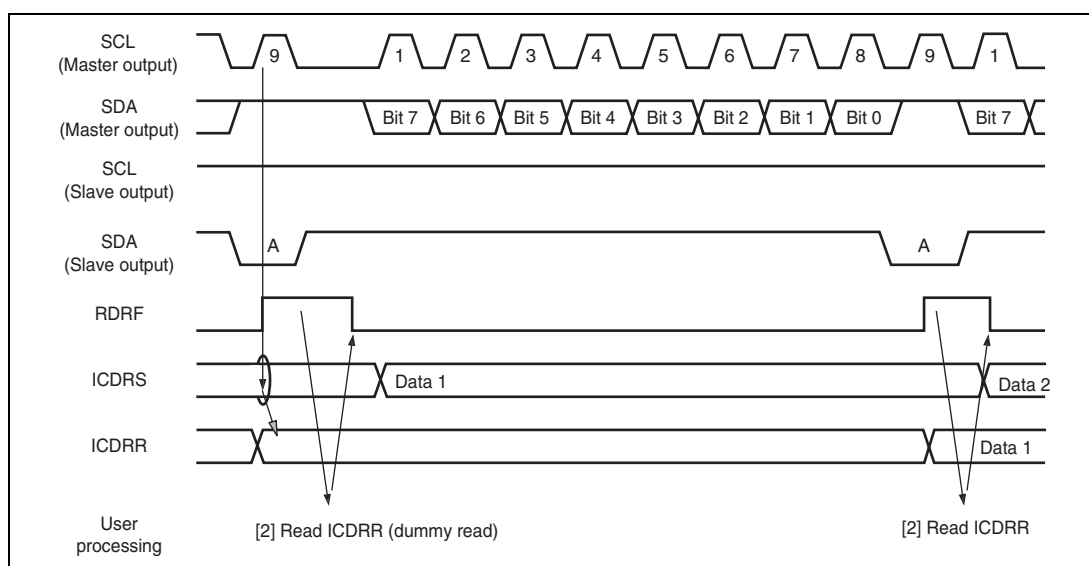
Figure 17.11 Slave Receive Mode Operation Timing (1)
