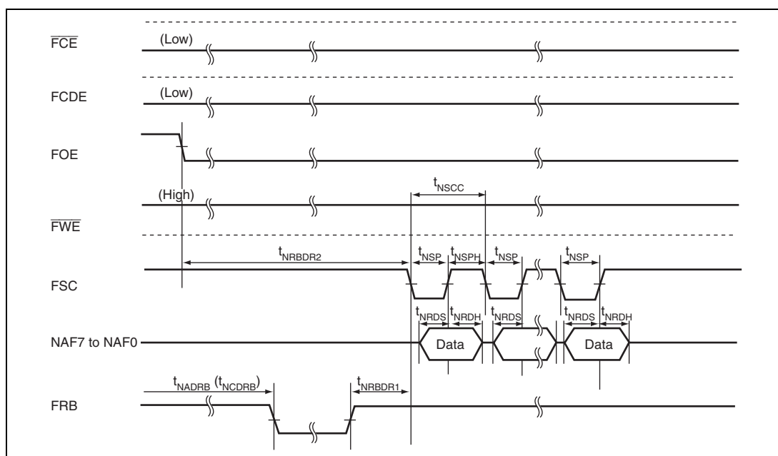
Figure 31.71 NAND Type Flash Memory Data Read Timing
