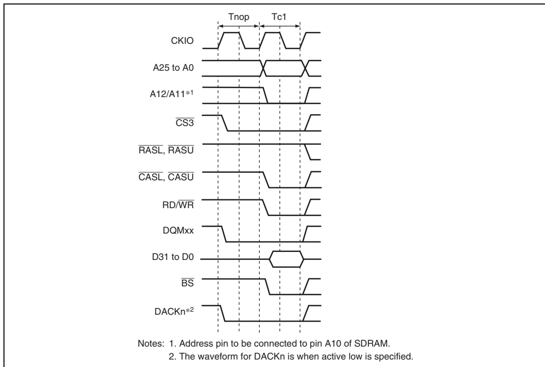
Figure 9.26 Single Write Timing (Bank Active, Same Row Addresses in the Same Bank)
