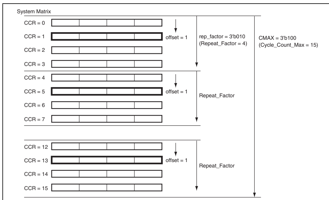
Figure 19.8 System Matrix
