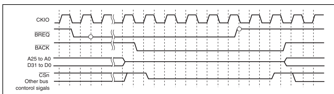
Figure 9.55 Bus Arbitration Timing
