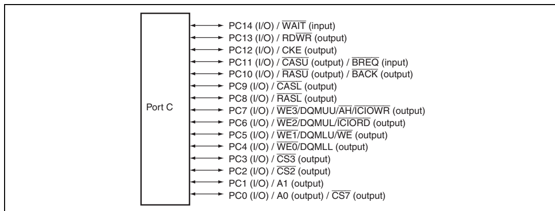
Figure 26.3 Port C
