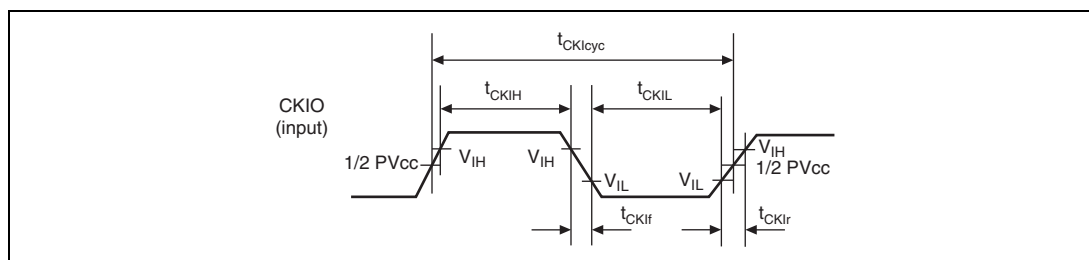
Figure 31.3 CKIO Clock Input Timing
