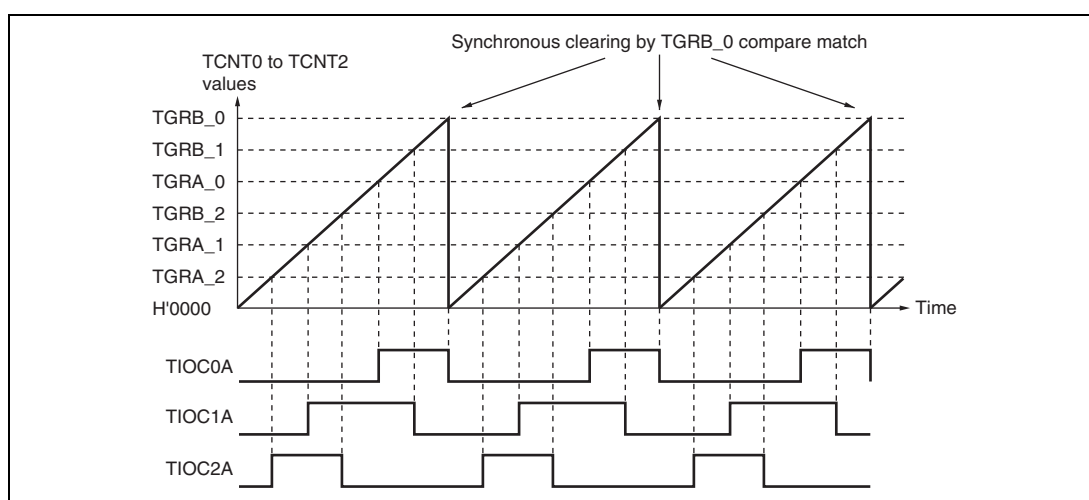
Figure 11.13 Example of Synchronous Operation
