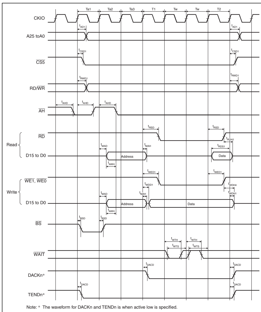
Figure 31.17 MPX-I/O Interface Bus Cycle (Three Address Cycles, One Software Wait Cycle, One External Wait Cycle)
