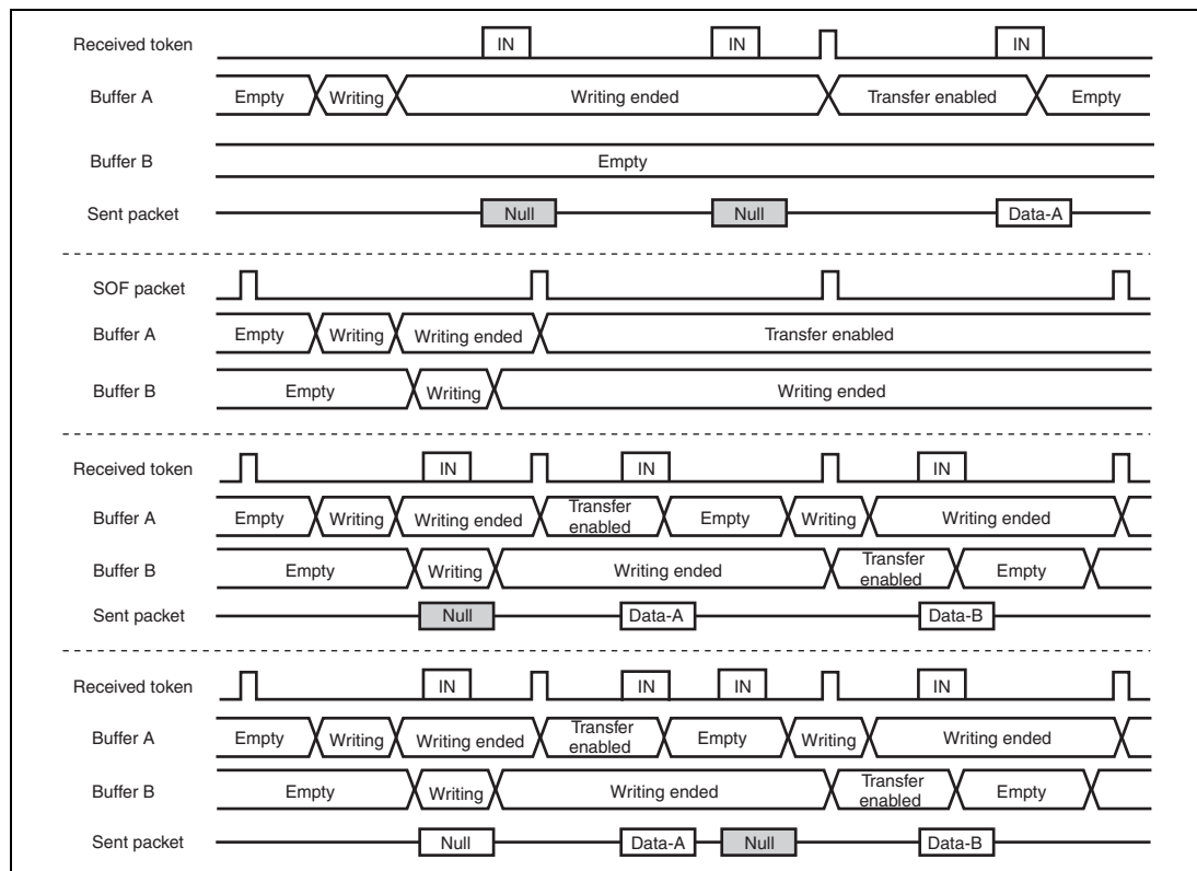
Figure 23.17 Example of Data Setup Function Operation
