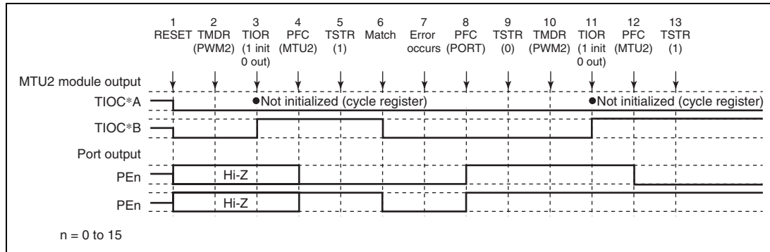
Figure 11.127 Error Occurrence in PWM Mode 2, Recovery in PWM Mode 2
