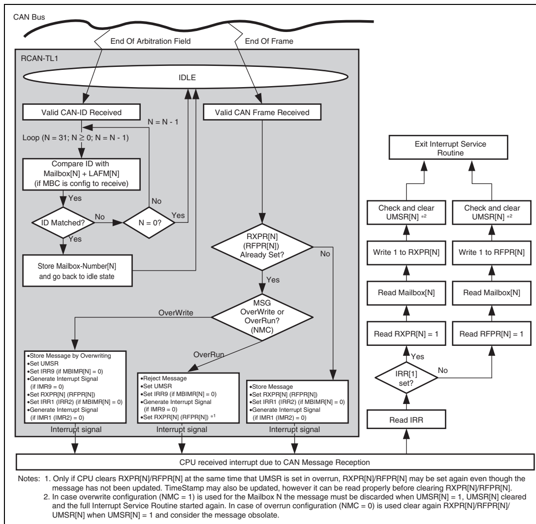
Figure 19.24 Message receive sequence
