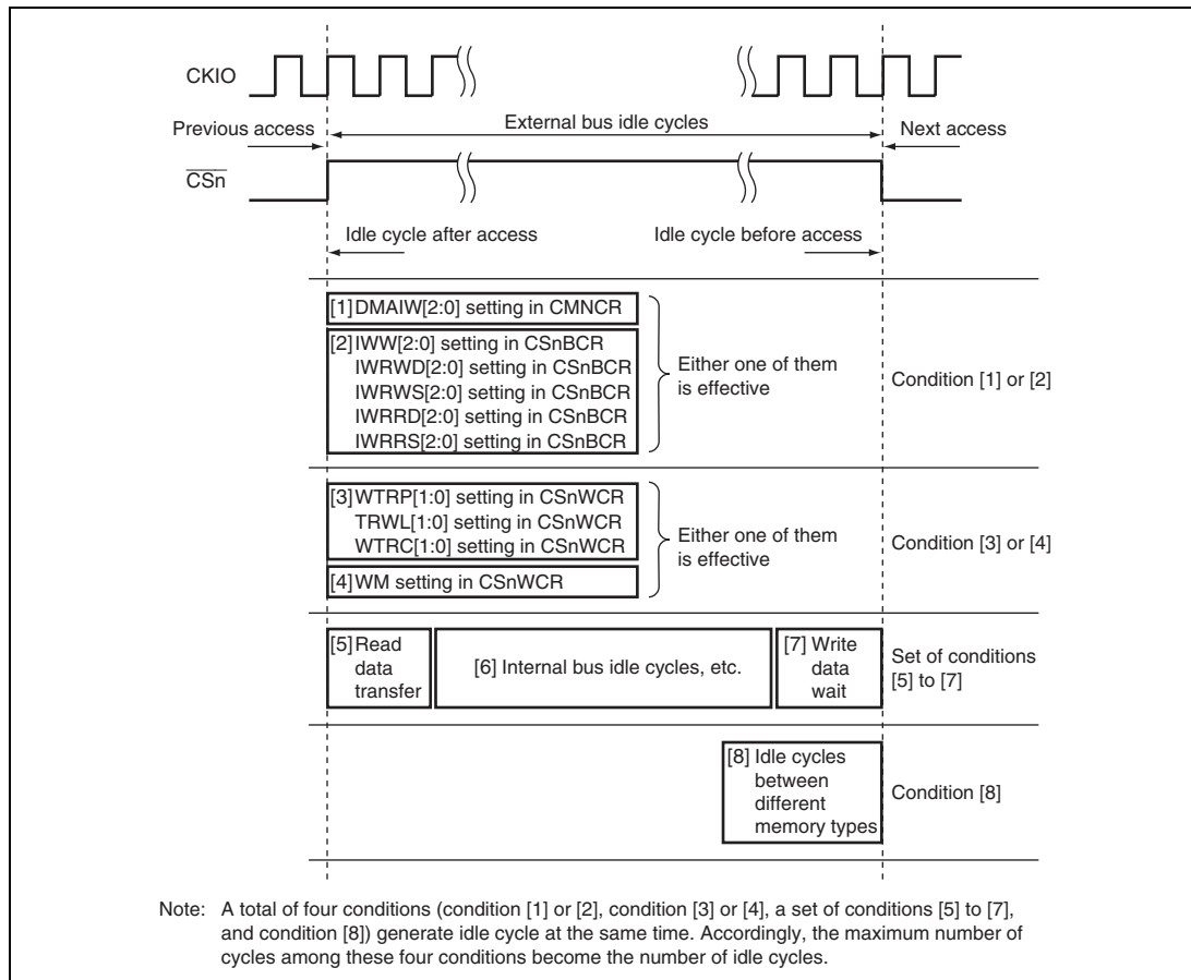
Figure 9.53 Idle Cycle Conditions
