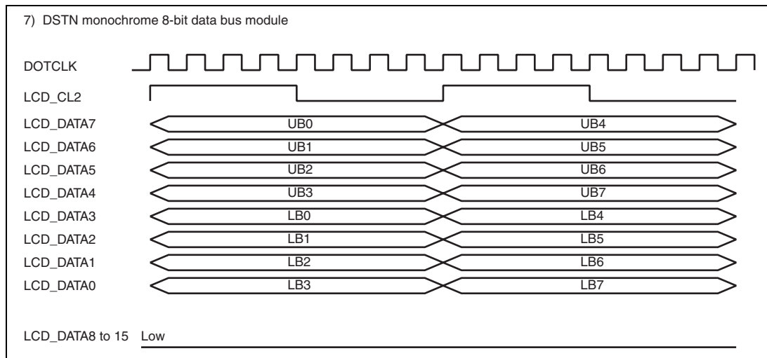
Figure 24.16 Clock and LCD Data Signal Example (DSTN Monochrome 8-Bit Data Bus Module)
