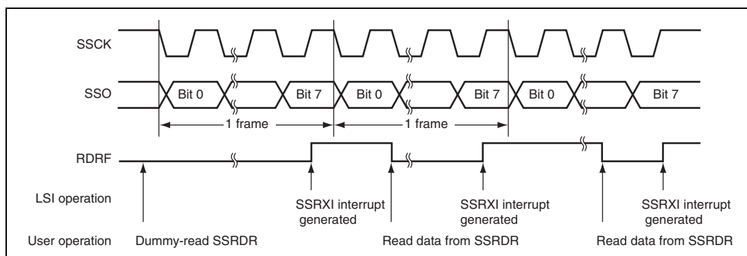
Figure 16.15 Example of Reception Operation (Clock Synchronous Communication Mode)
