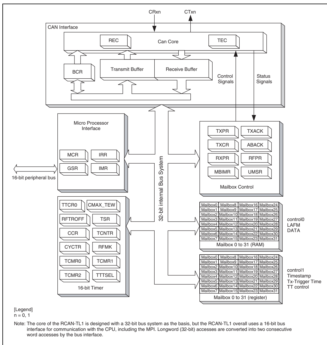
Figure 19.1 RCAN-TL1 architecture
