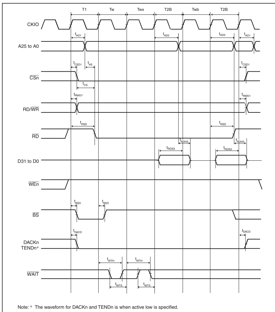
Figure 31.21 Burst ROM Read Cycle (One Software Wait Cycle, One Asynchronous External Burst Wait Cycle, Two Burst)
