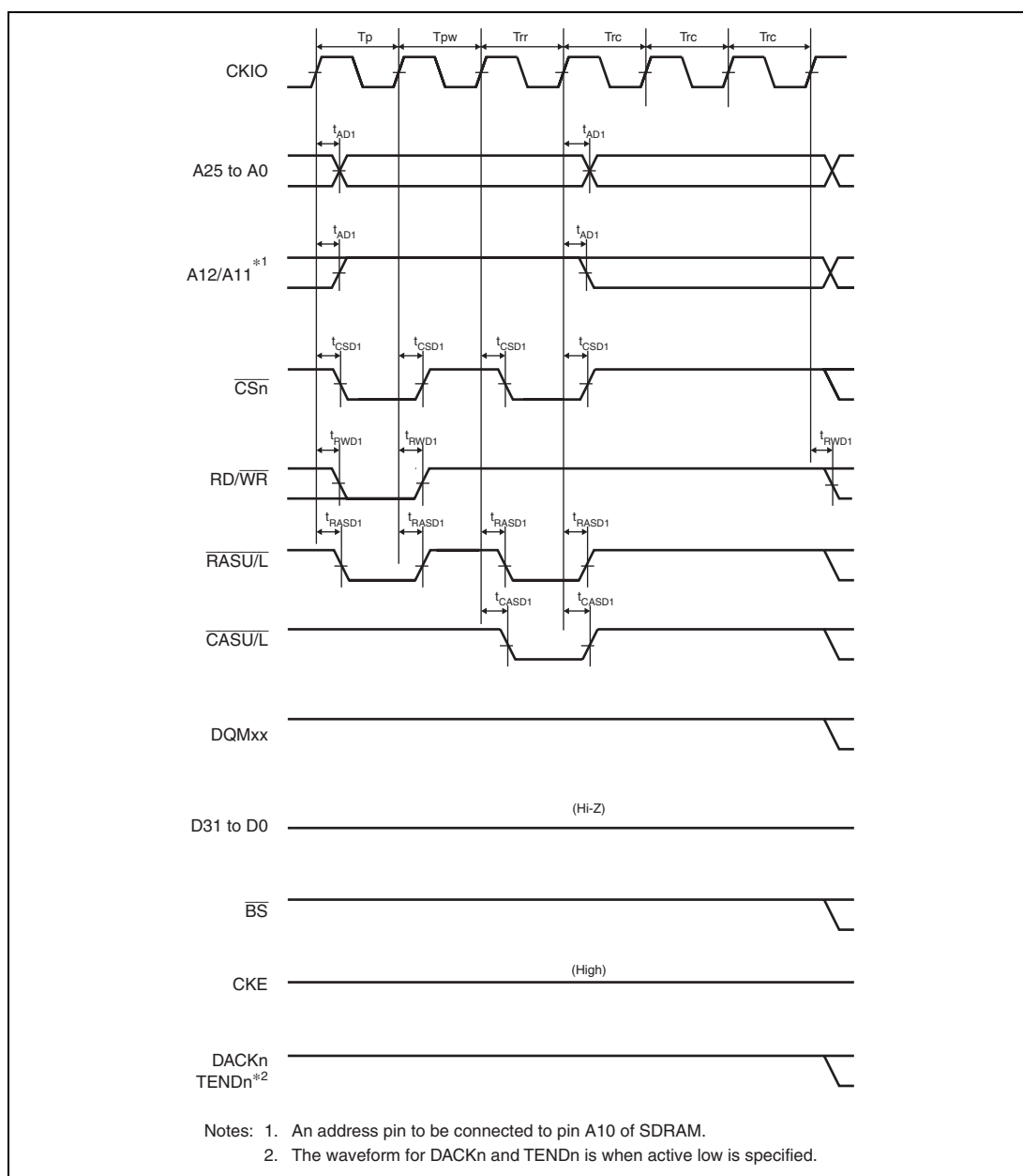
Figure 31.36 Synchronous DRAM Auto-Refreshing Timing (WTRP = 1 Cycle, WTRC = 3 Cycles)
