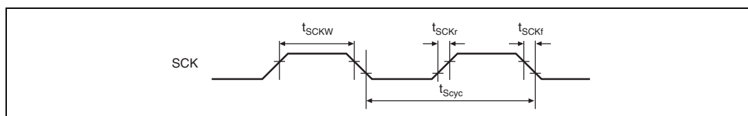
Figure 31.51 SCK Input Clock Timing
