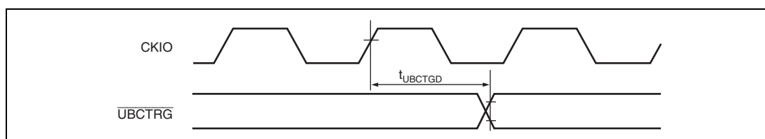
Figure 31.45 UBC Trigger Timing
