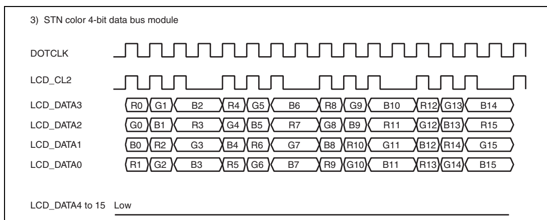
Figure 24.12 Clock and LCD Data Signal Example (STN Color 4-Bit Data Bus Module)
