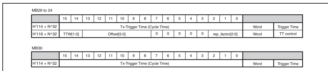
Figure 19.6 Tx-Trigger control field
