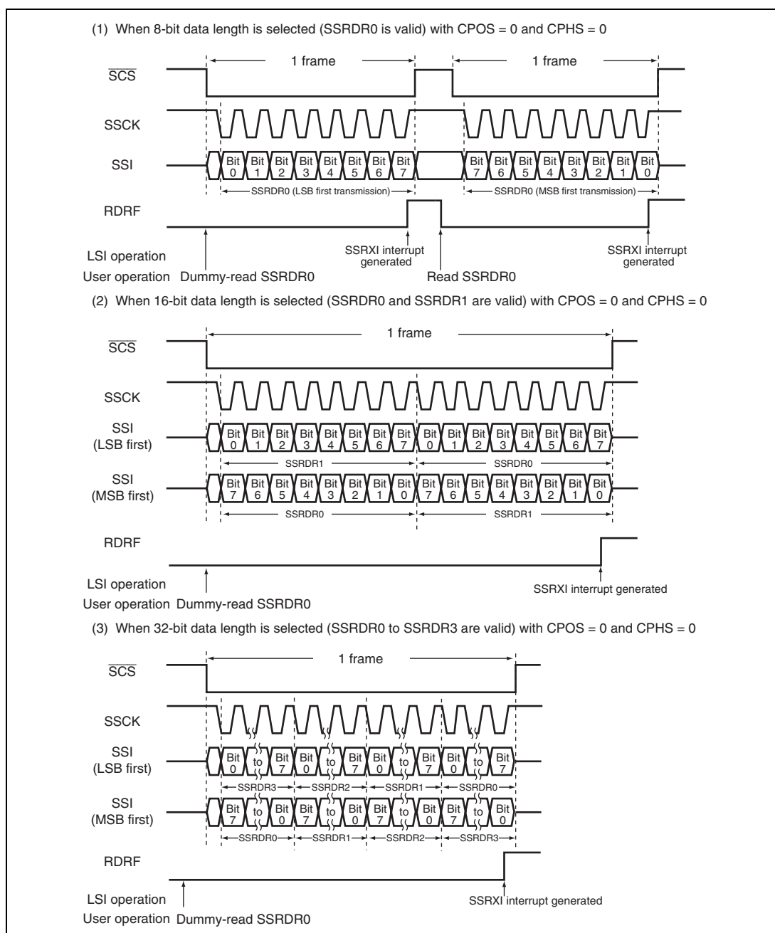
Figure 16.7 Example of Reception Operation (SSU Mode)
