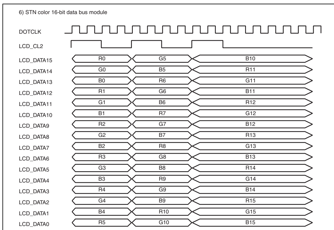
Figure 24.15 Clock and LCD Data Signal Example (STN Color 16-Bit Data Bus Module)
