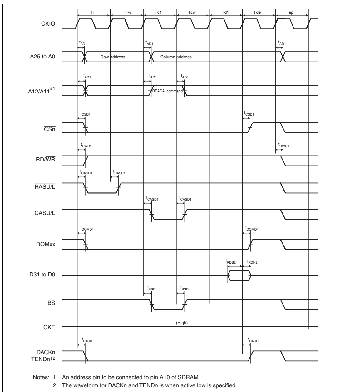
Figure 31.23 Synchronous DRAM Single Read Bus Cycle (Auto Precharge, CAS Latency 2, WTRCD = 1 Cycle, WTRP = 1 Cycle)
