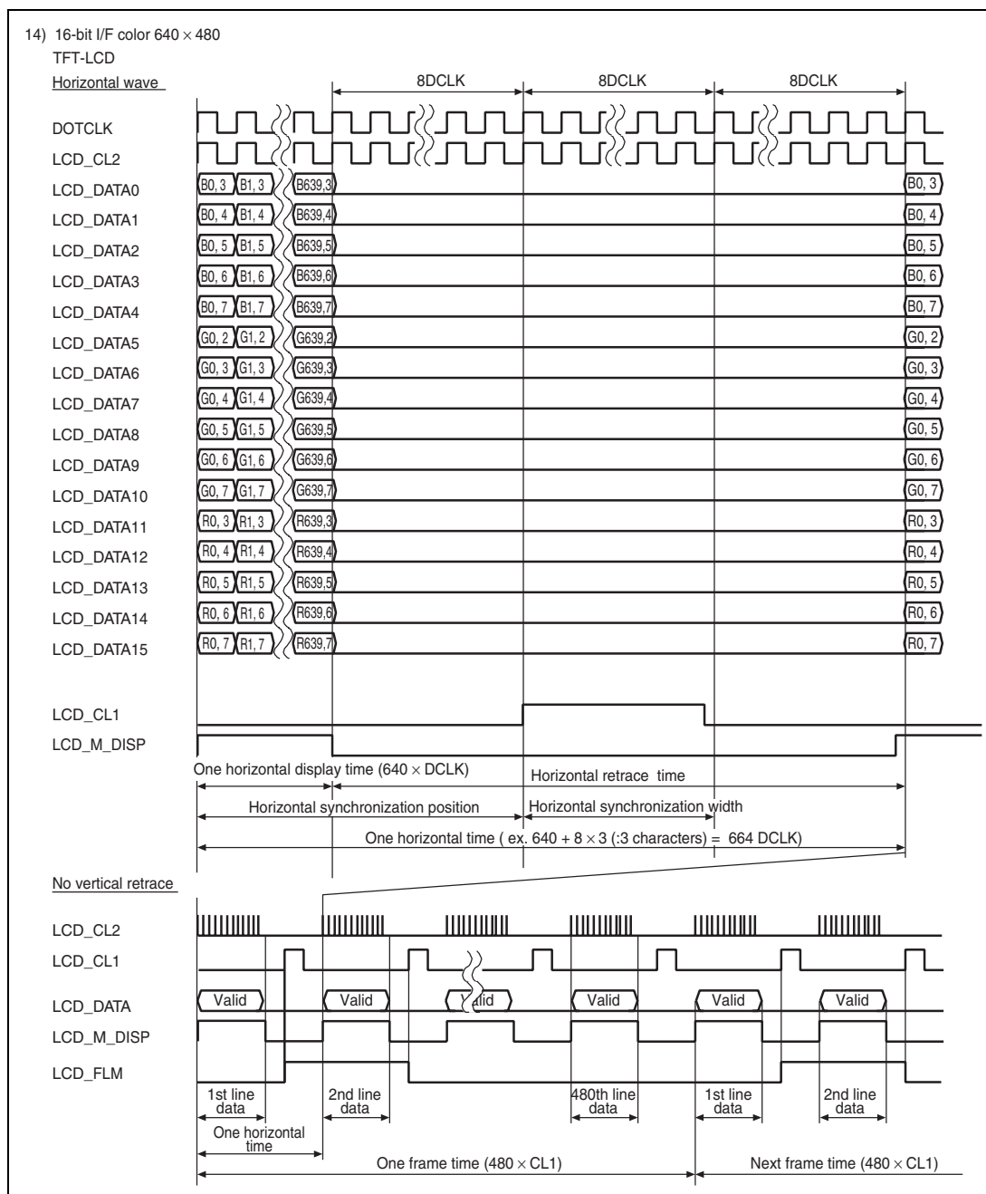
Figure 24.23 Clock and LCD Data Signal Example (16-Bit Interface Color 640 × 480)
