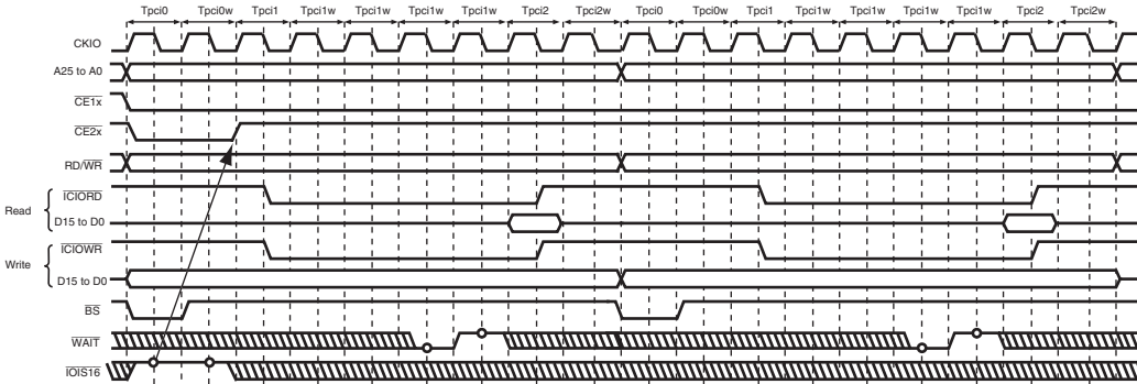
Figure 9.46 Dynamic Bus-Size Adjustment Timing for PCMCIA I/O Card Interface (TED[3:0] = B'0010, PCW[3:0] = B'0000, TEH[3:0] = B'0001, Hardware Wait = 1)
