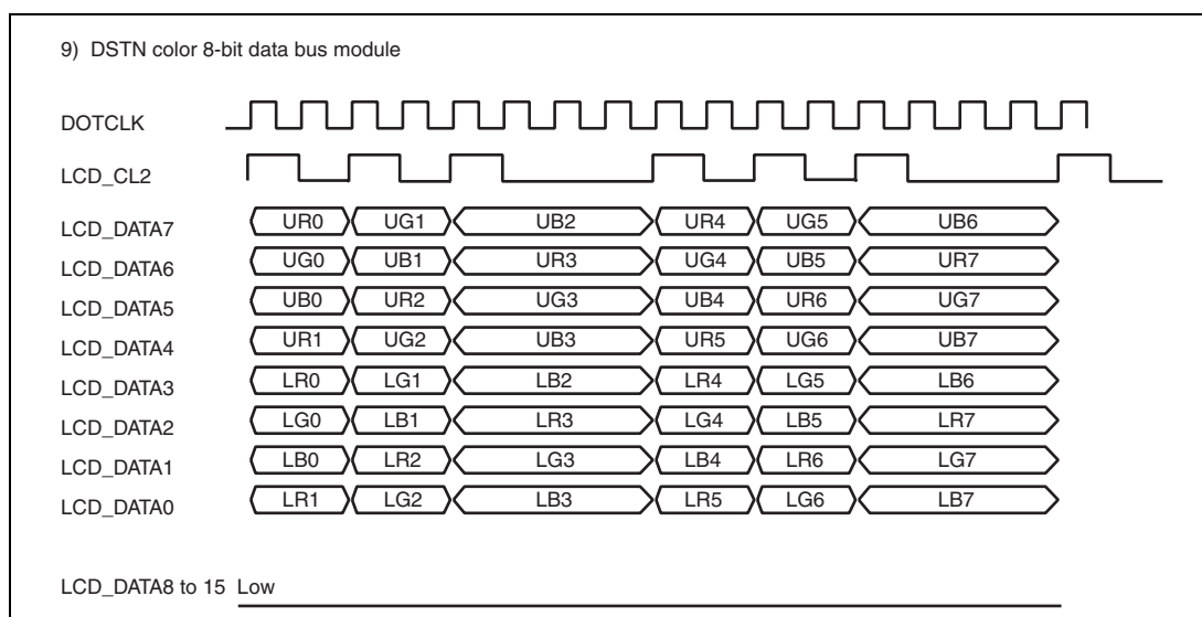
Figure 24.18 Clock and LCD Data Signal Example (DSTN Color 8-Bit Data Bus Module)
