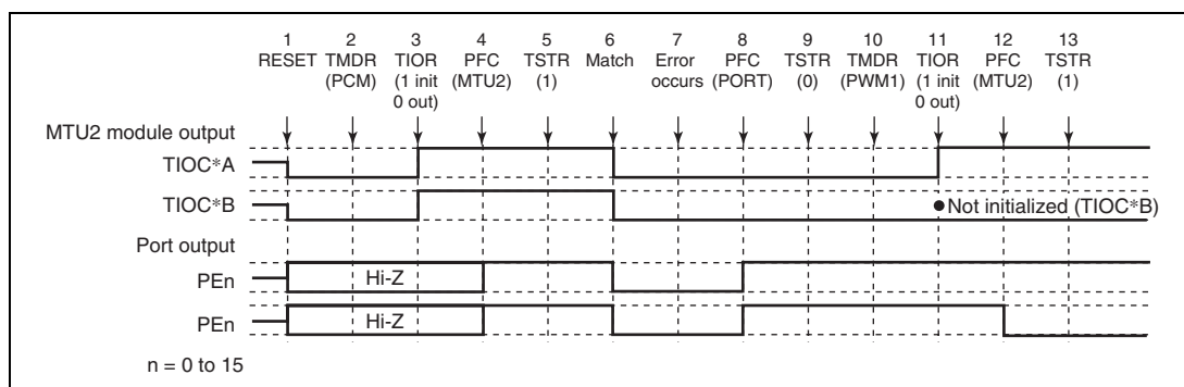
Figure 11.130 Error Occurrence in Phase Counting Mode, Recovery in PWM Mode 1
