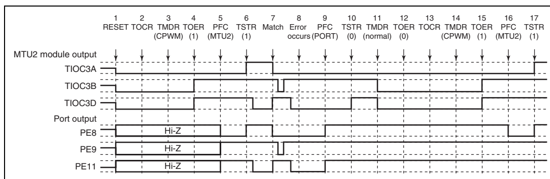
Figure 11.136 Error Occurrence in Complementary PWM Mode, Recovery in Complementary PWM Mode
