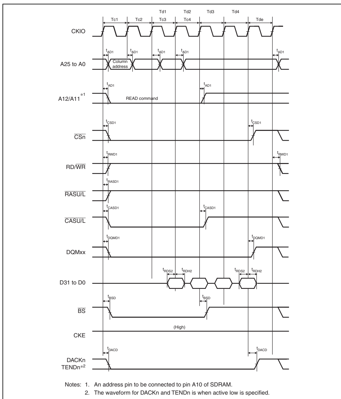
Figure 31.31 Synchronous DRAM Burst Read Bus Cycle (Four Read Cycles) (Bank Active Mode: READ Command, Same Row Address, CAS Latency 2, WTRCD = 0 Cycle)
