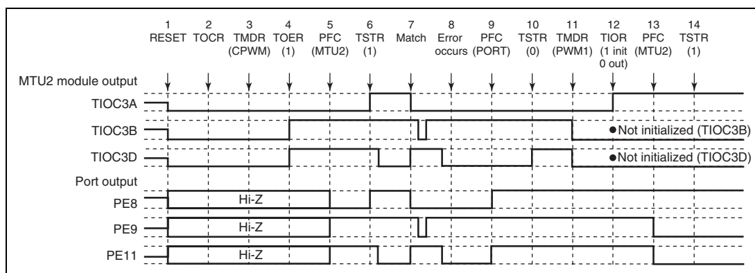
Figure 11.134 Error Occurrence in Complementary PWM Mode, Recovery in PWM Mode 1
