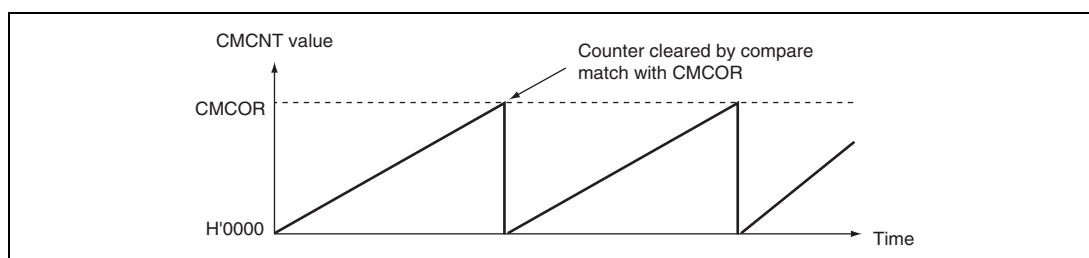
Figure 12.2 Counter Operation
