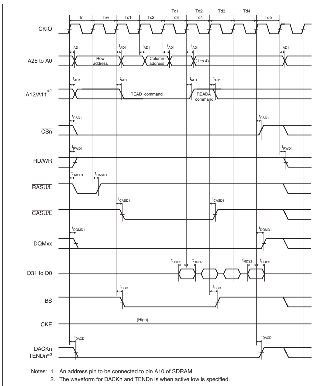
Figure 31.25 Synchronous DRAM Burst Read Bus Cycle (Four Read Cycles) (Auto Precharge, CAS Latency 2, WTRCD = 1 Cycle, WTRP = 0 Cycle)
