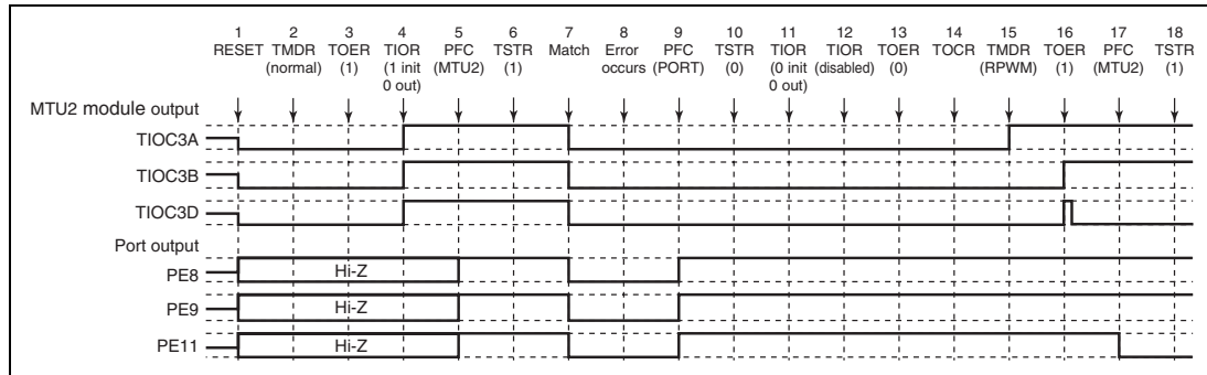
Figure 11.118 Error Occurrence in Normal Mode, Recovery in Reset-Synchronized PWM Mode
