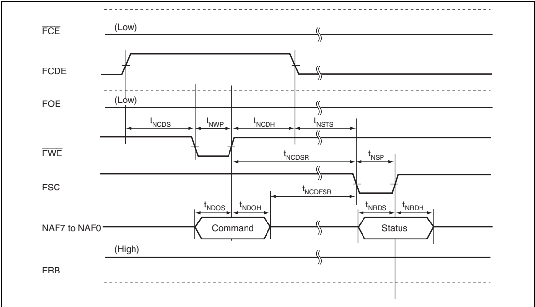
Figure 31.73 NAND Type Flash Memory Status Read Timing
