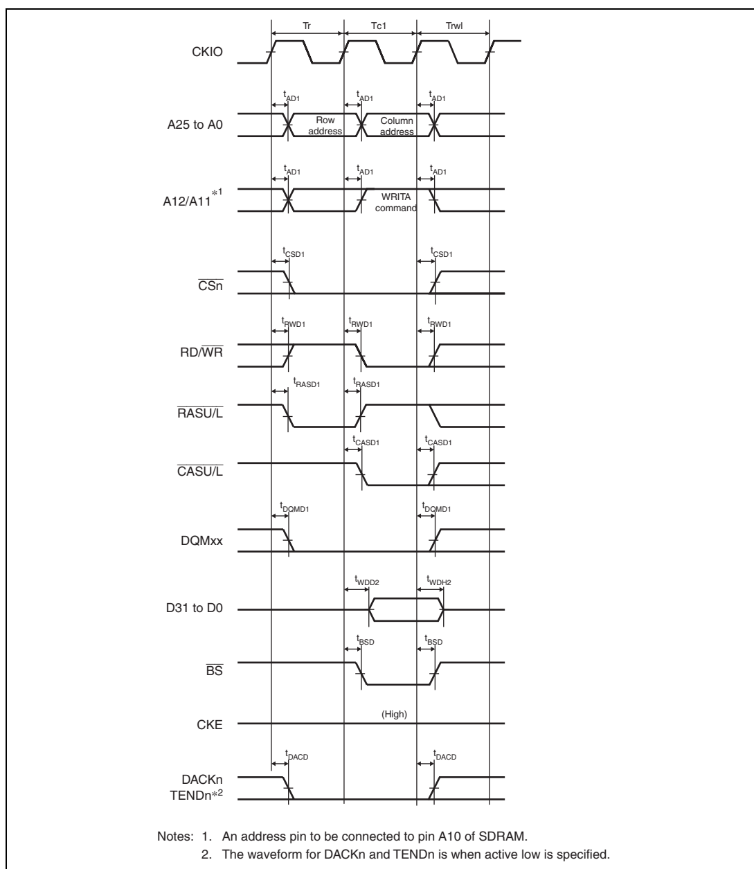
Figure 31.26 Synchronous DRAM Single Write Bus Cycle (Auto Precharge, TRWL = 1 Cycle)
