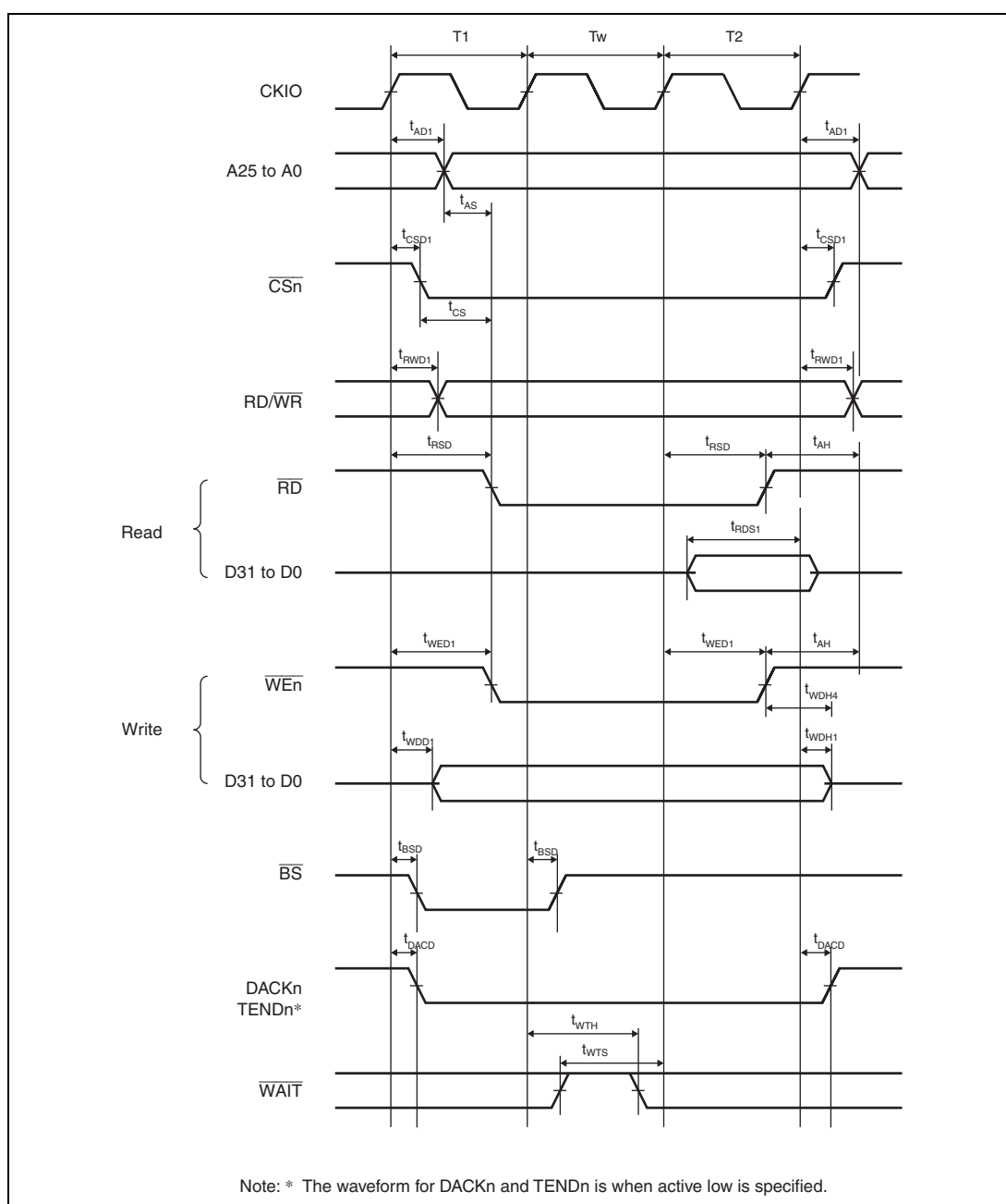
Figure 31.14 Basic Bus Timing for Normal Space (One Software Wait Cycle)
