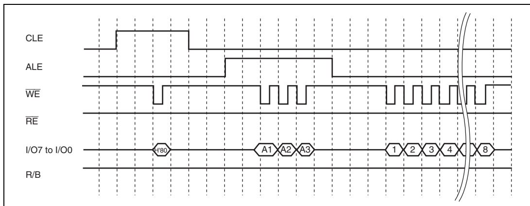
Figure 22.9 Programming Operation Timing for NAND-Type Flash Memory (1)
