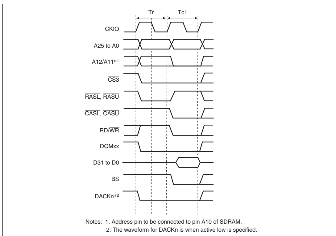
Figure 9.25 Single Write Timing (Bank Active, Different Bank)
