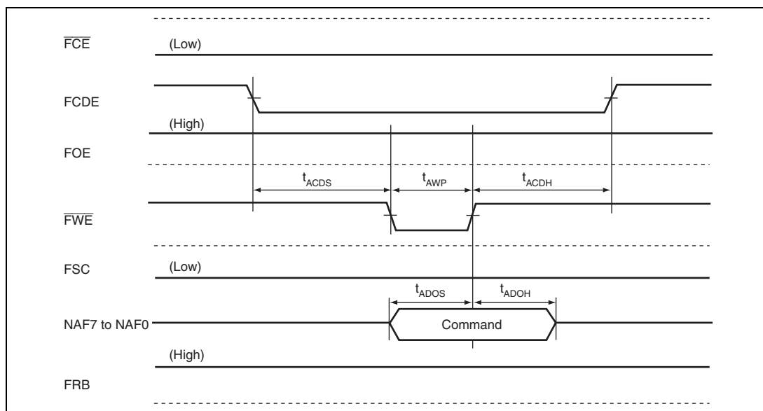
Figure 31.64 AND Type Flash Memory Command Issuance Timing
