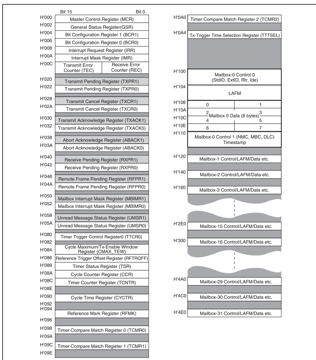
Figure 19.2 RCAN-TL1 Memory Map
