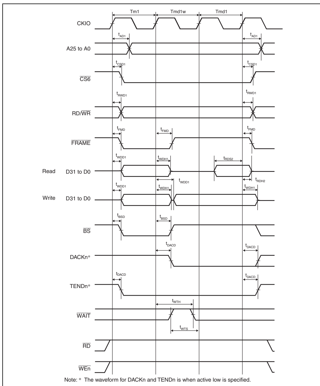
Figure 31.18 Burst MPX-I/O Interface Bus Cycle Single Read Write (One Address Cycle, One Software Wait Cycle)
