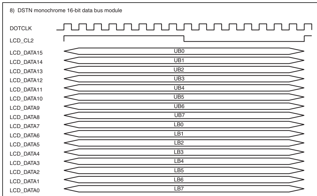
Figure 24.17 Clock and LCD Data Signal Example (DSTN Monochrome 16-Bit Data Bus Module)
