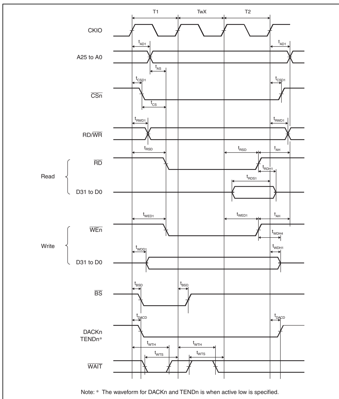
Figure 31.15 Basic Bus Timing for Normal Space (One External Wait Cycle)
