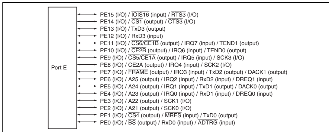
Figure 26.5 Port E
