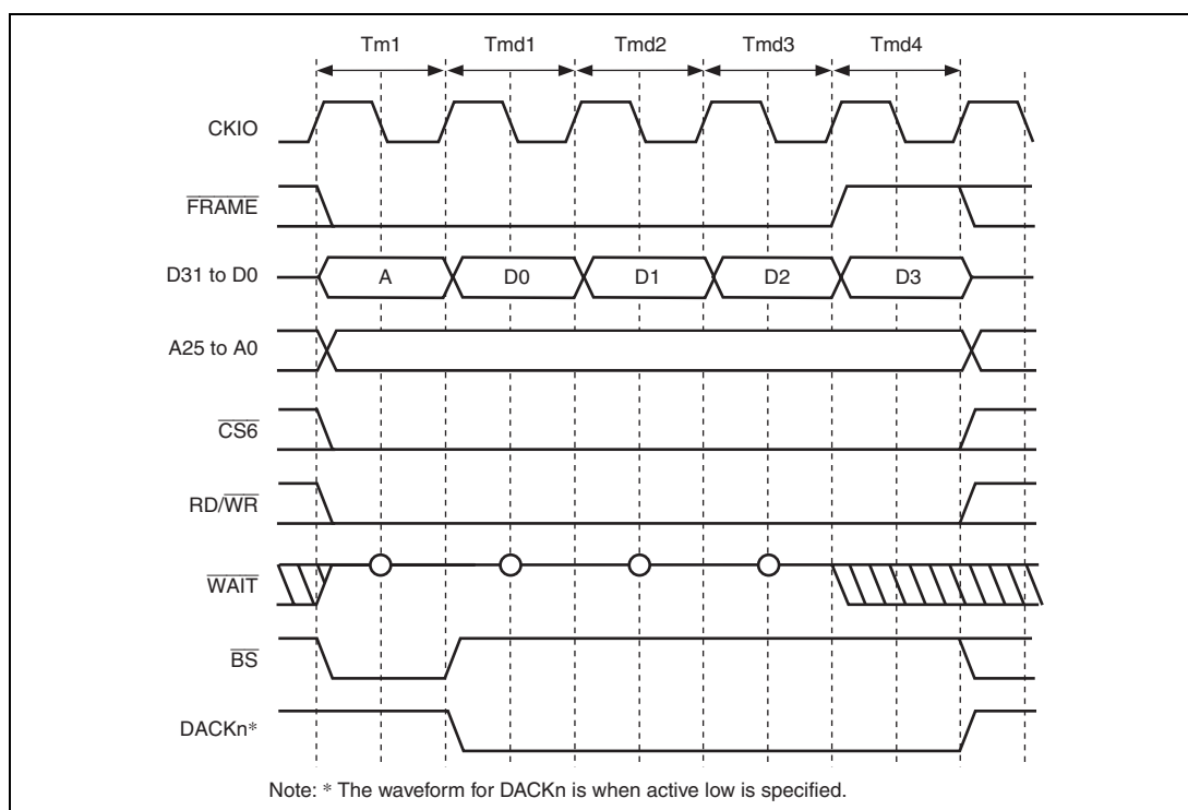
Figure 9.51 Burst MPX Space Access Timing (Burst Write, No Wait, CS6WCR.MPXMD = 0)
