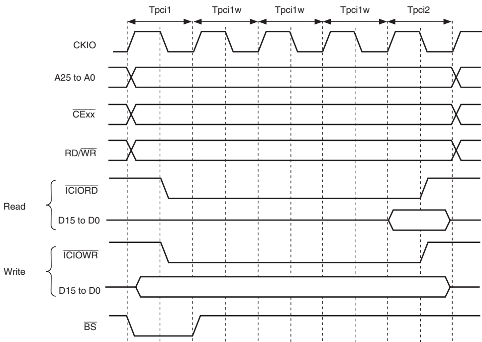
Figure 9.45 Basic Access Timing for PCMCIA I/O Card Interface
