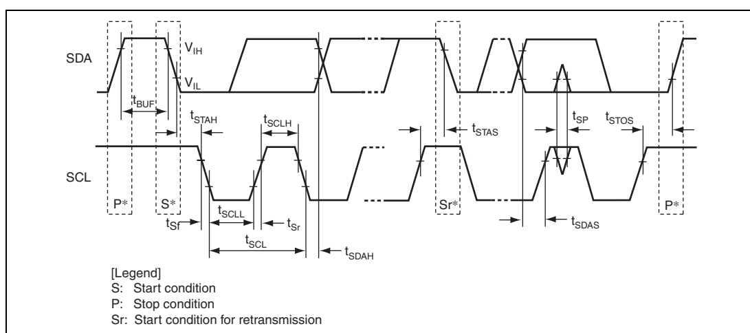
Figure 31.57 IIC3 Input/Output Timing
