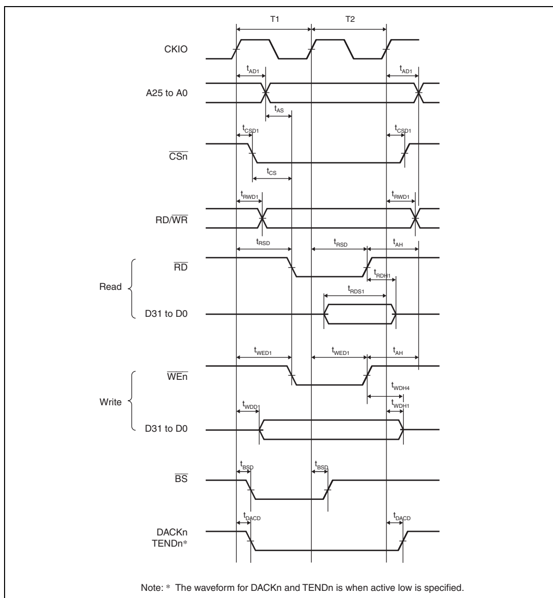
Figure 31.13 Basic Bus Timing for Normal Space (No Wait)
