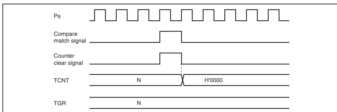
Figure 11.84 Counter Clear Timing (Compare Match)
