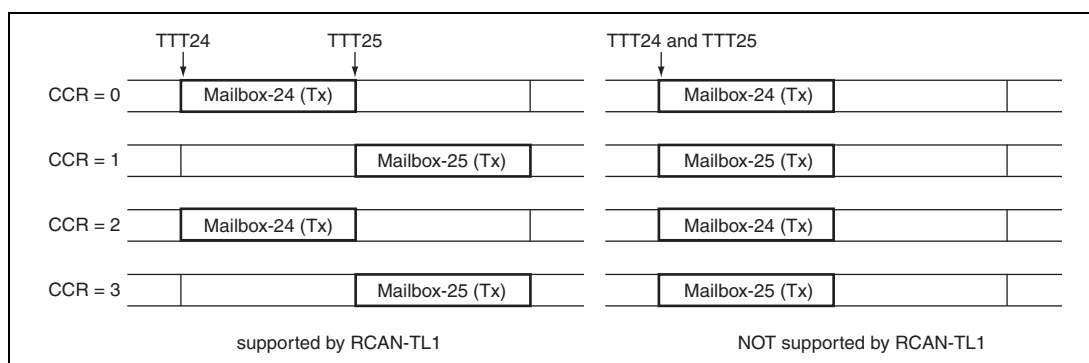
Figure 19.18 Limitation on Tx-Trigger Time
