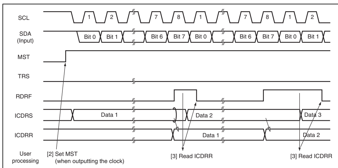
Figure 17.15 Receive Mode Operation Timing
