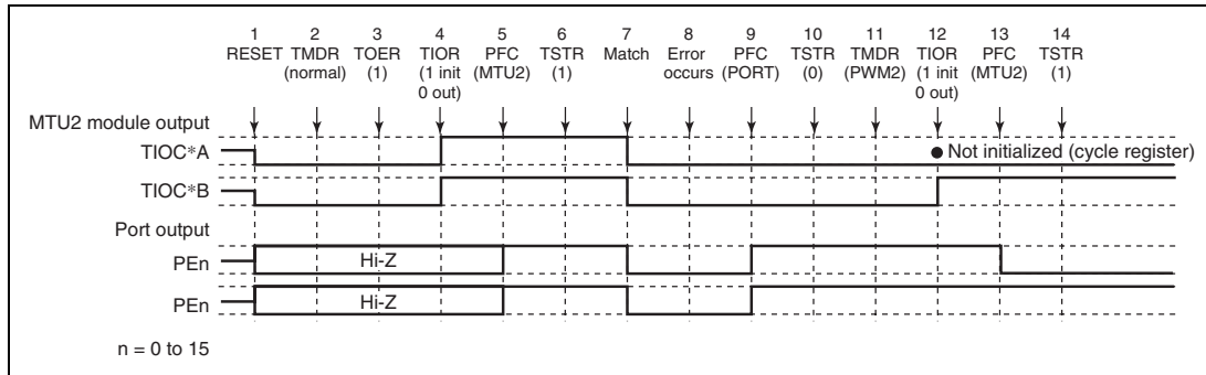
Figure 11.115 Error Occurrence in Normal Mode, Recovery in PWM Mode 2
