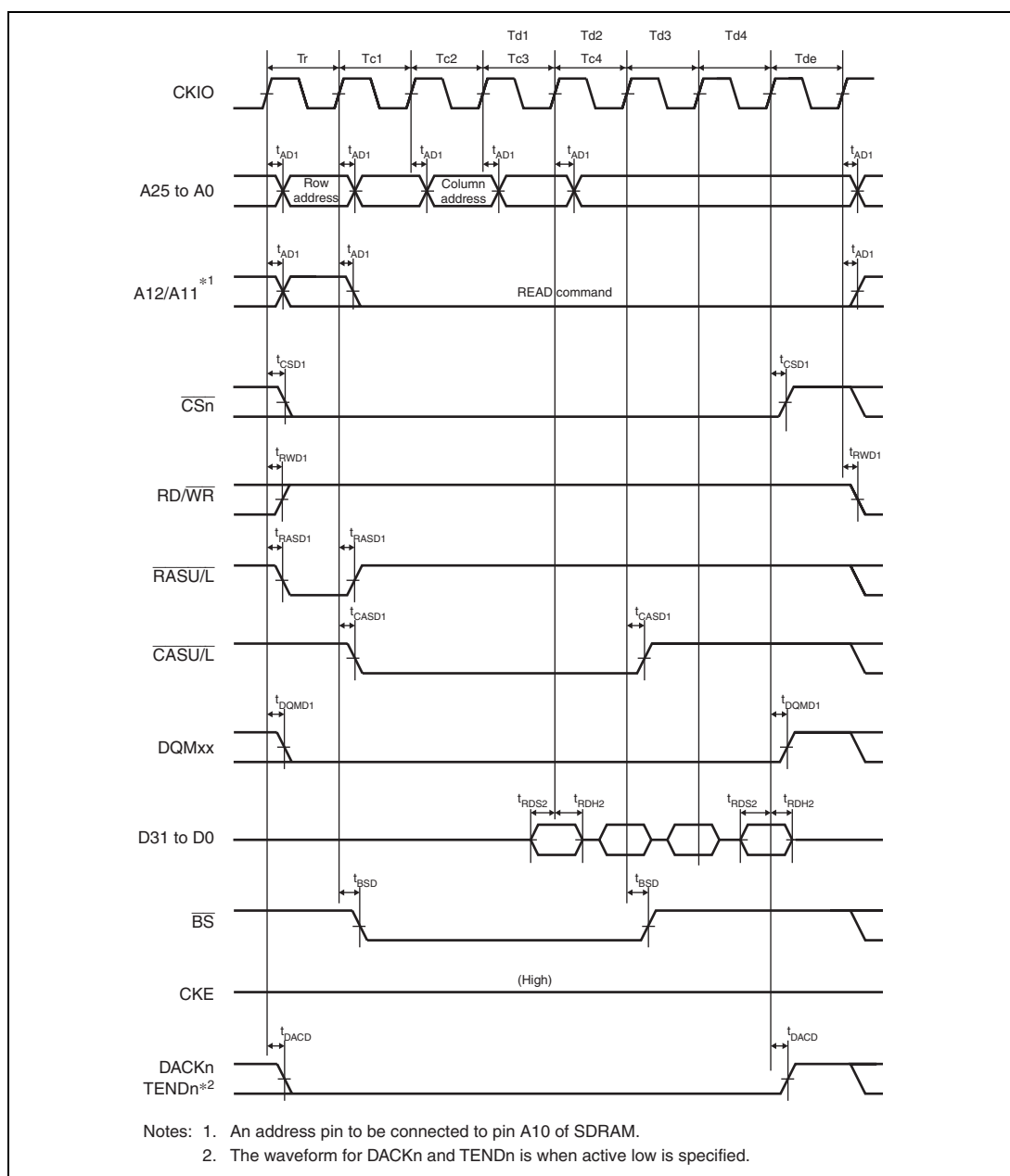
Figure 31.30 Synchronous DRAM Burst Read Bus Cycle (Four Read Cycles) (Bank Active Mode: ACT + READ Commands, CAS Latency 2, WTRCD = 0 Cycle)
