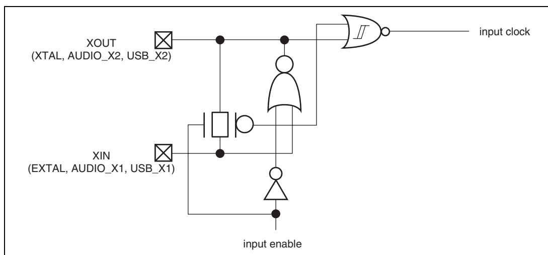
Figure 1.3 (13) Simplified Circuit Diagram (Oscillation Buffer 1)
