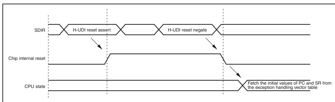
Figure 29.4 H-UDI Reset
