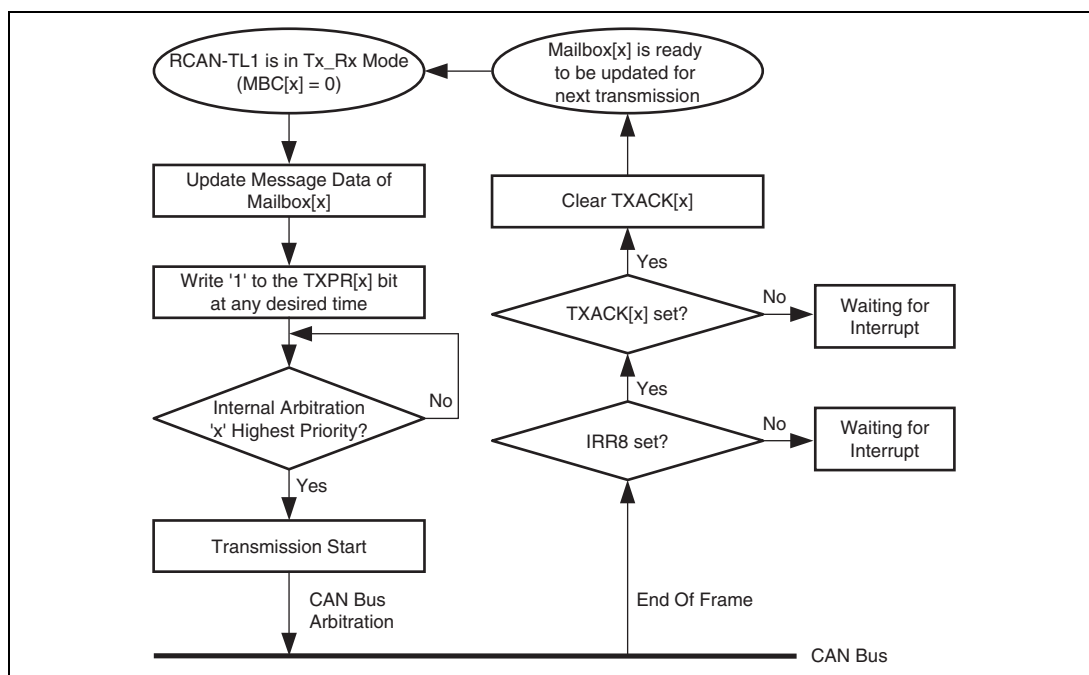
Figure 19.16 Transmission request
