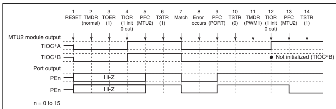
Figure 11.114 Error Occurrence in Normal Mode, Recovery in PWM Mode 1
