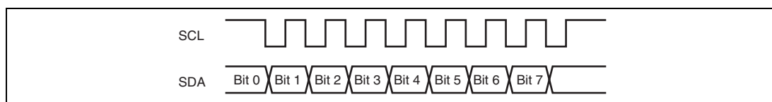
Figure 17.13 Clocked Synchronous Serial Transfer Format
