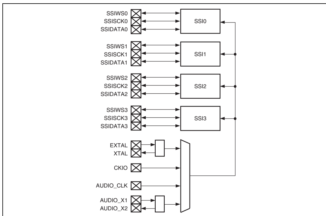
Figure 18.1 Schematic Diagram of SSI Module
