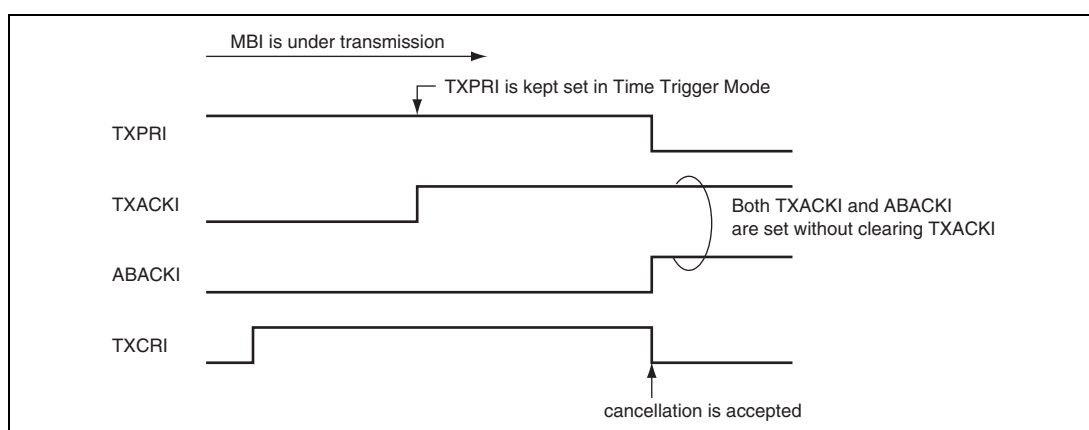
Figure 19.7 TXACK and ABACK in Time Trigger Transmission
