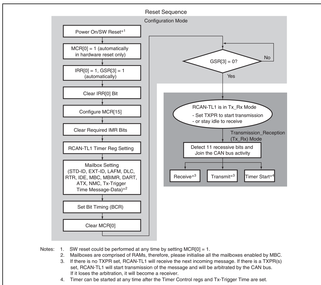
Figure 19.14 Reset Sequence
