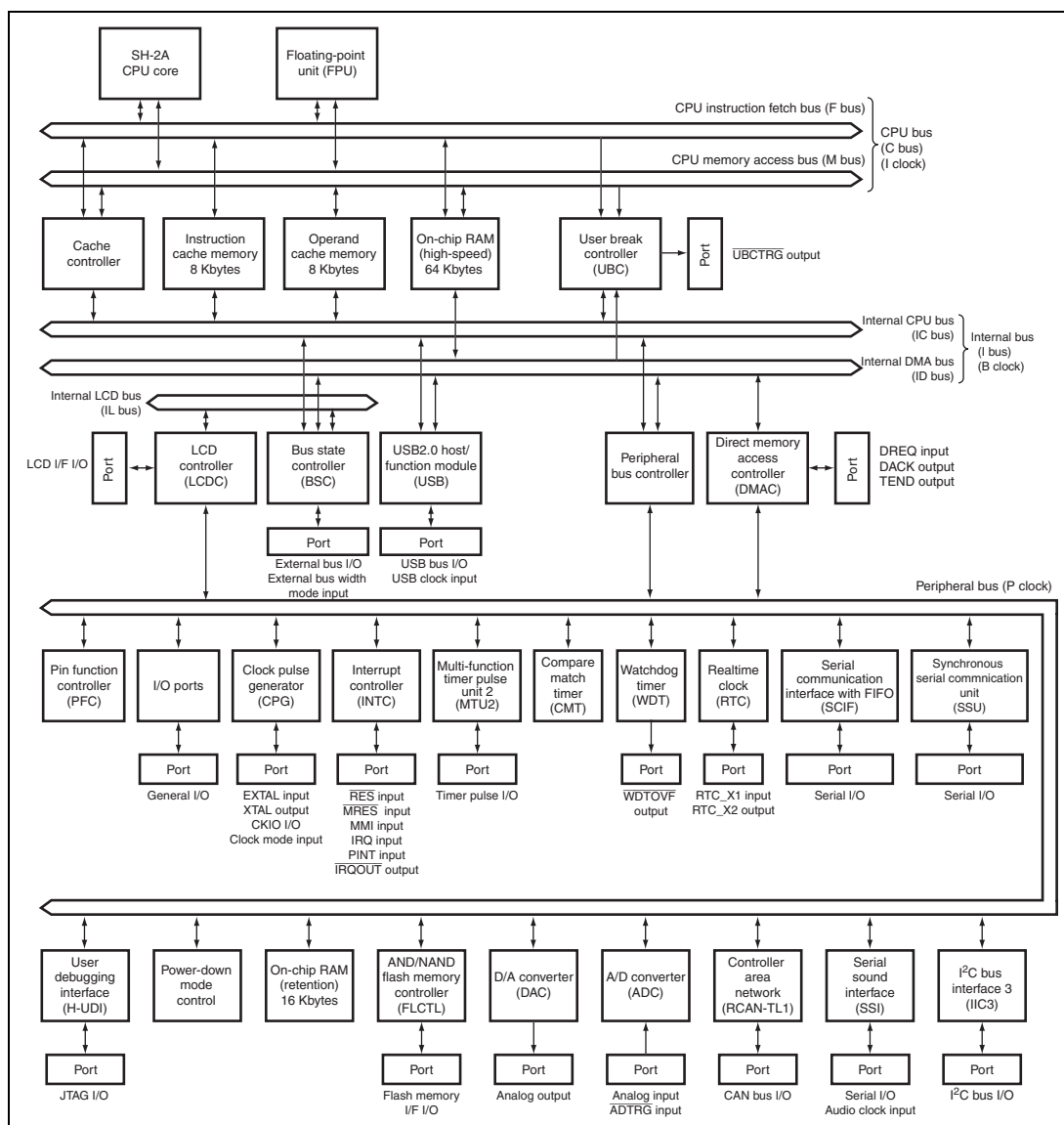
Figure 1.1 Block Diagram
