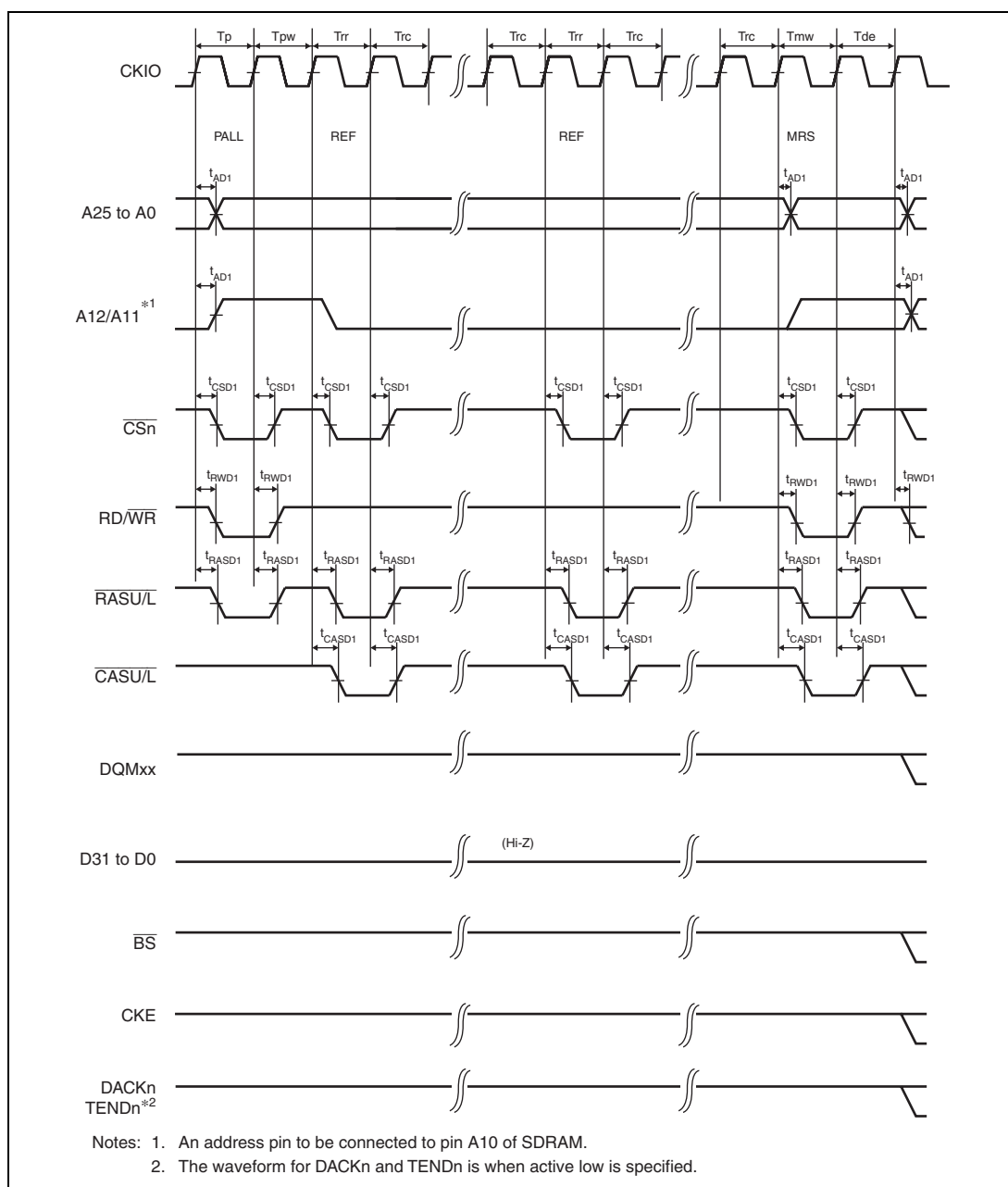
Figure 31.38 Synchronous DRAM Mode Register Write Timing (WTRP = 1 Cycle)
