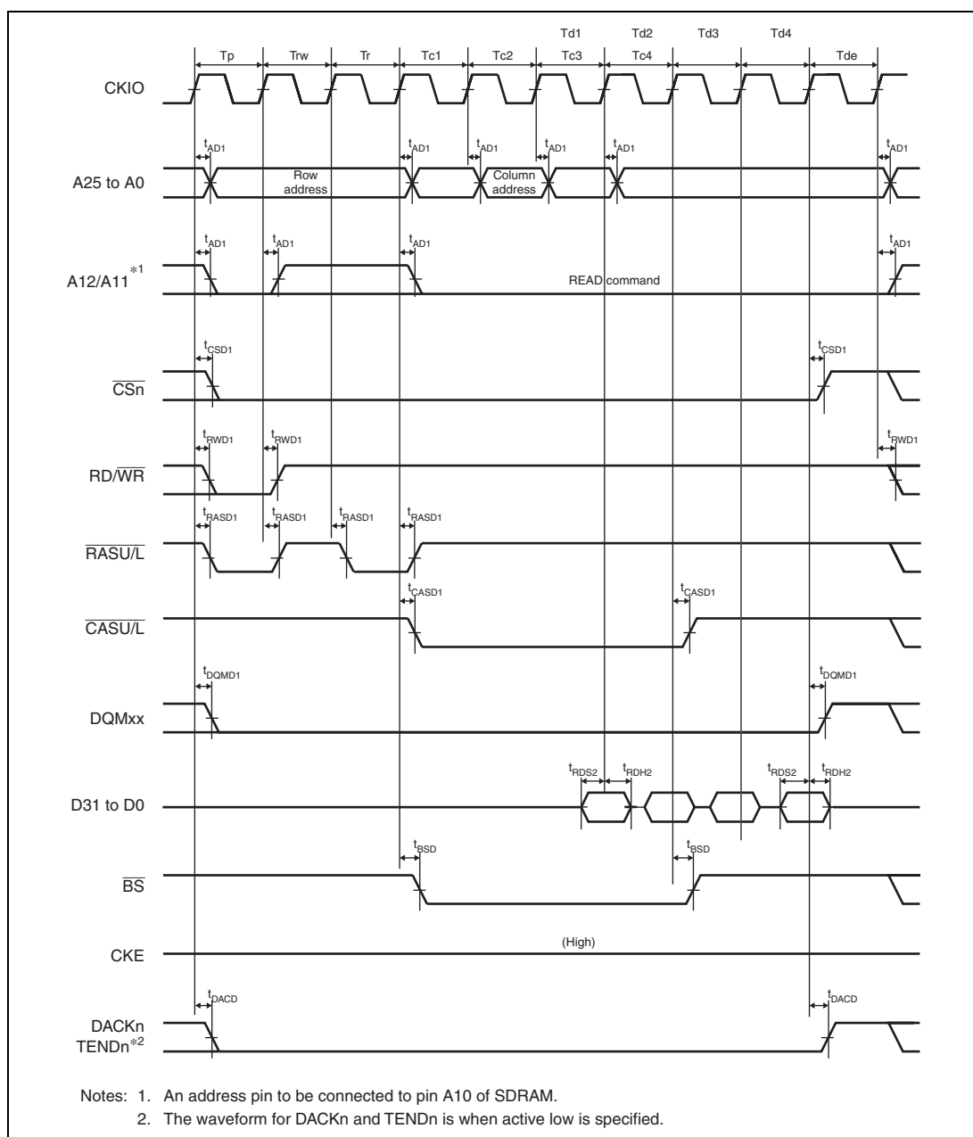
Figure 31.32 Synchronous DRAM Burst Read Bus Cycle (Four Read Cycles) (Bank Active Mode: PRE + ACT + READ Commands, Different Row Addresses, CAS Latency 2, WTRCD = 0 Cycle)
