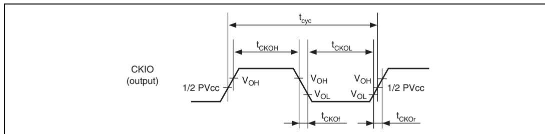
Figure 31.4 CKIO Clock Output Timing
