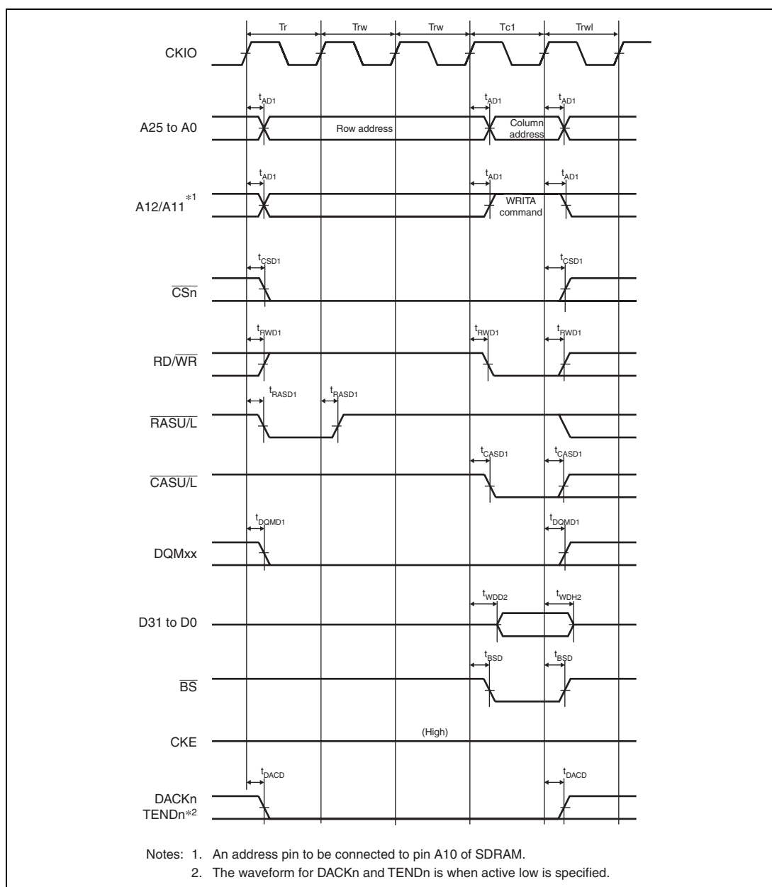
Figure 31.27 Synchronous DRAM Single Write Bus Cycle (Auto Precharge, WTRCD = 2 Cycles, TRWL = 1 Cycle)
