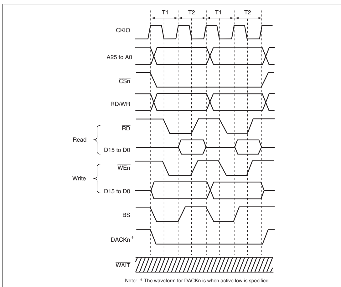
Figure 9.4 Continuous Access for Normal Space 2 Bus Width = 16 Bits, Longword Access, CSnWCR.WM Bit = 1 (Access Wait = 0, Cycle Wait = 0)
