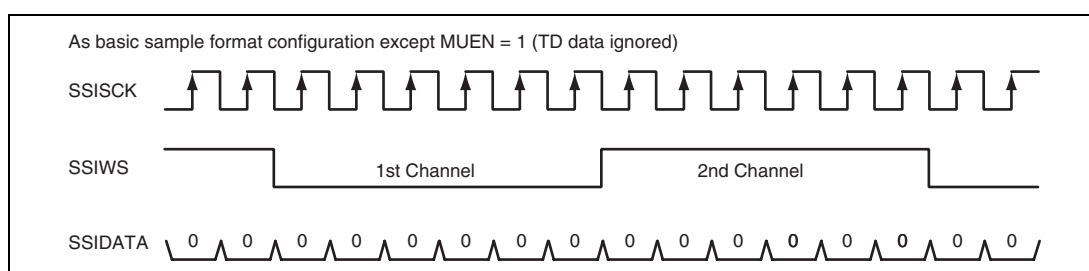
Figure 18.18 Mute Enabled
