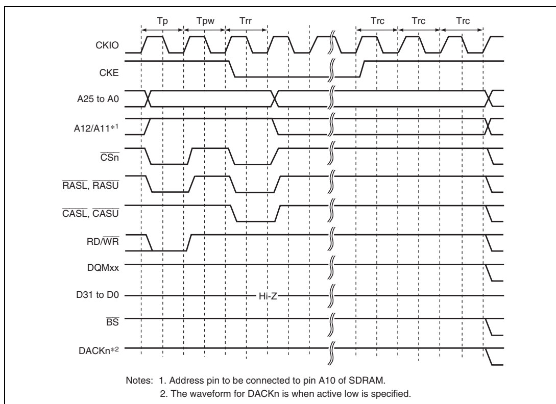
Figure 9.29 Self-Refresh Timing
