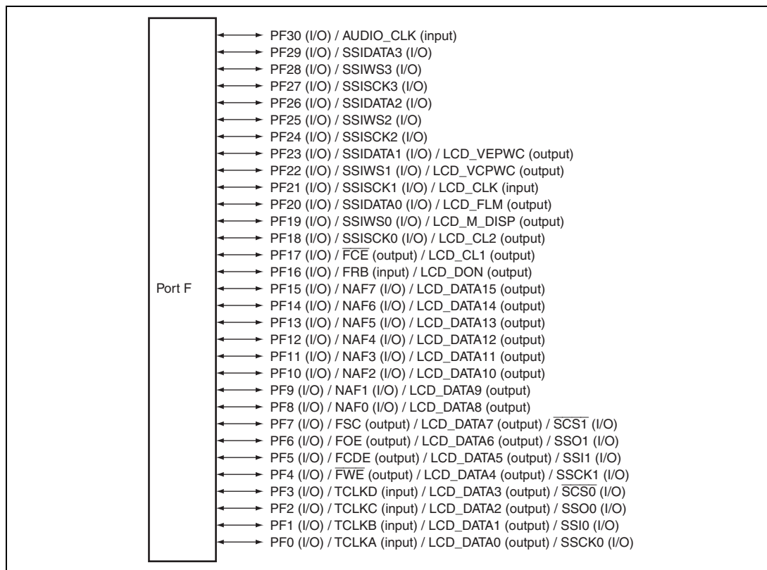
Figure 26.6 Port F
