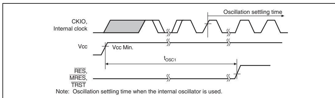
Figure 31.5 Power-On Oscillation Settling Time
