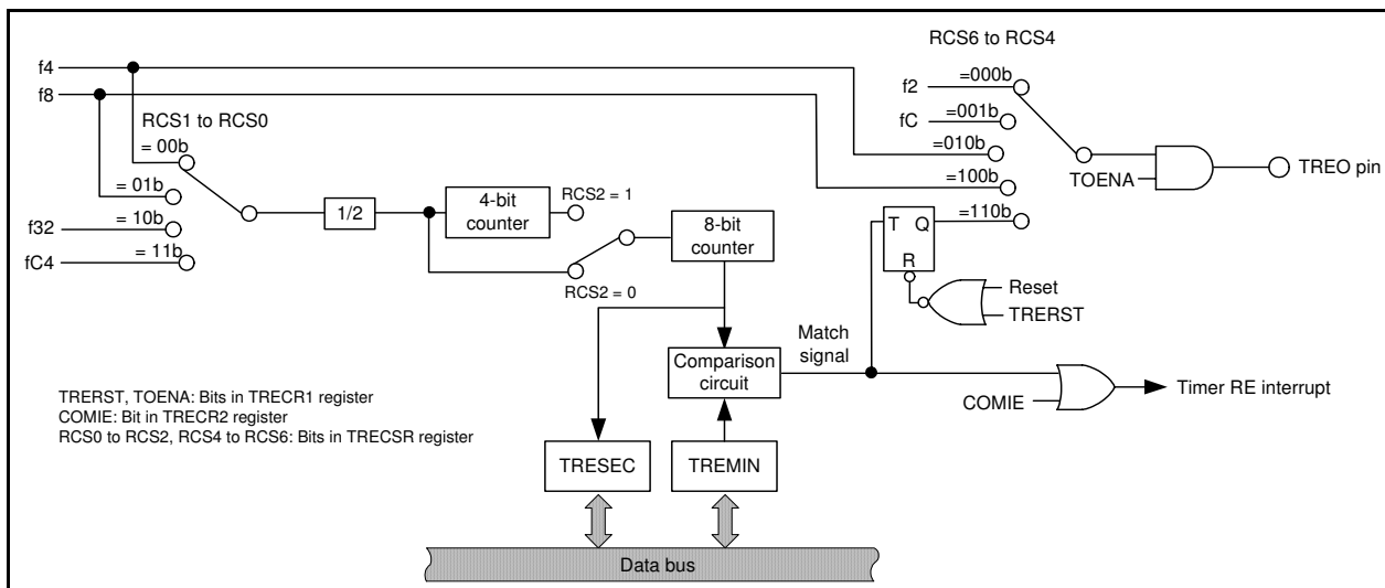
Figure 21.4 Block Diagram of Output Compare Mode
