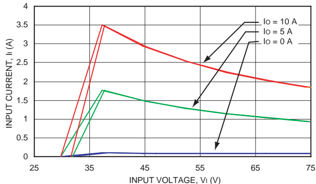
Figure 43. Input Voltage and Current Characteristics.
