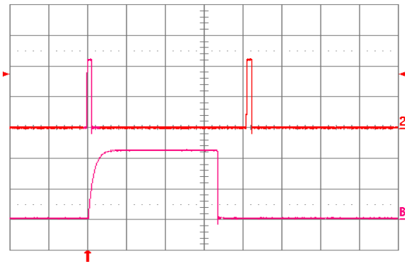
Figure 3.3V.24. Load current (top trace, 20 A/div., 50 ns/div.) into a 10 \text{ m}\Omega short circuit during restart, at V_{in} = 48 \text{ V} . Bottom trace (20 A/div., 2 ns/div.) is an expansion of the on-time portion of the top trace.
