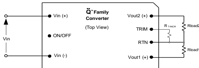
Figure 2. Configuration for increasing output voltage.
