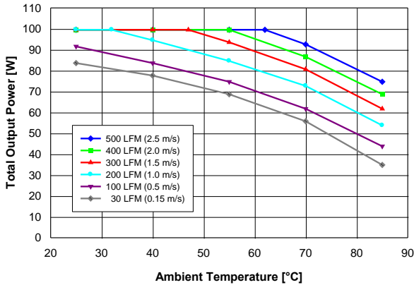
Figure 7. Available output power for balanced load current ( l_{out1} = 1.5 \cdot l_{out2} ) vs. ambient air temperature and airflow rates for converter mounted vertically with V_{in} = 48 V, air flowing from pin 3 to pin 1 and maximum FET temperature \leq 120 °C.
