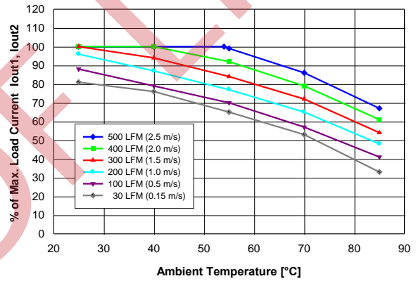
Figure 14. Available balanced load current ( I_{out1} = 1.5 \cdot I_{out2} ) vs. ambient air temperature and airflow rates for converter mounted vertical-ly with V_{in} = 48\text{ V} , air flowing from pin 4 to pin 3 and maximum FET temperature \leq 120\text{ }^\circ\text{C} .
