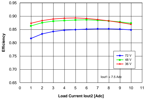
Figure 17. Efficiency vs. load current Iout2 and input voltage for converter mounted vertically with air flowing from pin 3 to pin 1 at a rate of 300 LFM (1.5 m/s), for Iout1 = 7.5 A and Ta = 25 °C.
