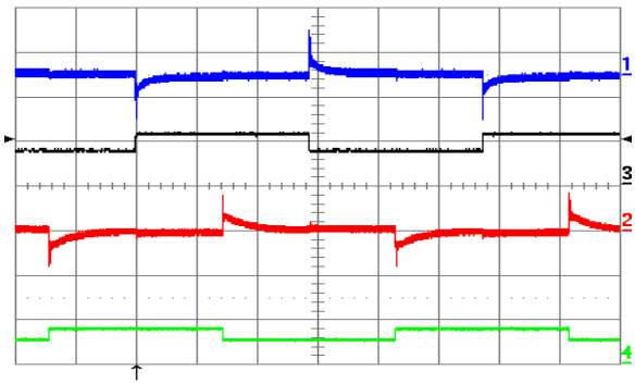
Figure 28. Output voltage response to both Iout1 and Iout2 (out of phase) load current step-change of 3.75 A (Iout1) and 2.5 A (Iout2) (50%-75%-50%) at Vin = 48 V. Ch1 = Vout1 (100 mV/div), Ch2 = Vout2 (100 mV/div), Ch3 = Iout1 (10 A/div.), Ch4 = Iout2 (10 A/div.). Current slew rate: 5 A/ \mu s, Co = 300 \mu F tantalum + 1 \mu F ceramic. Time scale: 1 ms/div.
