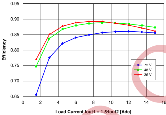
Figure 19. Efficiency vs. balanced load current (Iout1 = 1.5*Iout2) and input voltage for converter mounted vertically with air flowing from pin 3 to pin 1 at a rate of 300 LFM (1.5 m/s) and Ta = 25 °C.
