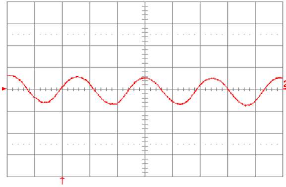
Figure 35. Input reflected ripple current, I_c (100 mA/div), measured at input terminals at full rated load current on both outputs and V_{in} = 48 V. Refer to Fig. 34 for test setup. Time scale: 1 \mu s/div.
