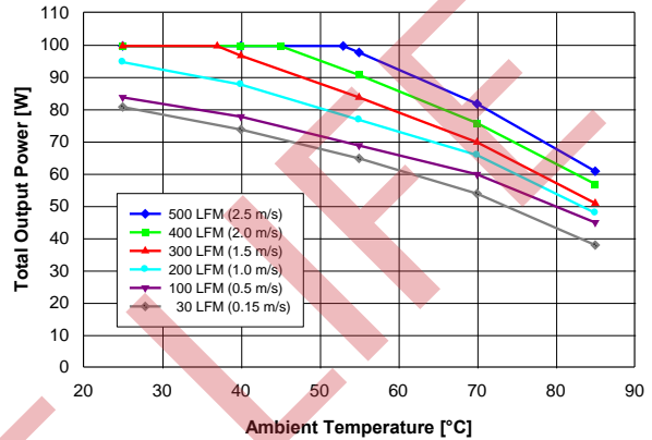
Figure 8. Available output power for balanced load current ( l_{out1} = 1.5 \cdot l_{out2} ) vs. ambient air temperature and airflow rates for converter mounted horizontally with V_{in} = 48 V, air flowing from pin 3 to pin 4 and maximum FET temperature \leq 120 °C.
