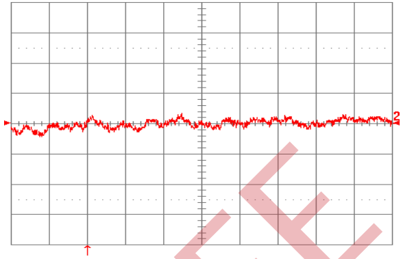
Figure 36. Input reflected ripple current, I_s (10 mA/div), measured through 10 \mu H at the source at full rated load current on both outputs and V_{in} = 48 V. Refer to Fig. 34 for test setup. Time scale: 1 \mu s/div.
