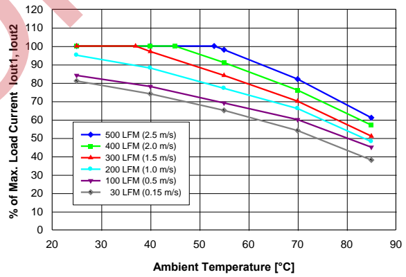
Figure 10. Available balanced load current ( l_{out1} = 1.5 \cdot l_{out2} ) vs. ambient temperature and airflow rates for converter mounted horizontally with V_{in} = 48 V, air flowing from pin 3 to pin 4 and maximum FET temperature \leq 120 °C.
