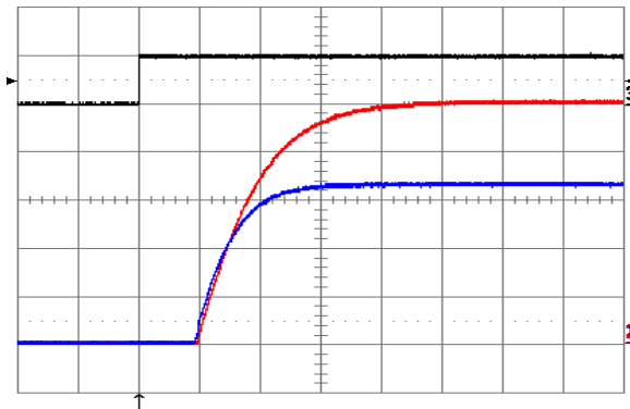
Figure 22. Turn-on transient waveforms at full rated load current (resistive) and Vin = 48 V, triggered via ON/OFF pin. Top trace: ON/OFF signal (5 V/div.). Bottom traces: Vout1 (blue, 1 V/div.), Vout2 (red, 1 V/div.). Time scale: 1 ms/div.
