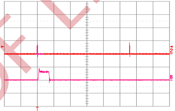
Figure 32. Load current Iout2 into a 10 mΩ short circuit on Vout2 during re-start, with Vout1 open (no load), at Vin = 48 V. Ch2 = Iout2 (20 A/div, 20 ms/div). ChB = Iout2 (20 A/div, 1 ms/div) is an expansion of the on-time portion of Iout2.
