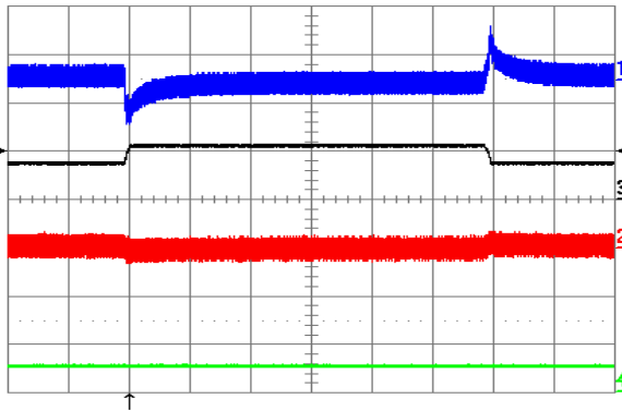
Figure 23. Output voltage response to Iout1 load current step-change of 3.75 A (50%-75%-50%) at Iout2 = 5 A and Vin = 48 V. Ch1 = Vout1 (50 mV/div), Ch2 = Vout2 (50 mV/div), Ch3 = Iout1 (10 A/div.), Ch4 = Iout2 (10 A/div.). Current slew rate: 0.1 A/ \mu s, Co = 10 \mu F tantalum + 1 \mu F ceramic. Time scale: 0.5 ms/div.
