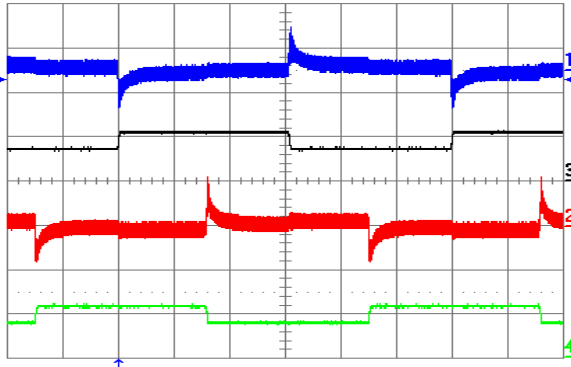
Figure 23. Output voltage response to both lout1 and lout2 (out of phase) load current step-change of 3.75 A (50%-75%-50%) at V_{in} = 48 V. Ch1 = Vout1 (50 mV/div), Ch2 = Vout2 (50 mV/div), Ch3 = lout1 (10 A/div.), Ch4 = lout2 (10 A/div.). Current slew rate: 0.1 A/ \mu s, C_o = 10 \mu F tantalum + 1 \mu F ceramic. Time scale: 1 ms/div.
