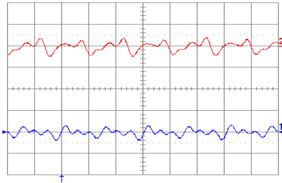
Figure 29. Output voltage ripple at full rated load current into a resistive load on both outputs with C_o = 1\mu\text{F} (ceramic) and V_{in} = 48\text{ V} . Ch2 = V_{out2} , Ch1 = V_{out1} (both 20 mV/div). Time scale: 1 \mu\text{s}/\text{div} .
