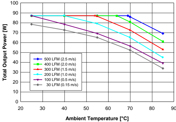
Figure 7. Available output power for balanced load current ( I_{out1} = I_{out2} ) vs. ambient air temperature and airflow rates for converter mounted vertically with V_{in} = 48 V , air flowing from pin 3 to pin 1 and maximum FET temperature \leq 120\text{ }^{\circ}C .
