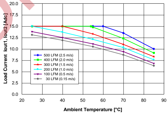
Figure 10. Available balanced load current ( I_{out1} = I_{out2} ) vs. ambient temperature and airflow rates for converter mounted horizontally with V_{in} = 48 V , air flowing from pin 3 to pin 4 and maximum FET temperature \leq 120\text{ }^{\circ}C .
