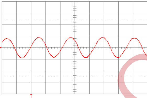
Figure 35. Input reflected ripple current, i_c (100 mA/div), measured at input terminals at full rated load current on both outputs and V_{in} = 48\text{ V} . Refer to Fig. 34 for test setup. Time scale: 1\text{ }\mu\text{s/div} .
