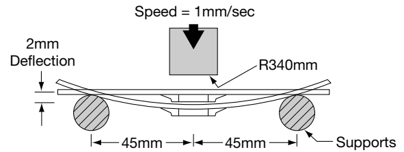
Figure 2. Bend Strength
