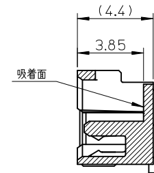
SECTION Y-Y
