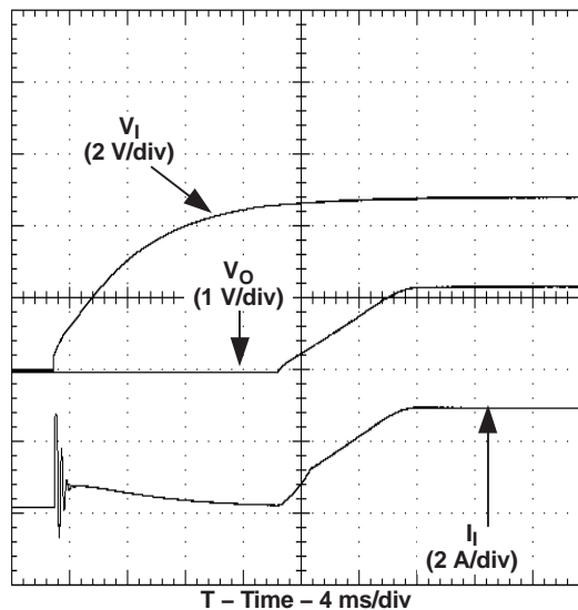
Figure 26. Power-Up Waveform
