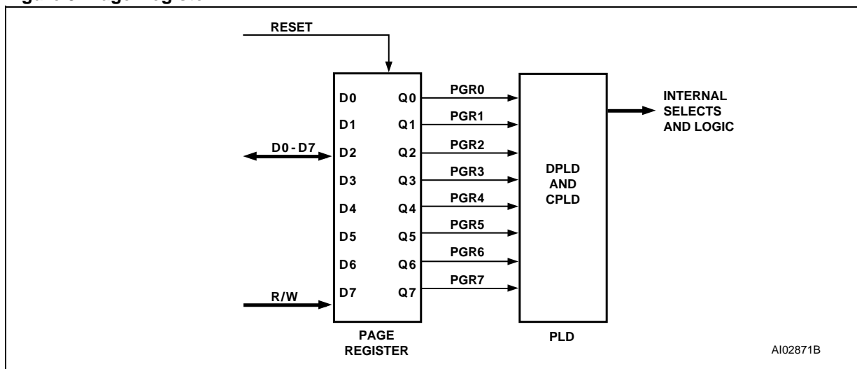
Figure 9. Page Register
