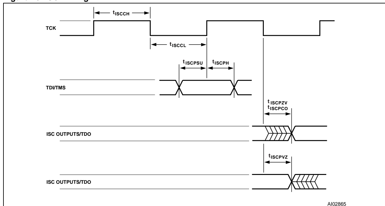
Figure 45. ISC Timing
