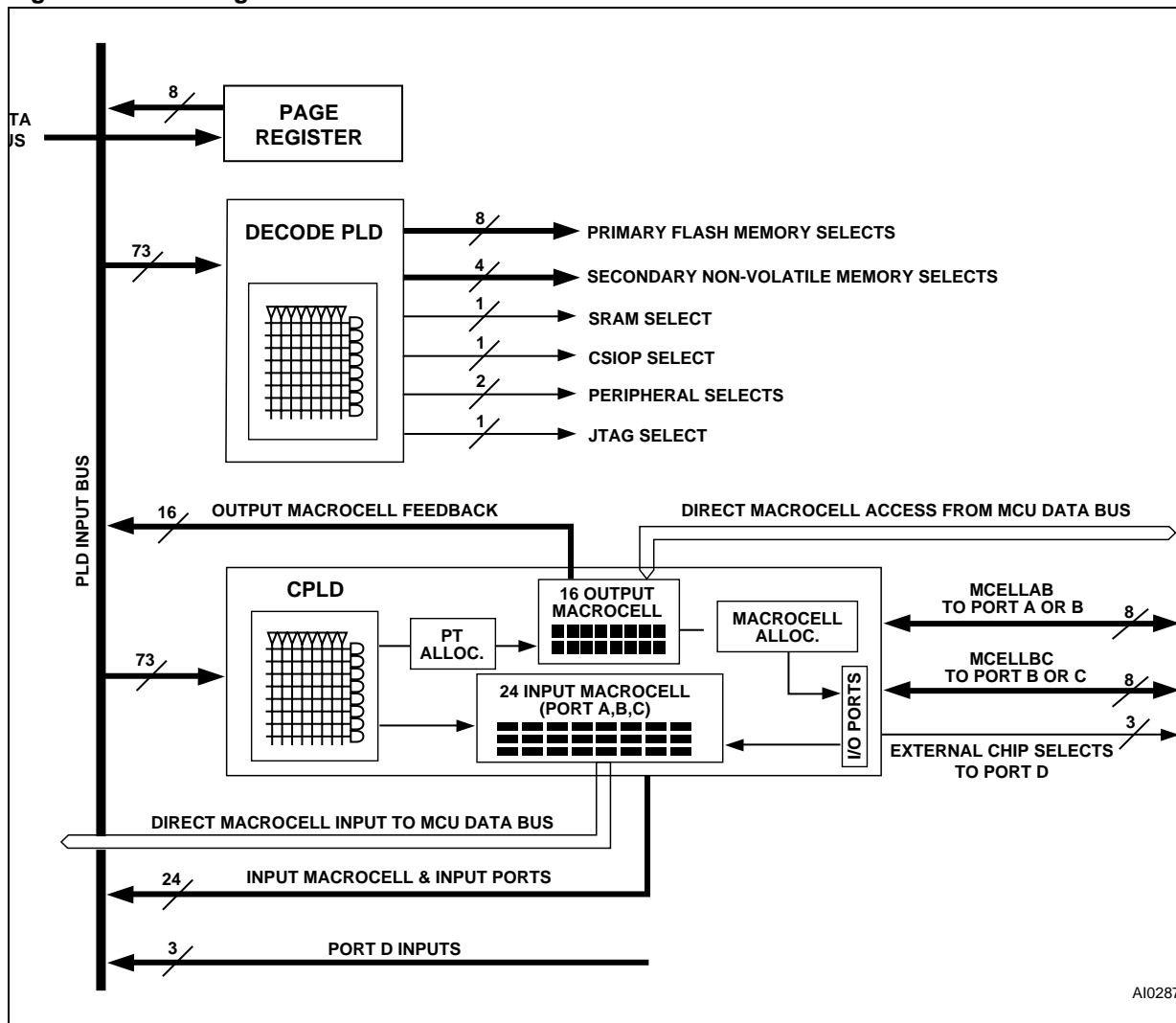
Figure 10. PLD Diagram
