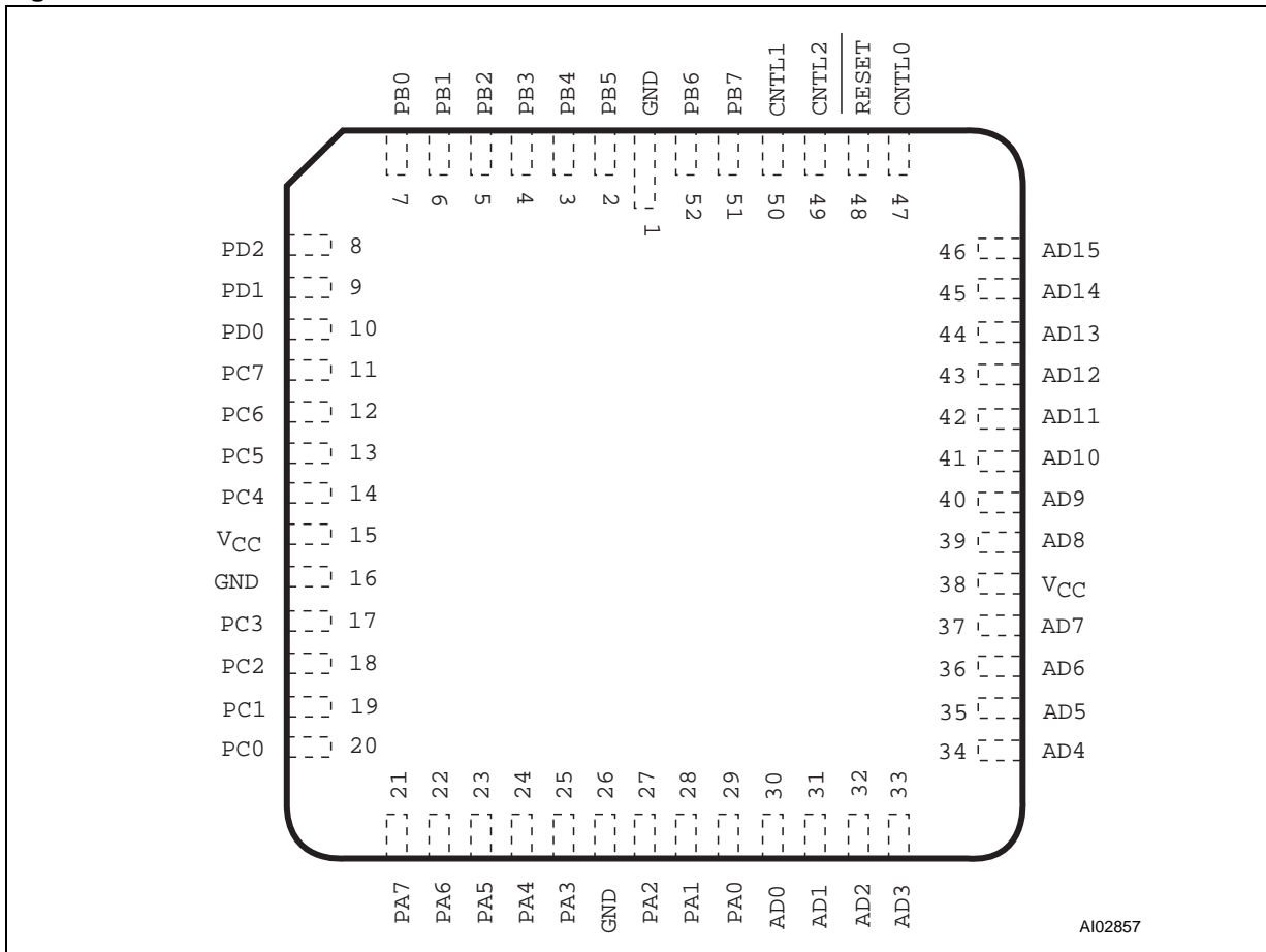
Figure 47. PLCC52 Connections
