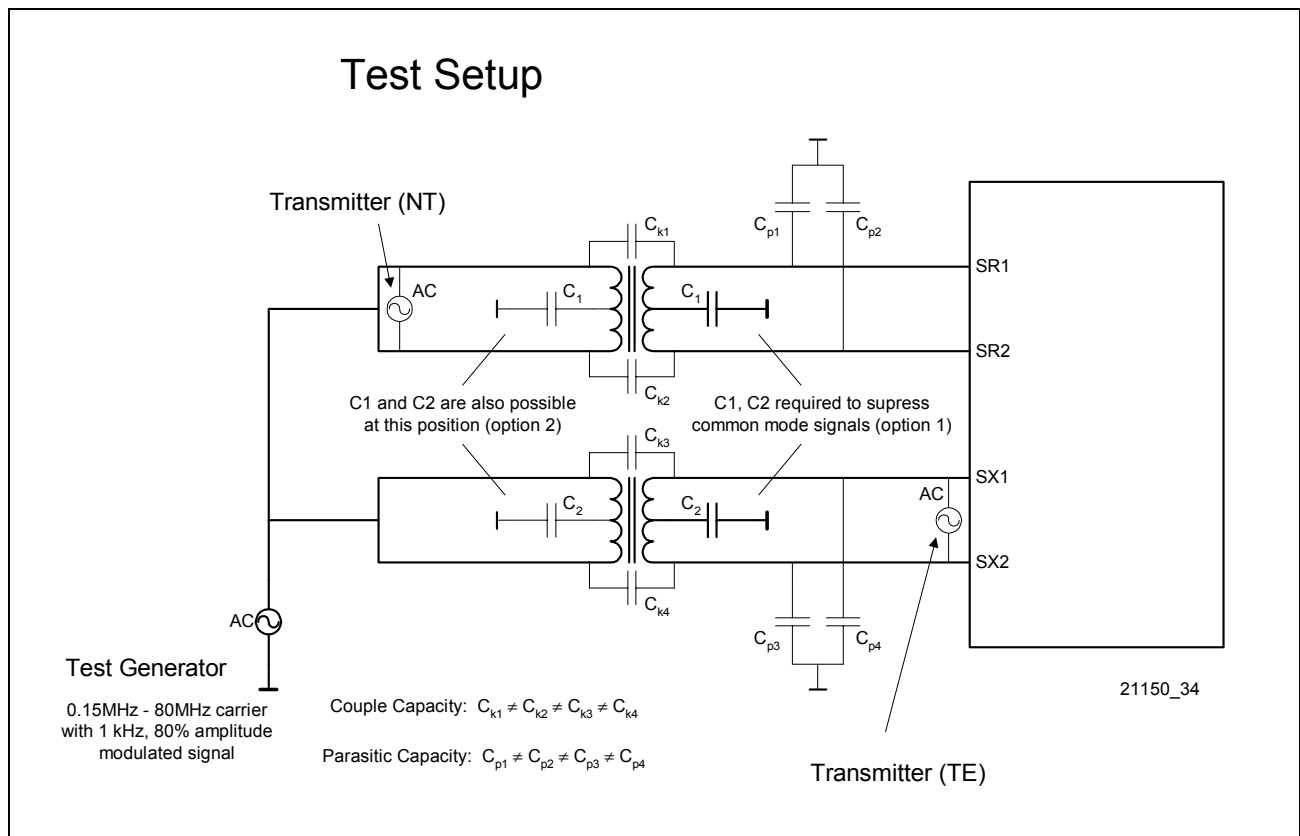
Figure 105 Transformer Circuitry
