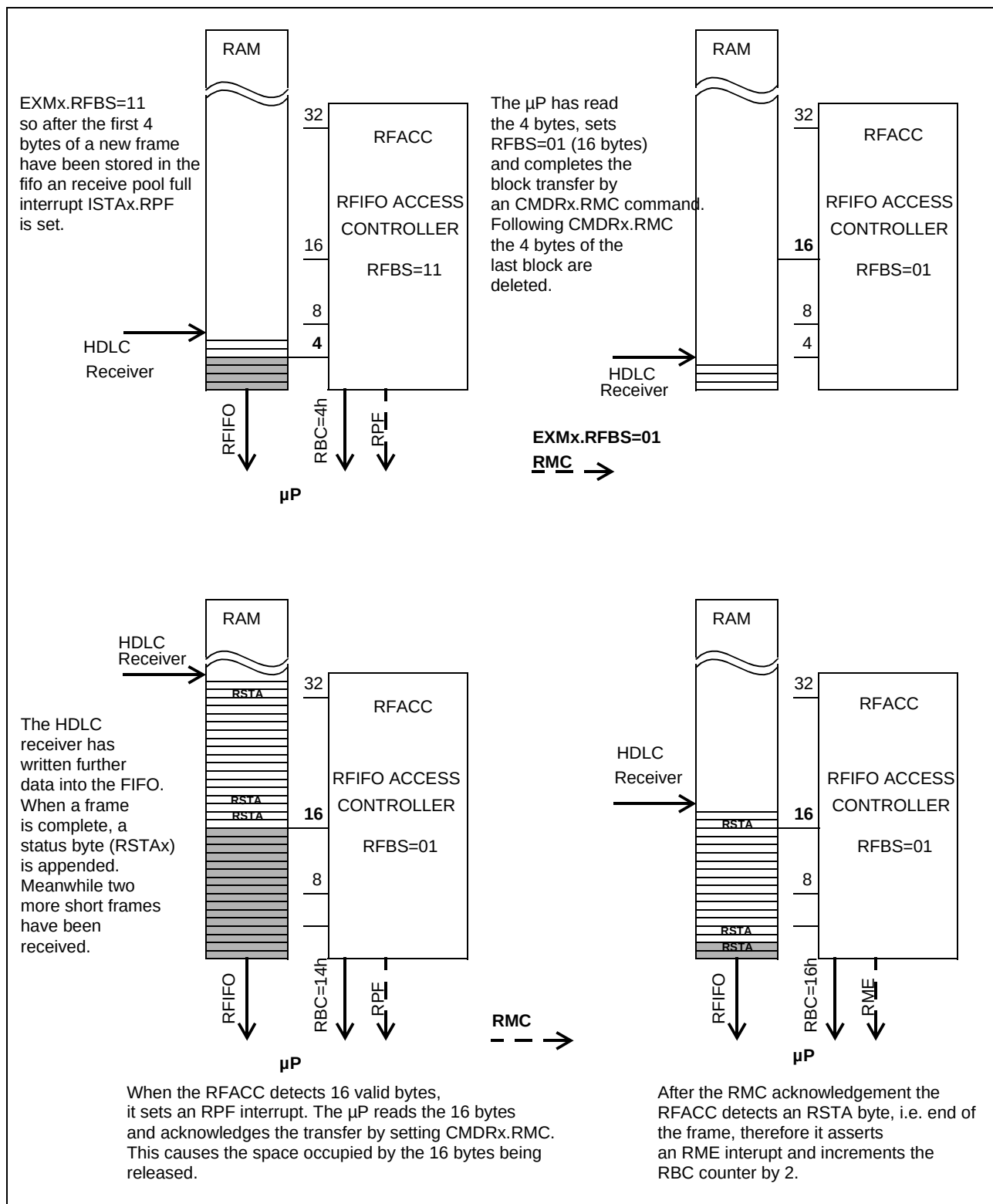
Figure 79 RFIFO Operation
