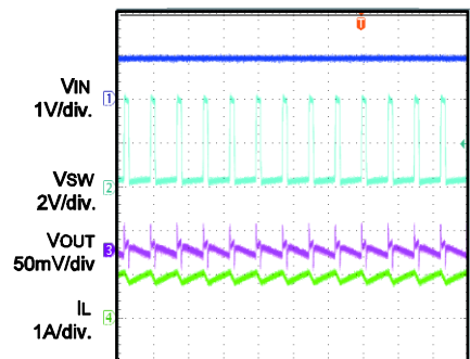
1μs/div
