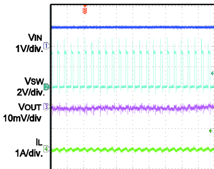
2μs/div
