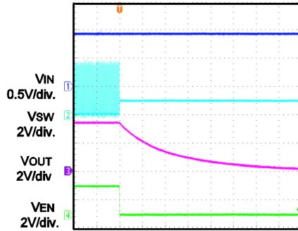
10ms/div
