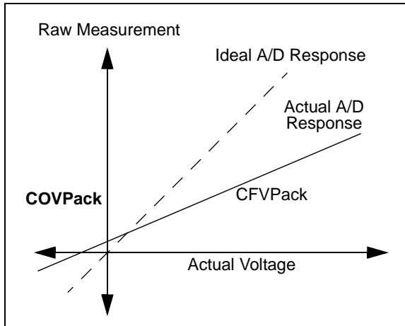
FIGURE 2-2: COVPack AND CFVPack VALUE RELATIONSHIP
