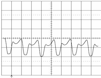
Output voltage ripple (20mV/div.) at: T_{ref} = +25^{\circ}\text{C} , I_O = 22\text{ A} resistive load, V_i = 5.0\text{ V} . Time scale: 2 \mu\text{s}/\text{div} .. See the filter in the Output ripple and noise section (EMC Specification).
