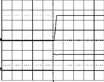
Start-up enabled by connecting V_I at: T_{ref} = +25^\circ\text{C} , V_I = 3.3\text{ V} , I_O = 6\text{ A} resistive load. Top trace: output voltage (1.0 V/div.). Bottom trace: input voltage (2 V/div.). Time scale: (20 ms/div.).
