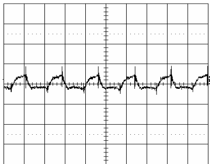
Output voltage ripple (20mV/div.) at: T_{ref} = +25^{\circ}\text{C} , I_O = 6\text{ A} resistive load, V_I = 3.3\text{ V} . Time scale: 1 \mu\text{s}/\text{div} . See the filter in the Output ripple and noise section (EMC Specification).
