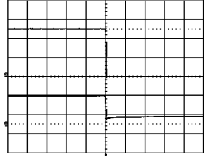
Shut-down enabled by disconnecting V_I at: T_{ref} = +25^\circ\text{C} , I_O = 6\text{ A} resistive load, V_I = 3.3\text{ V} . Top trace: output voltage (1.0 V/div.). Bottom trace: input voltage (2 V/div.). Time scale: 10.0 ms/div.
