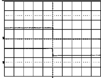
Shut-down enabled by disconnecting V_I at: T_{ref} = +25^{\circ}\text{C} , I_O = 6\text{ A} resistive load, V_I = 3.3\text{ V} . Top trace: output voltage (1.0 V/div.). Bottom trace: input voltage (2 V/div.). Time scale: 10.0 ms/div.
