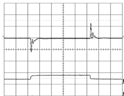
Output voltage response to load current step- change (3-6-3 A) at: T_{ref} = +25^{\circ}\text{C} , V_I = 3.3\text{ V} . Top trace: output voltage (100mV/div.). Bottom trace: load current (10 A/div.). Time scale: 0.1 ms/div.
