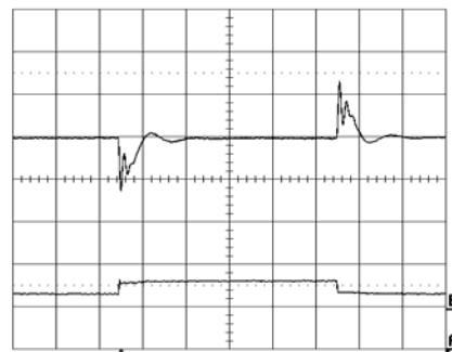
Output voltage response to load current step- change (3-6-3 A) at: T_{ref} = +25^\circ\text{C} , V_I = 3.3\text{ V} . Top trace: output voltage (100mV/div.). Bottom trace: load current (10 A/div.). Time scale: 0.1 ms/div.
