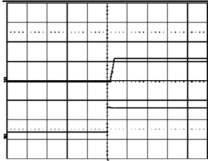
Start-up enabled by connecting V_I at: T_{ref} = +25^{\circ}\text{C} , V_I = 3.3\text{ V} , I_O = 6\text{ A} resistive load. Top trace: output voltage (1.0 V/div.). Bottom trace: input voltage (2 V/div.). Time scale: (20 ms/div.).
