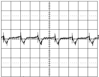
Output voltage ripple (20mV/div.) at: T_{ref} = +25^\circ\text{C} , I_O = 6\text{ A} resistive load, V_I = 3.3\text{ V} . Time scale: 1 \mu\text{s}/\text{div} . See the filter in the Output ripple and noise section (EMC Specification).
